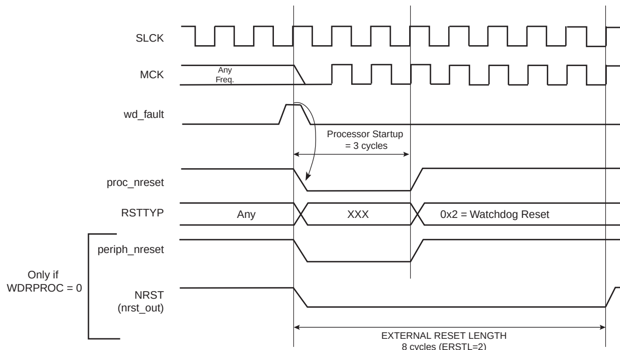
Figure 19-8. Watchdog Reset
