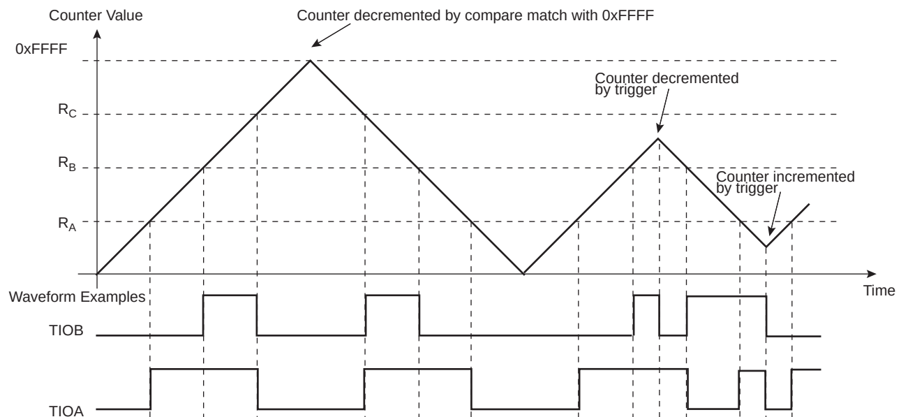
Figure 47-13.WAVSEL = 01 with Trigger
