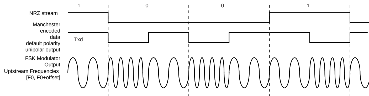
Figure 44-19.FSK Modulator Output
