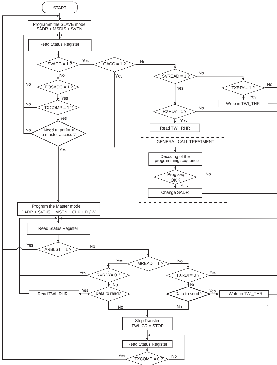
Figure 40-24. Multi-master Flowchart
