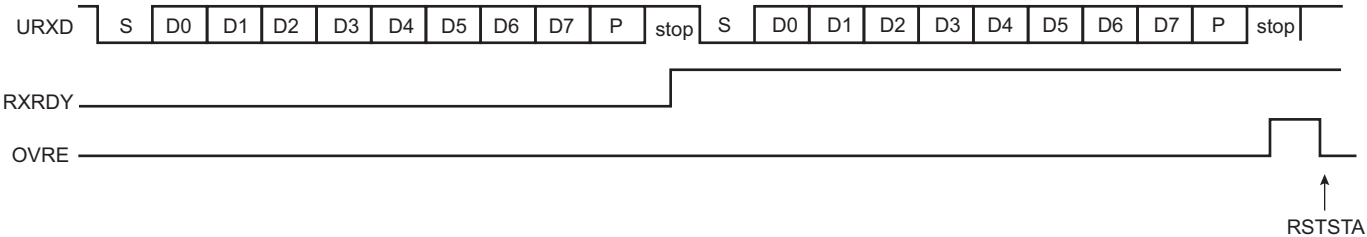
Figure 43-6. Receiver Overrun
