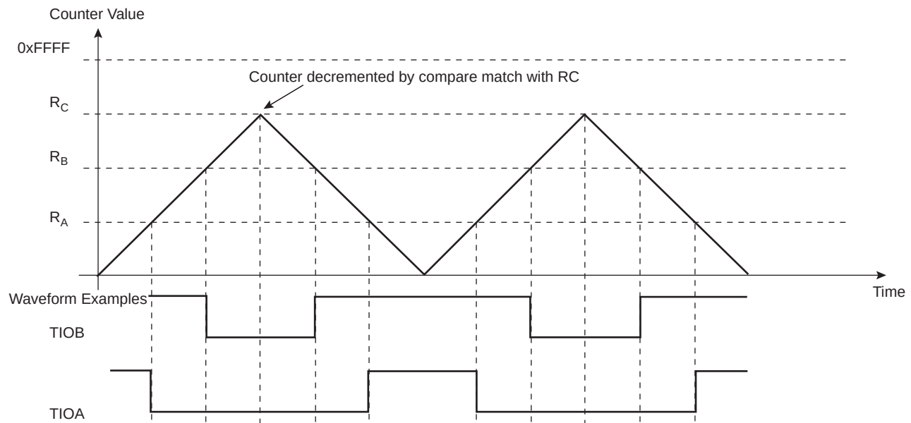
Figure 47-14.WAVSEL = 11 without Trigger
