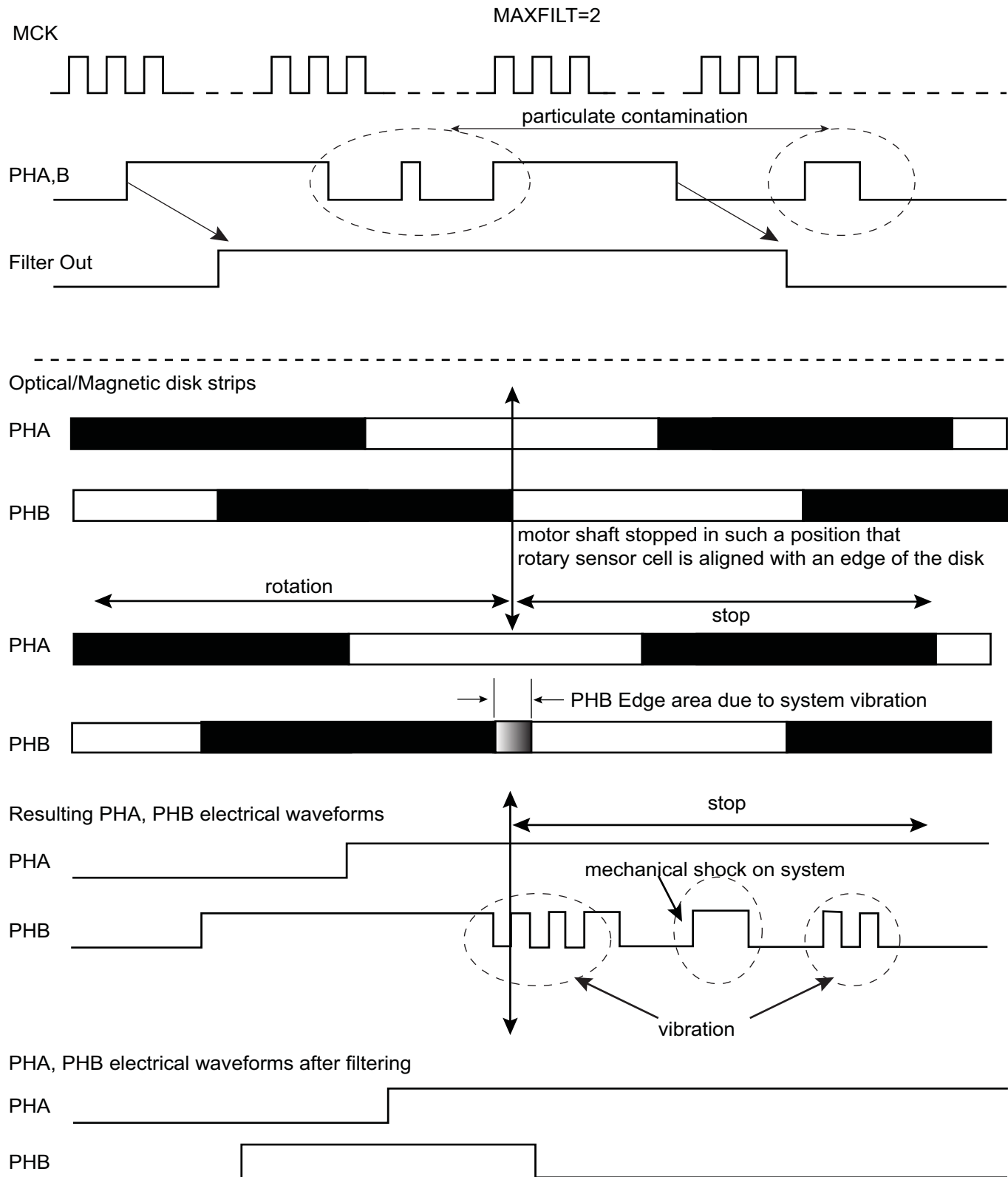
Figure 47-18. Filtering Examples
