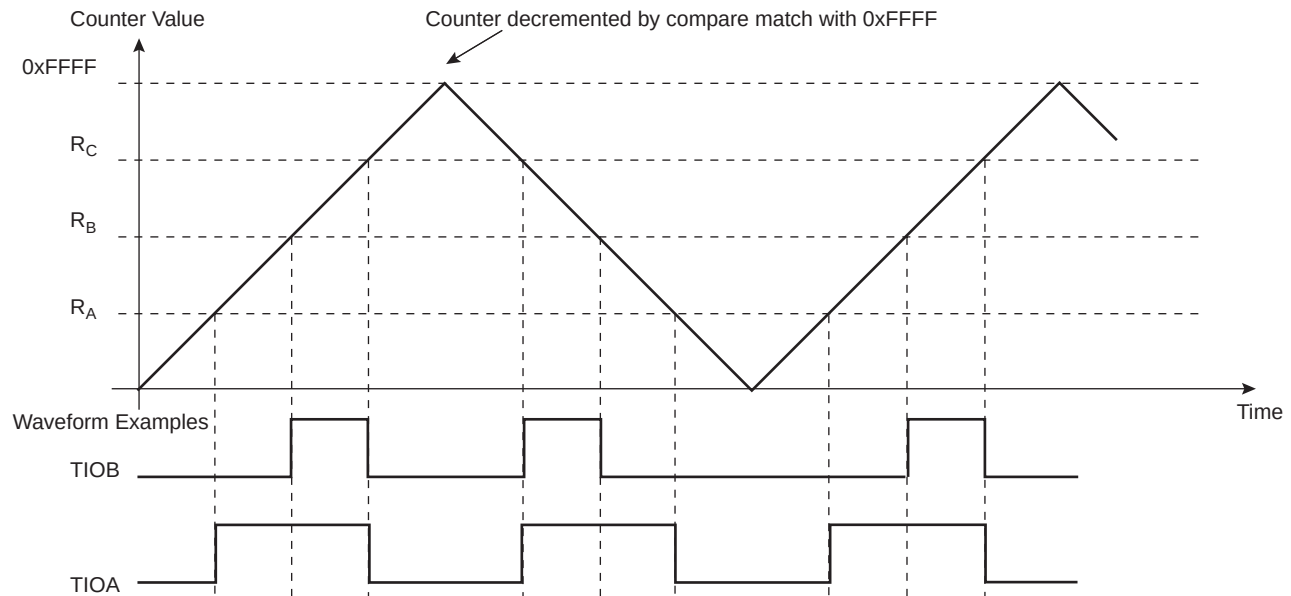
Figure 47-12.WAVSEL = 01 without Trigger
