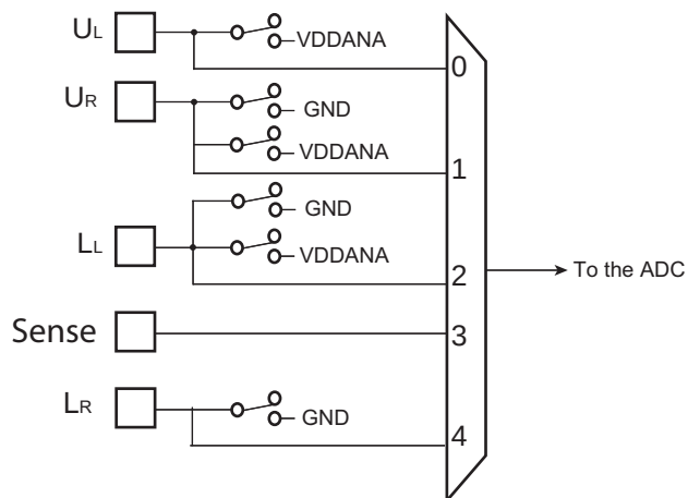
Figure 49-12.Touchscreen Switches Implementation
