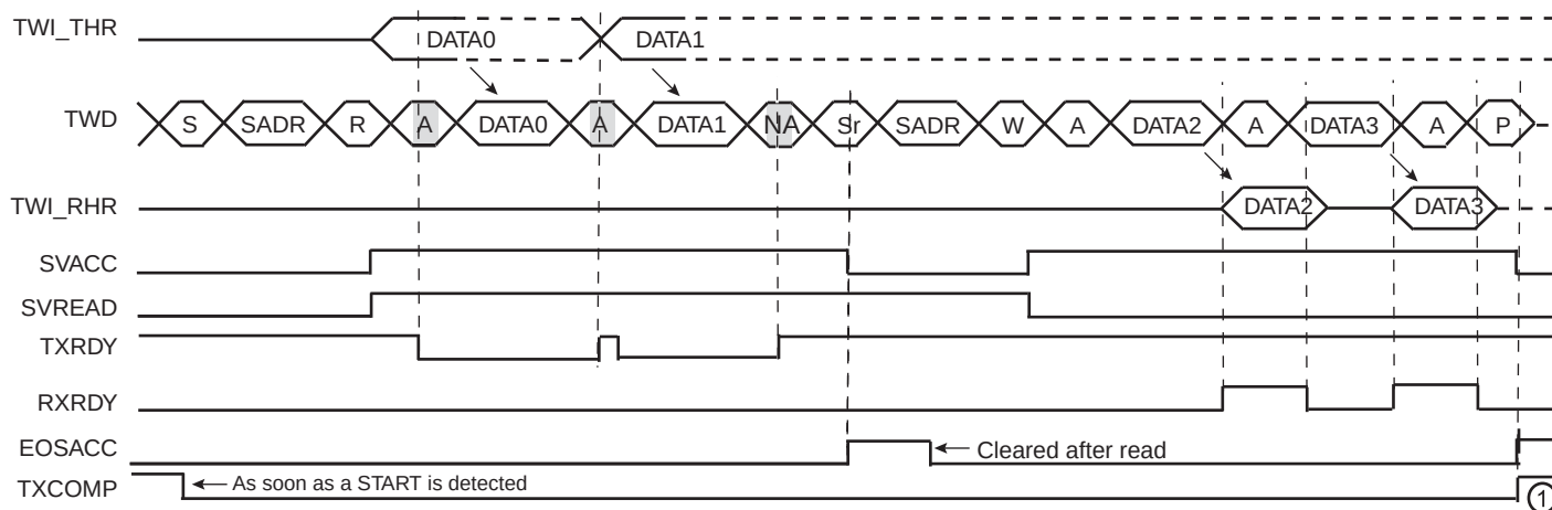
Figure 40-31.Repeated Start + Reversal from Read to Write Mode
