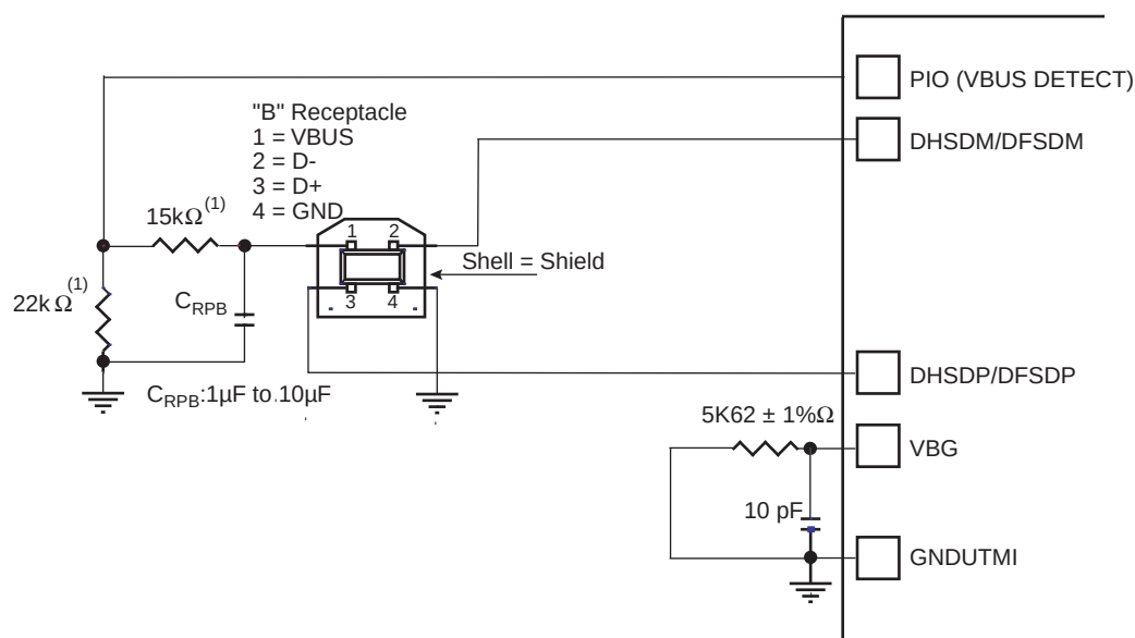
Figure 34-2. Board Schematic
