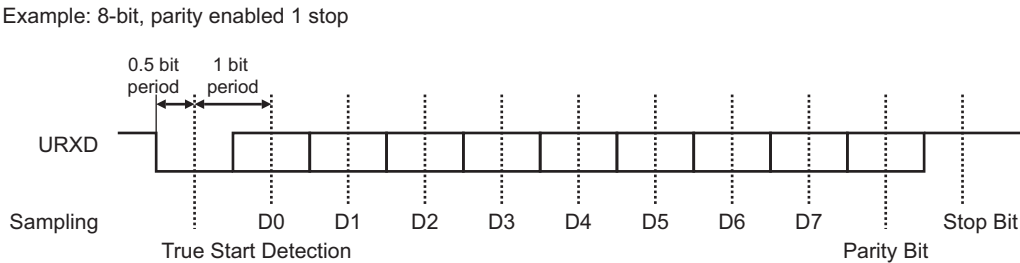
Figure 43-4. Character Reception
