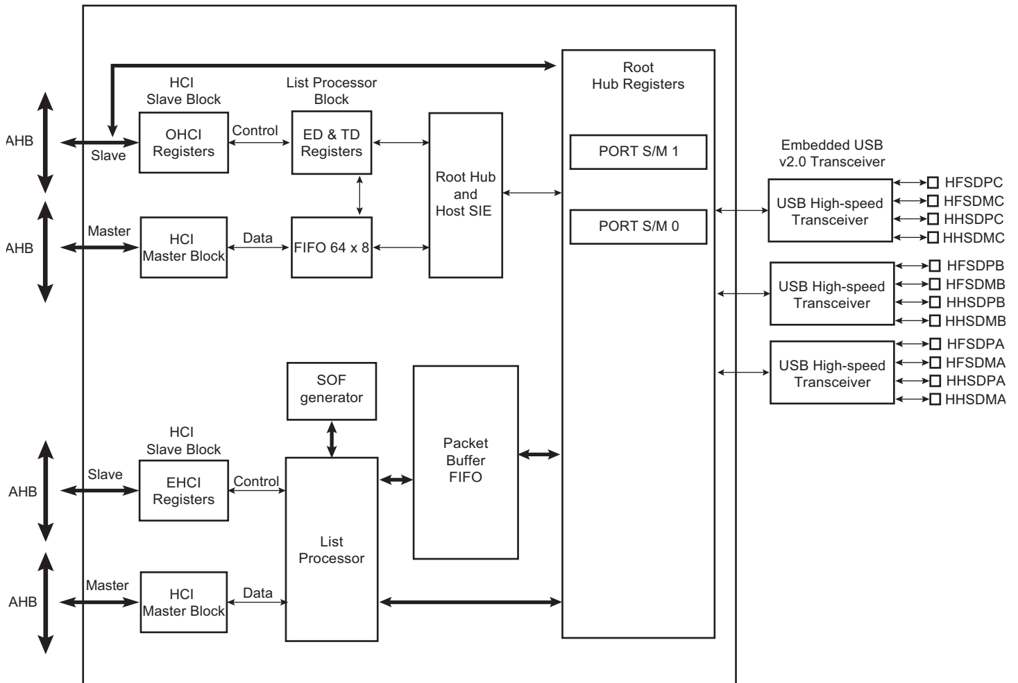
Figure 35-1. Block Diagram
