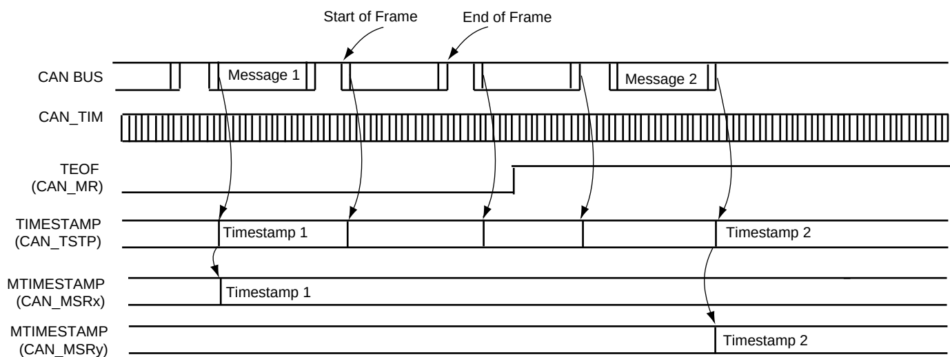
Figure 45-19. Mailbox Timestamp
