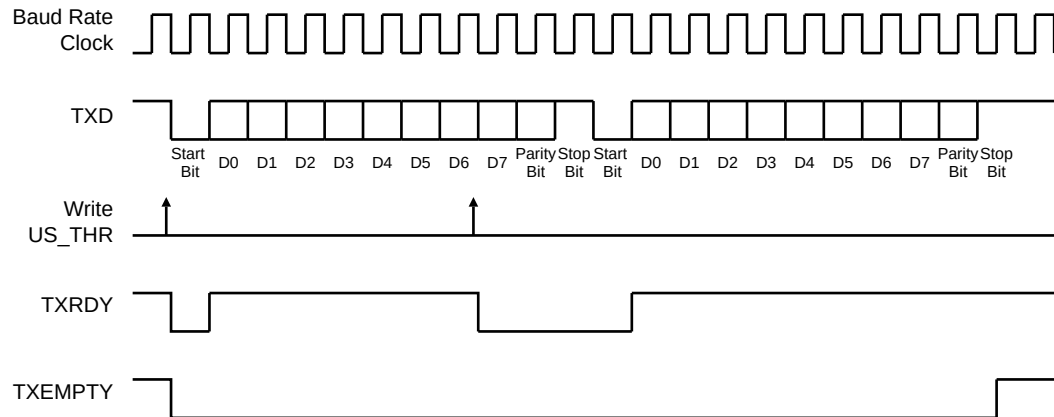
Figure 44-7. Transmitter Status
