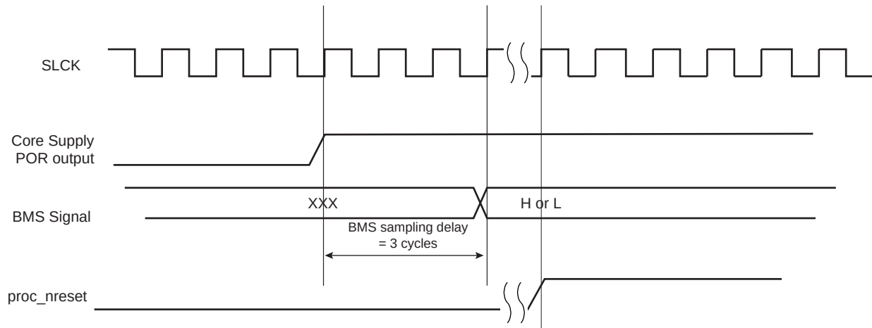
Figure 19-3. BMS Sampling
