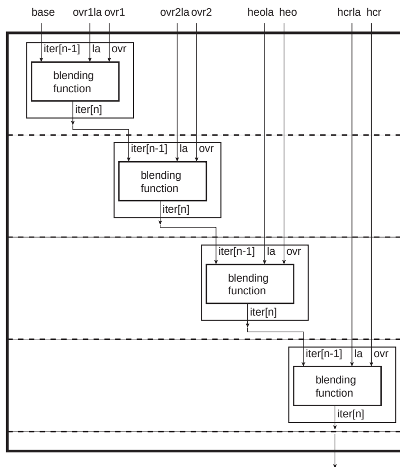
Figure 32-13.Global Alpha Blender
