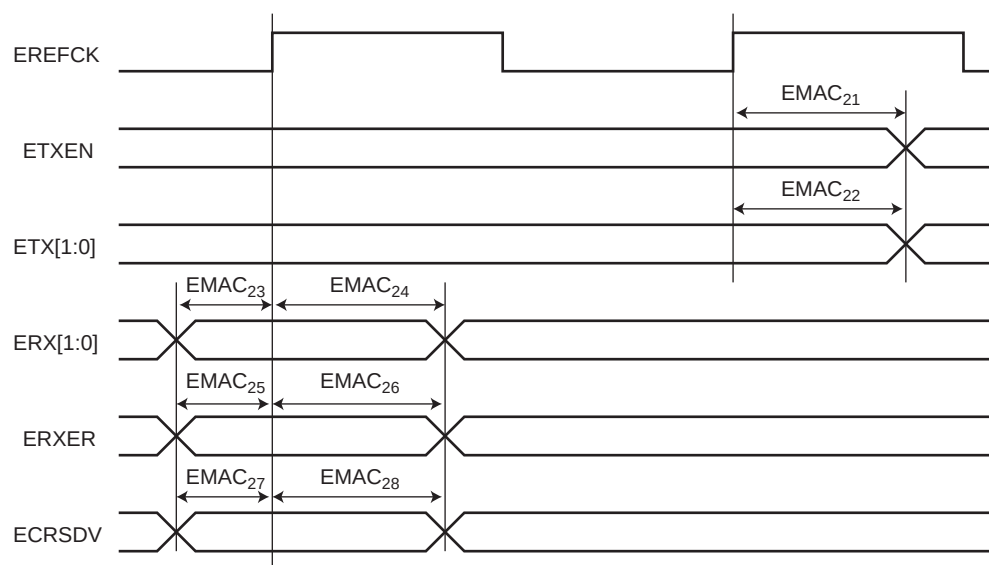
Figure 54-28.EMAC RMII Timings
