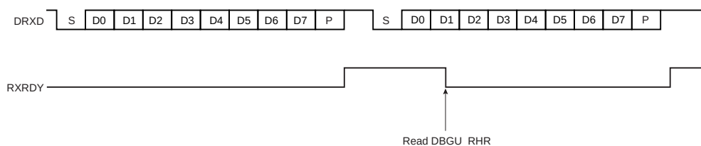
Figure 42-6. Receiver Ready
