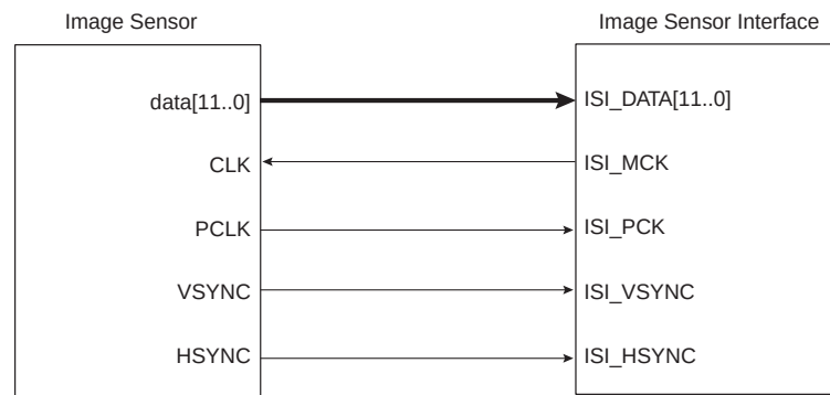
Figure 33-1. ISI Connection Example
