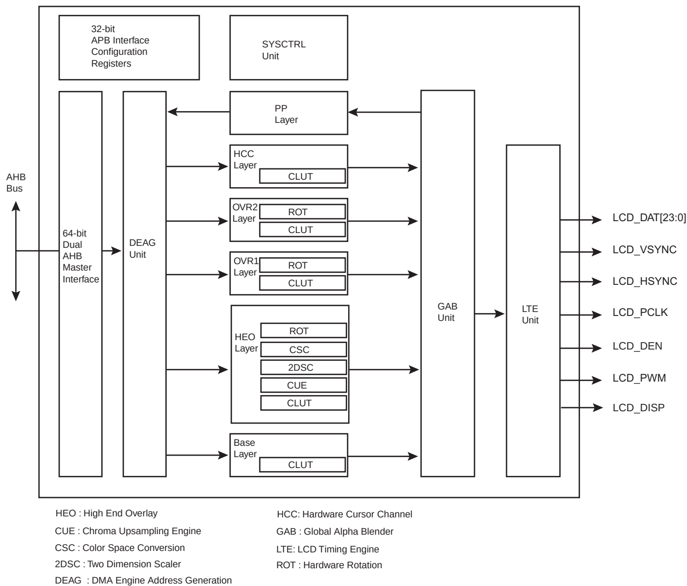
Figure 32-1. Block Diagram
