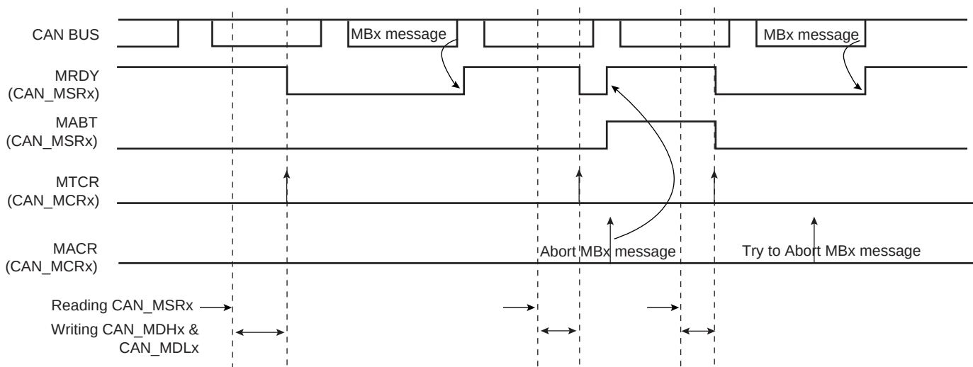
Figure 45-15. Transmitting Messages
