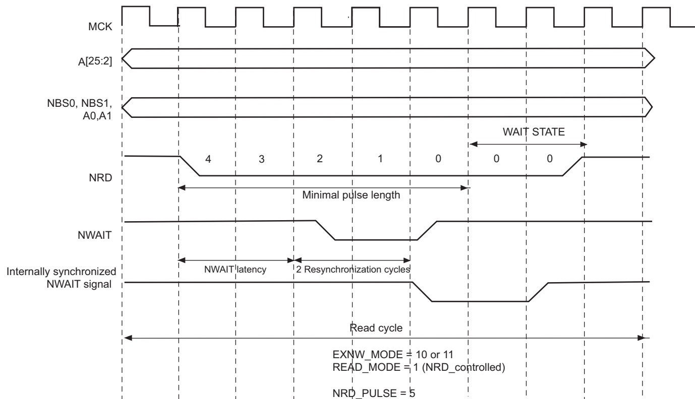
Figure 30-27.NWAIT Latency
