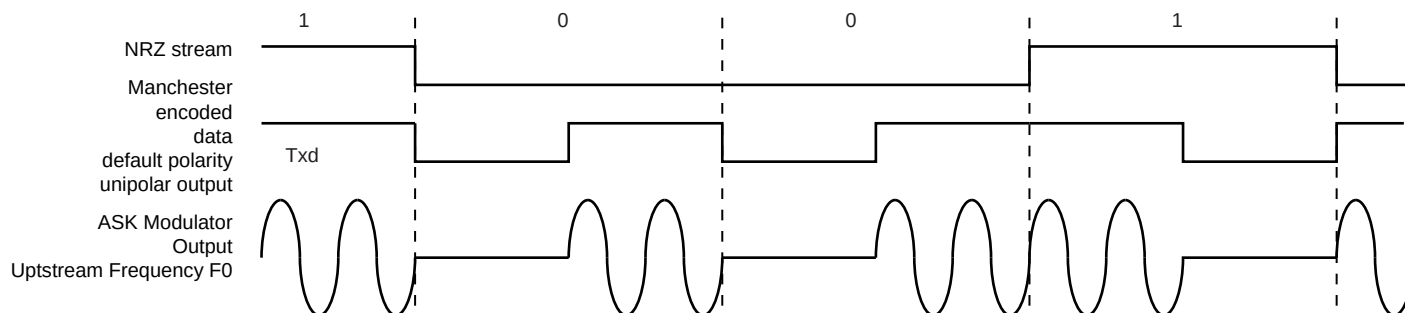
Figure 44-18.ASK Modulator Output
