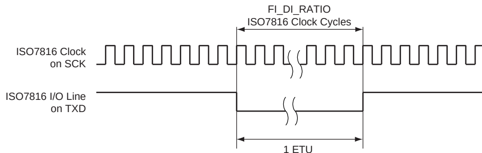
Figure 44-5. Elementary Time Unit (ETU)
