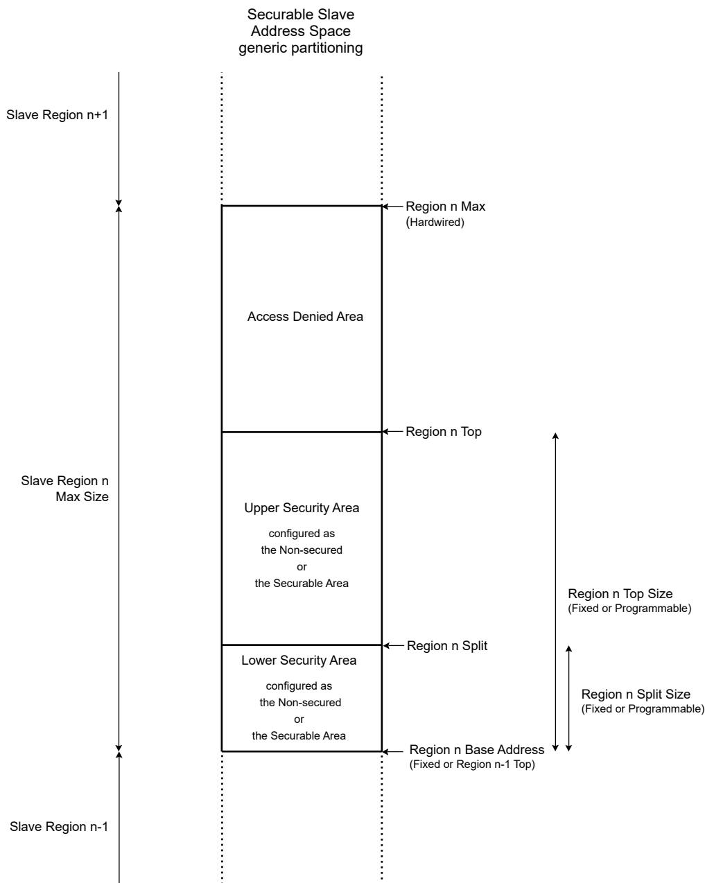
Figure 15-1: Generic Partitioning of the AHB Slave Address Space
