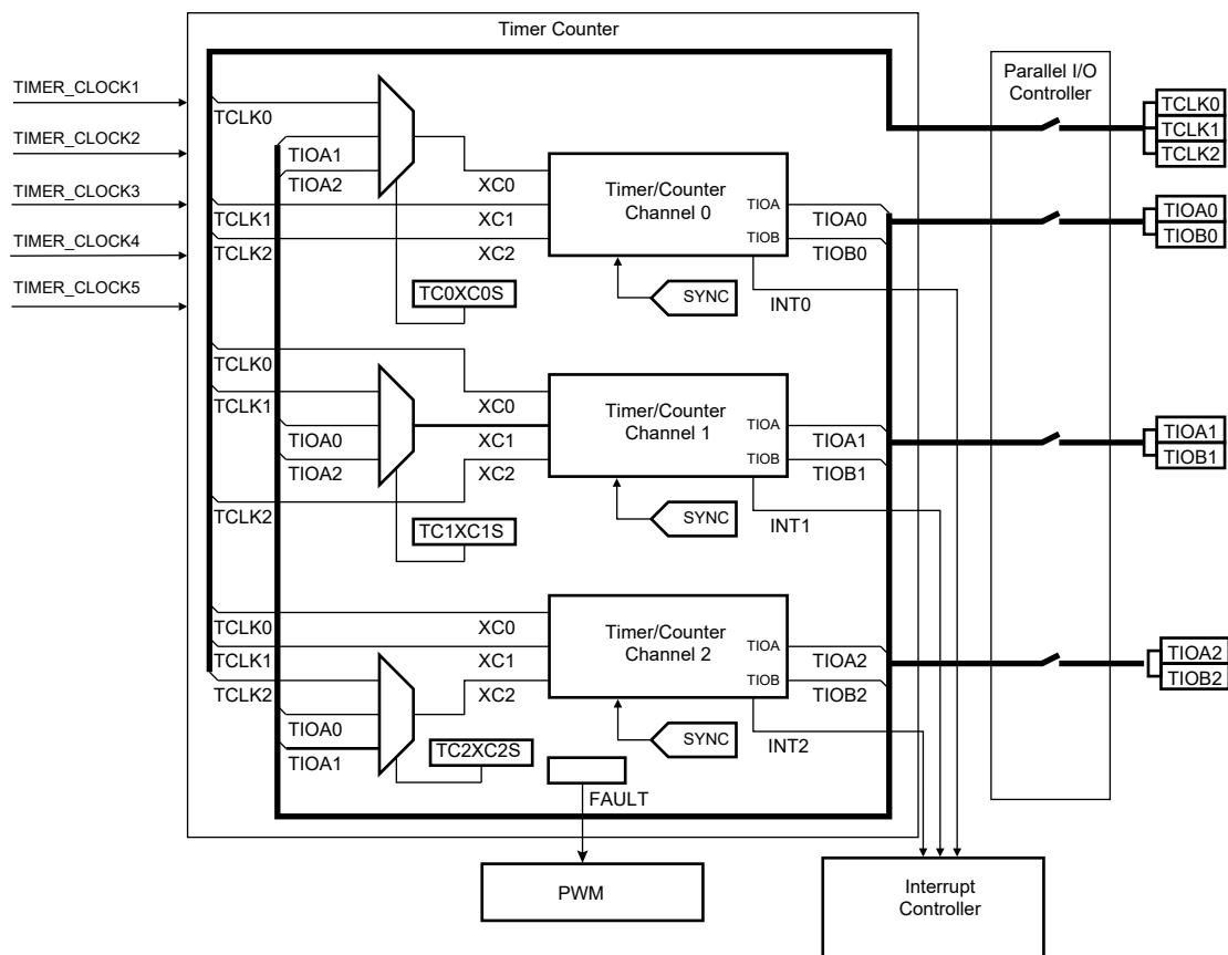
Figure 46-1: Block Diagram
