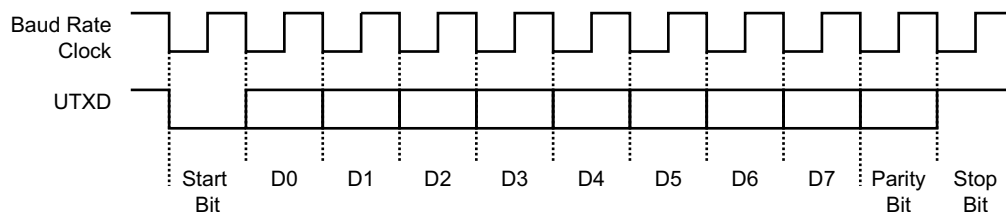
Figure 43-9: Character Transmission
