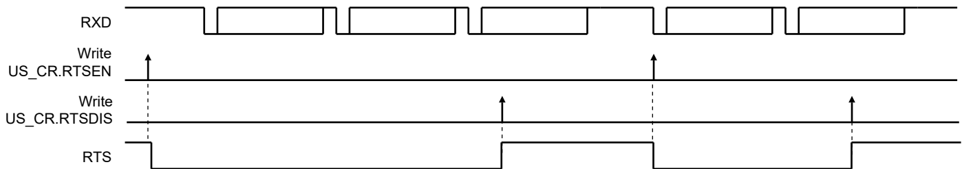
Figure 44-27: RTS Line Software Control when US_MR.USART_MODE = 2
