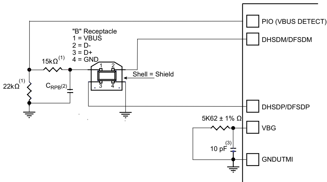
Figure 35-2: Board Schematic
