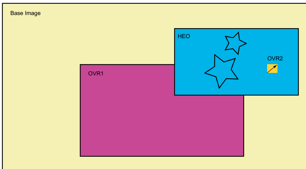
Video Prioritization Algorithm 2 : OVR2 &gt; HEO &gt; OVR1 &gt; BASE
