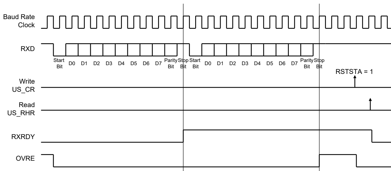
Figure 44-20: Receiver Status
