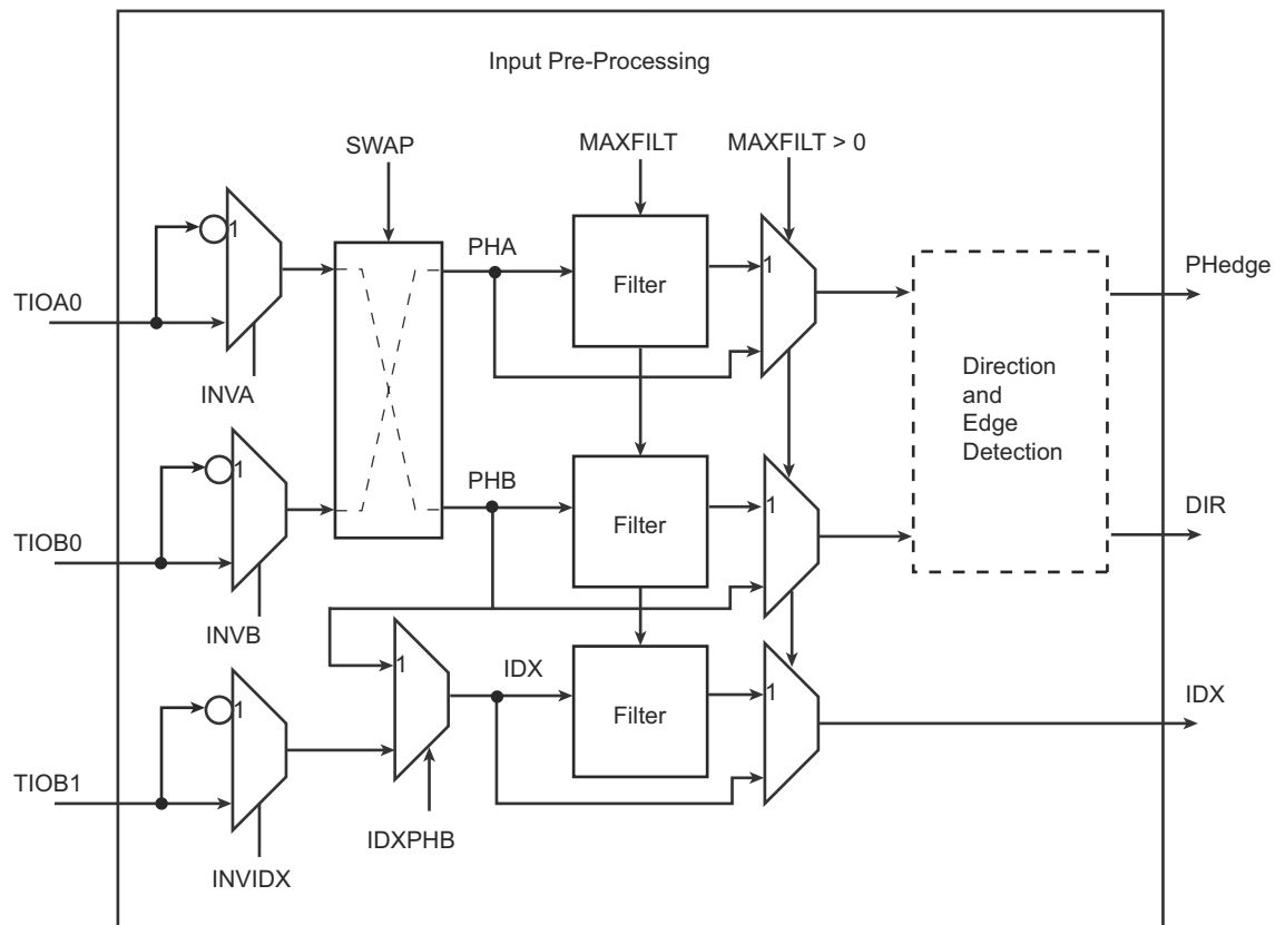
Figure 46-17: Input Stage
