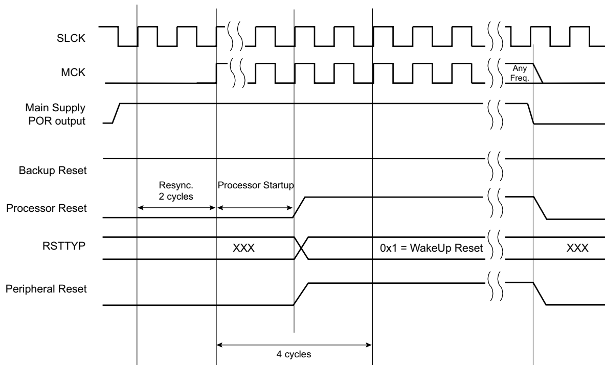
Figure 19-4: Wakeup Reset
