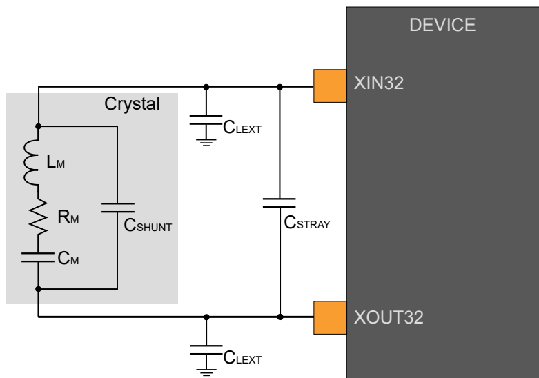
Figure 45-6. Oscillator Connection
