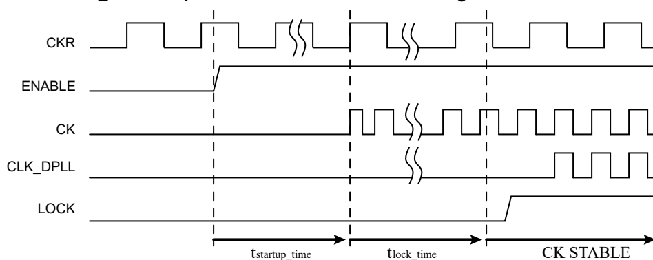
Figure 20-4. CK and CLK_DPLL Output from DPLL Off Mode to Running Mode
