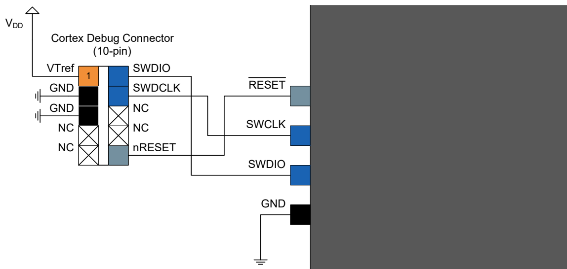
Figure 36-10. Cortex Debug Connector (10-pin)
