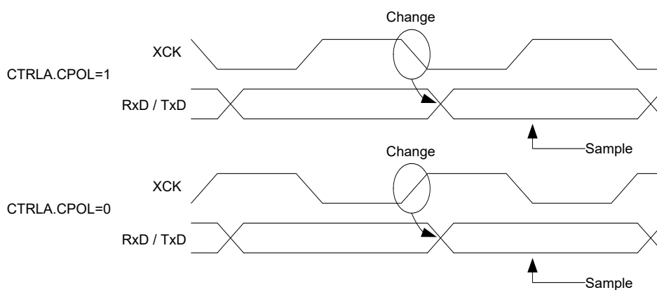
Figure 24-4. Synchronous Mode XCK Timing
