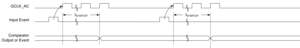
Figure 29-10. Single-Shot SleepWalking
