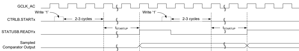
Figure 29-3. Single-Shot Example
