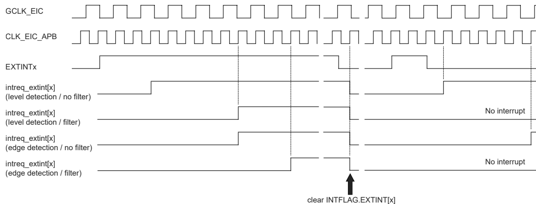
Figure 19-2. Interrupt Detections
