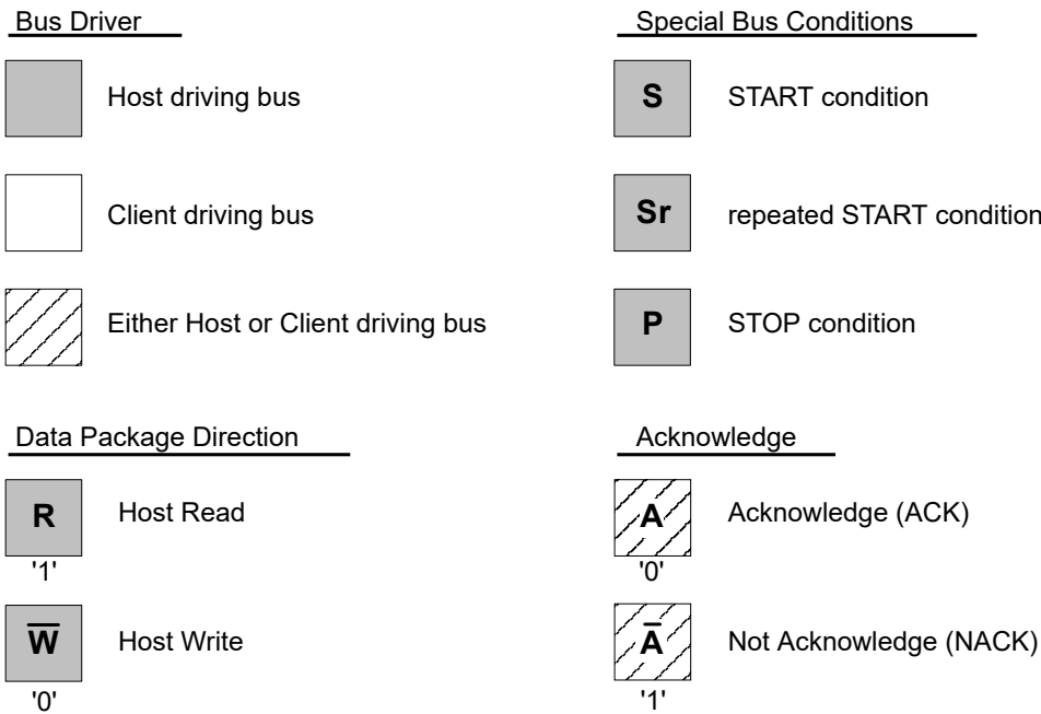
Figure 26-2. Transaction Diagram Symbols
