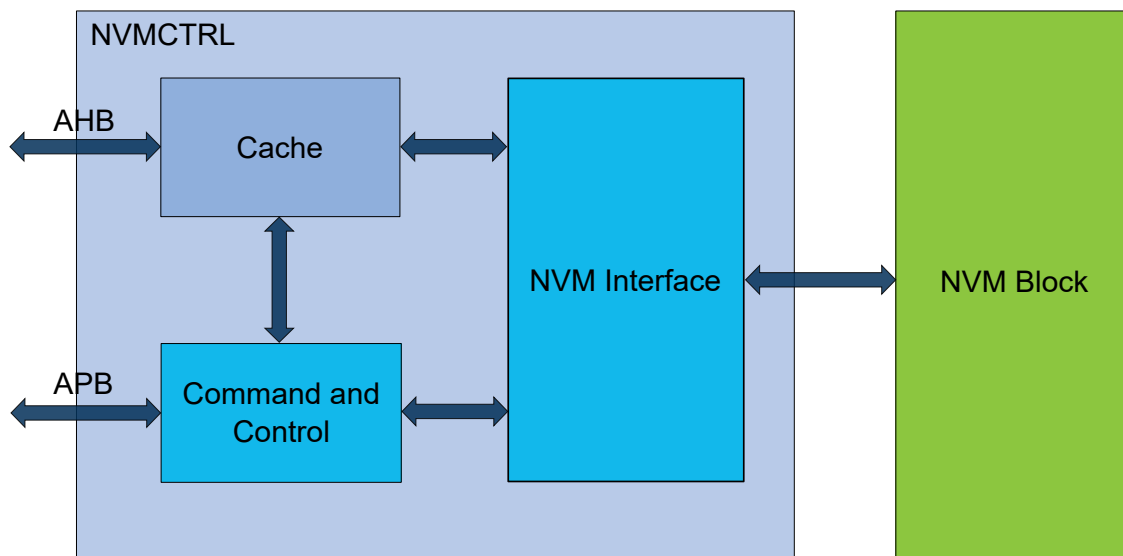
Figure 20-1. Block Diagram
