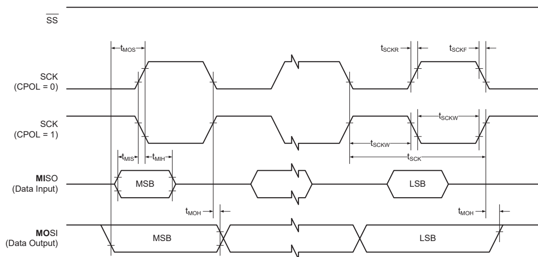
Figure 32-14. SPI timing requirements in Host mode
