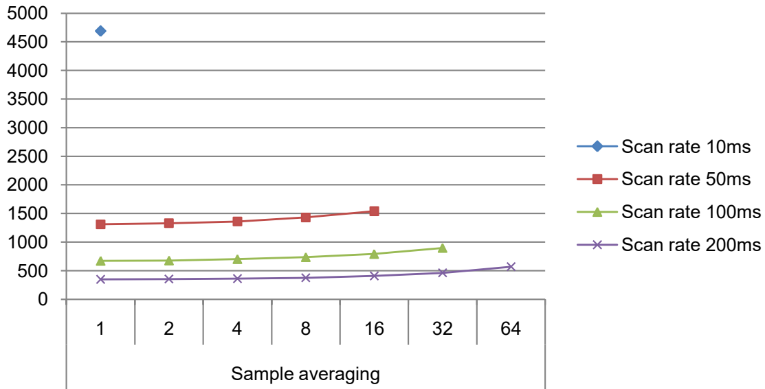
Figure 32-12. Power Consumption [ \mu\text{A} ]
