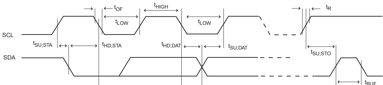
Figure 34-9. I 2 C Interface Bus Timing
