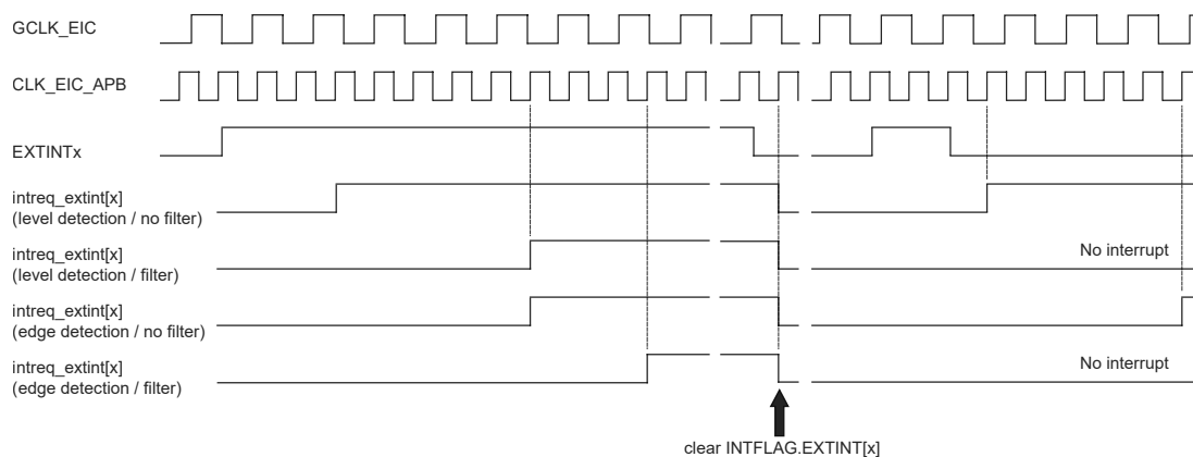
Figure 19-2. Interrupt Detections
