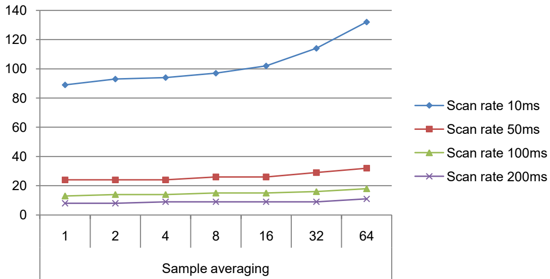
Figure 32-8. Power Consumption [ \mu\text{A} ]
