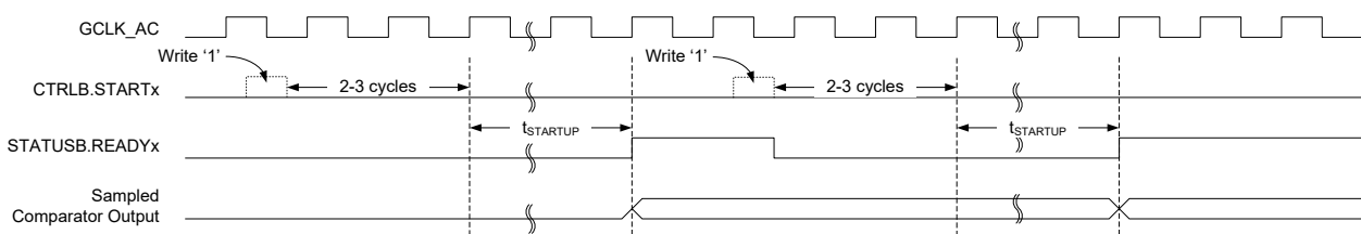
Figure 29-3. Single-Shot Example
