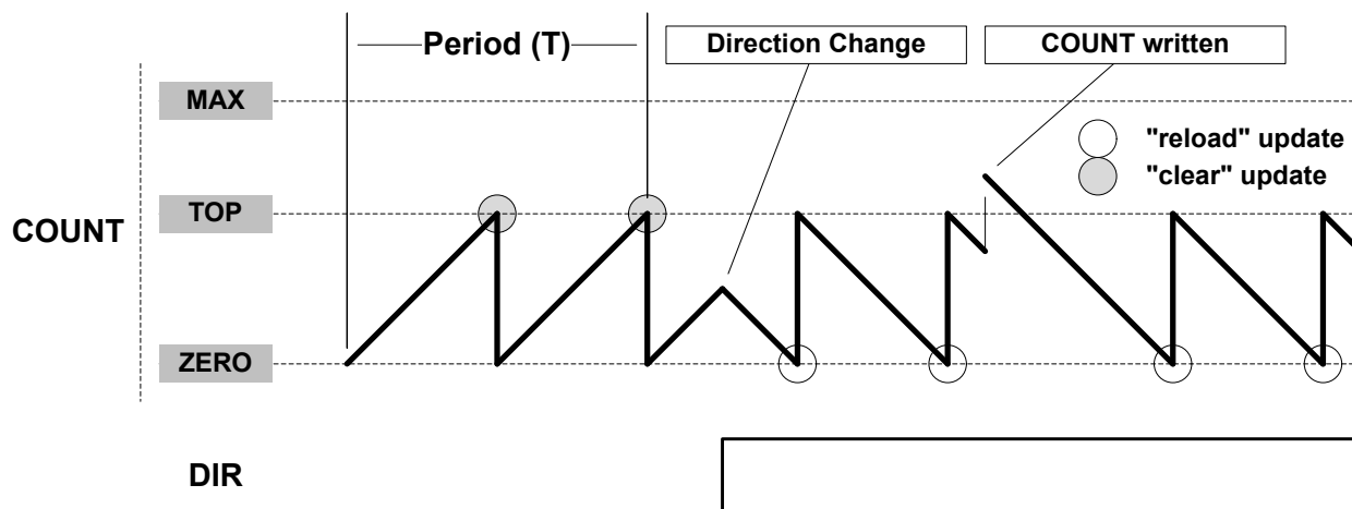
Figure 27-3. Counter Operation
