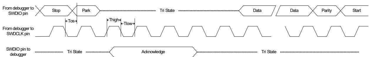
Figure 32-17. SWD Interface Signals
