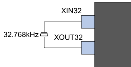
Figure 36-7. External Real-Time Oscillator without Load Capacitor
