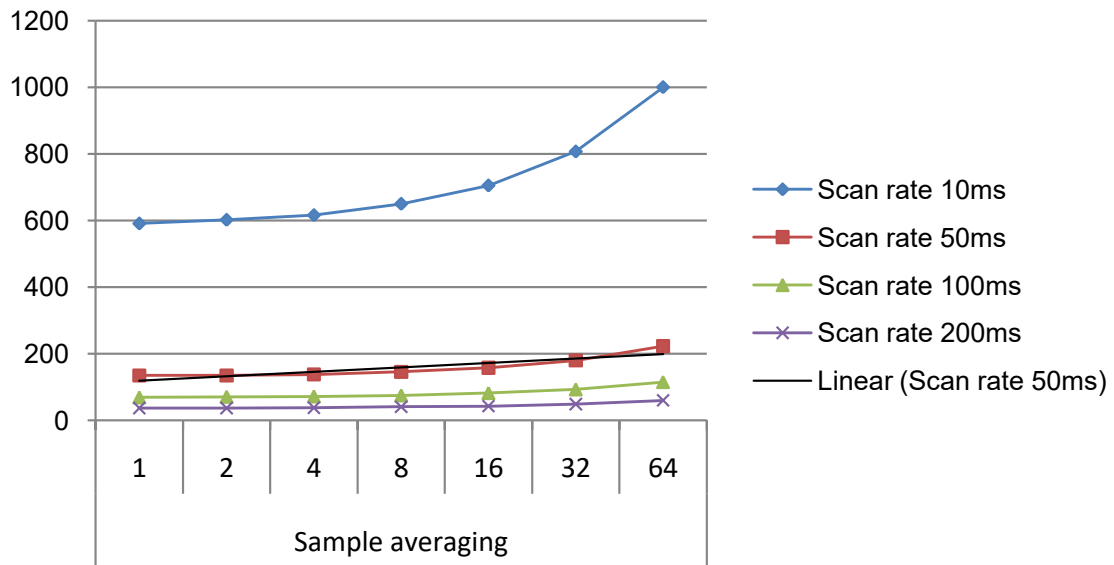
Figure 32-10. Power Consumption [ \mu\text{A} ]
