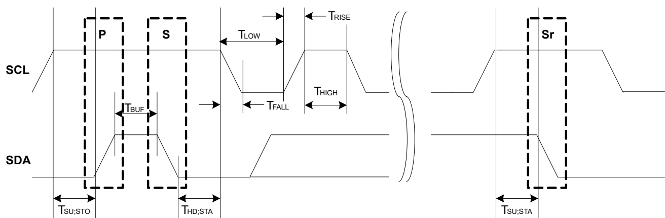
Figure 26-5. SCL Timing
