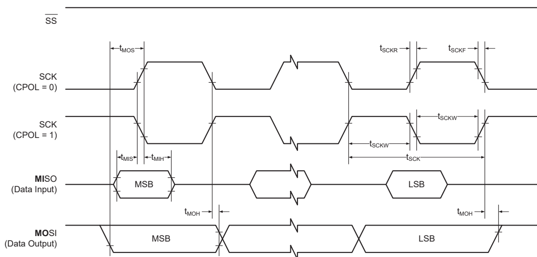
Figure 34-7. SPI Timing Requirements in Host Mode
