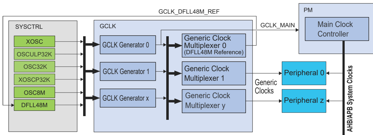
Figure 13-1. Clock distribution
