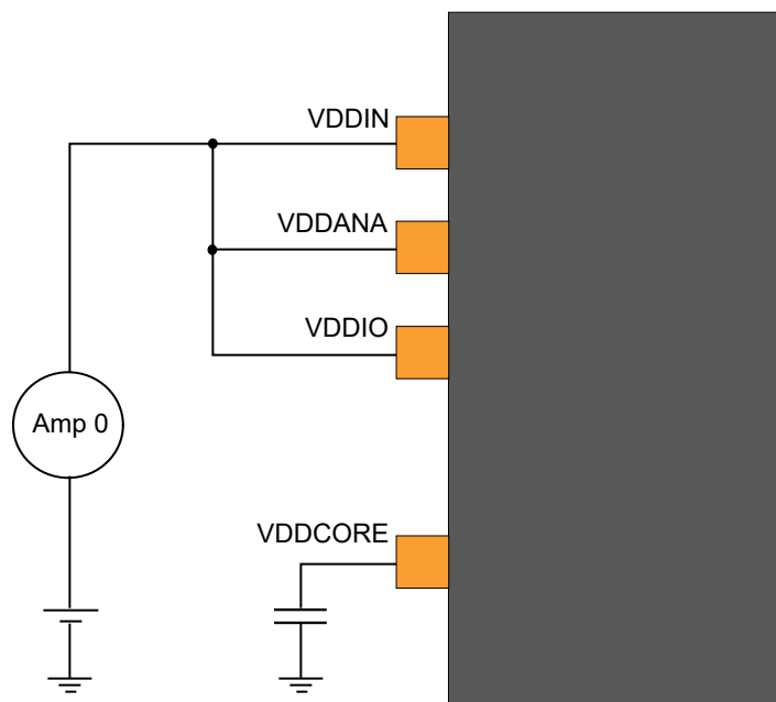
Figure 33-1. Measurement Schematic
