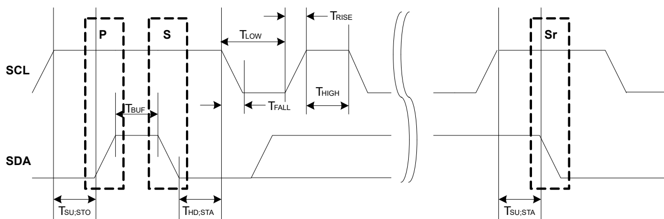
Figure 26-5. SCL Timing
