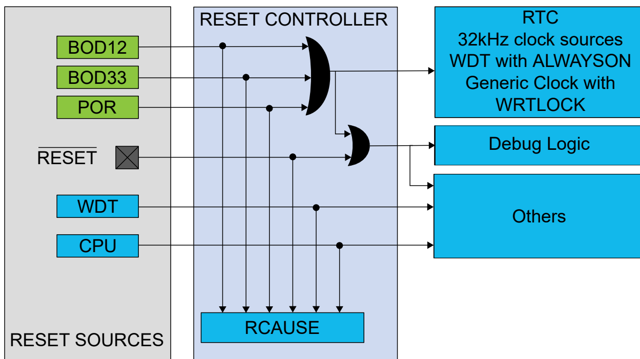
Figure 15-3. Reset Controller
