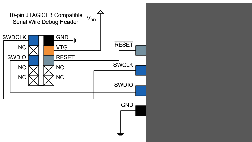
Figure 36-11. 10-pin JTAGICE3 Compatible Serial Wire Debug Interface
