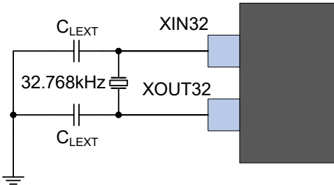
Figure 36-8. External Real-Time Oscillator with Load Capacitor
