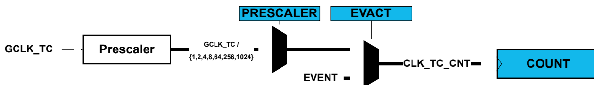
Figure 27-2. Prescaler
