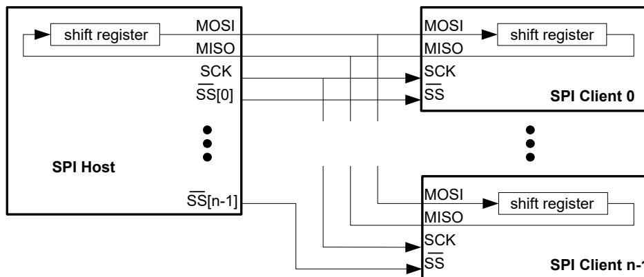
Figure 25-5. Multiple Clients in Parallel
