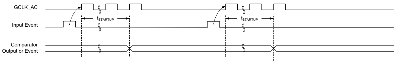
Figure 29-10. Single-Shot SleepWalking
