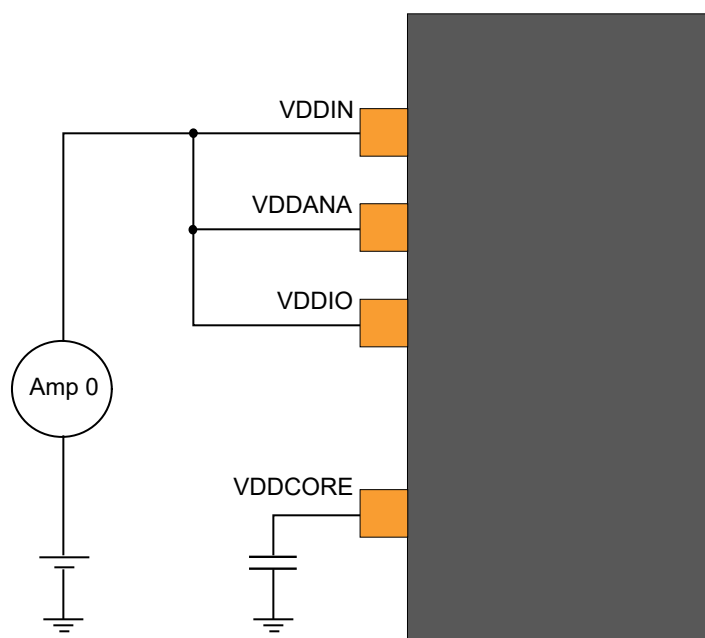
Figure 34-1. Measurement Schematic
