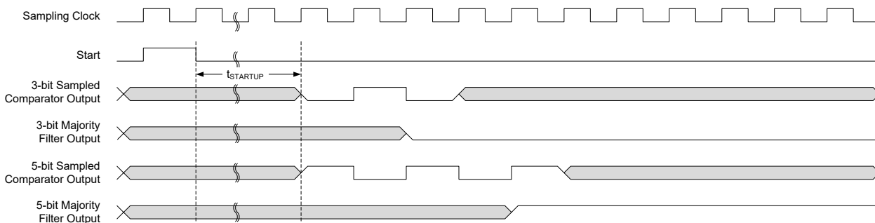
Figure 29-7. Single-Shot Filtering
