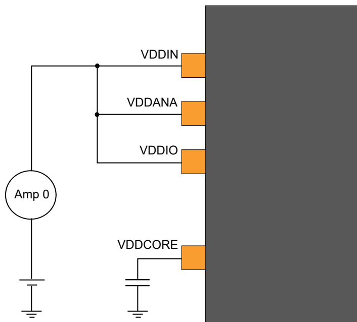
Figure 32-1. Measurement Schematic
