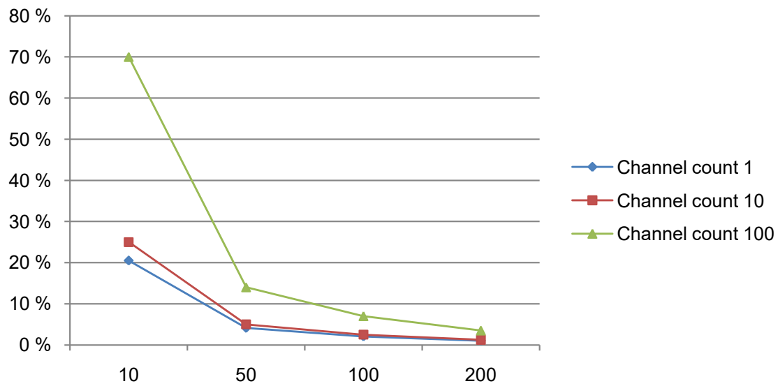
Figure 32-13. CPU Utilization
