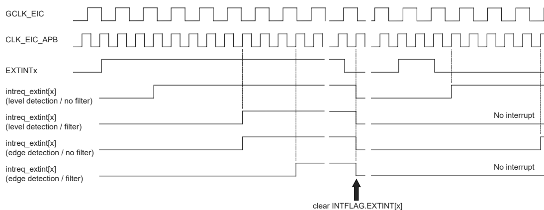
Figure 19-2. Interrupt Detections
