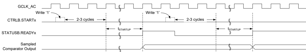
Figure 29-3. Single-Shot Example
