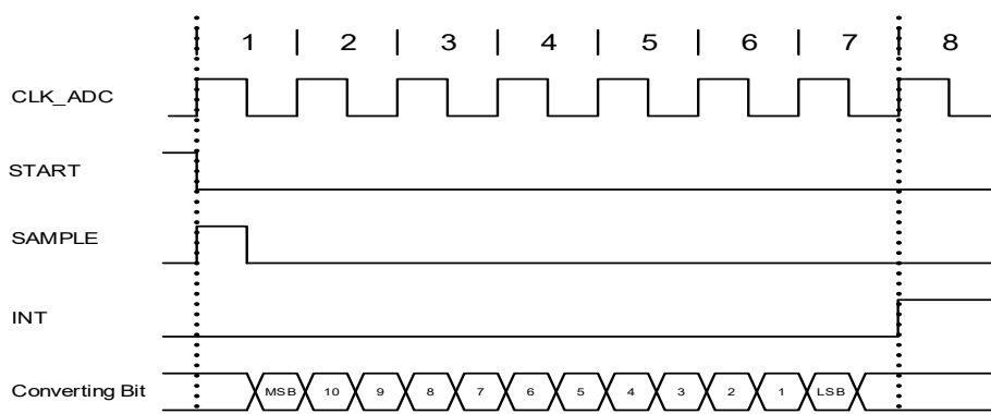
Figure 28-3. ADC Timing for One Conversion in Differential Mode without Gain
