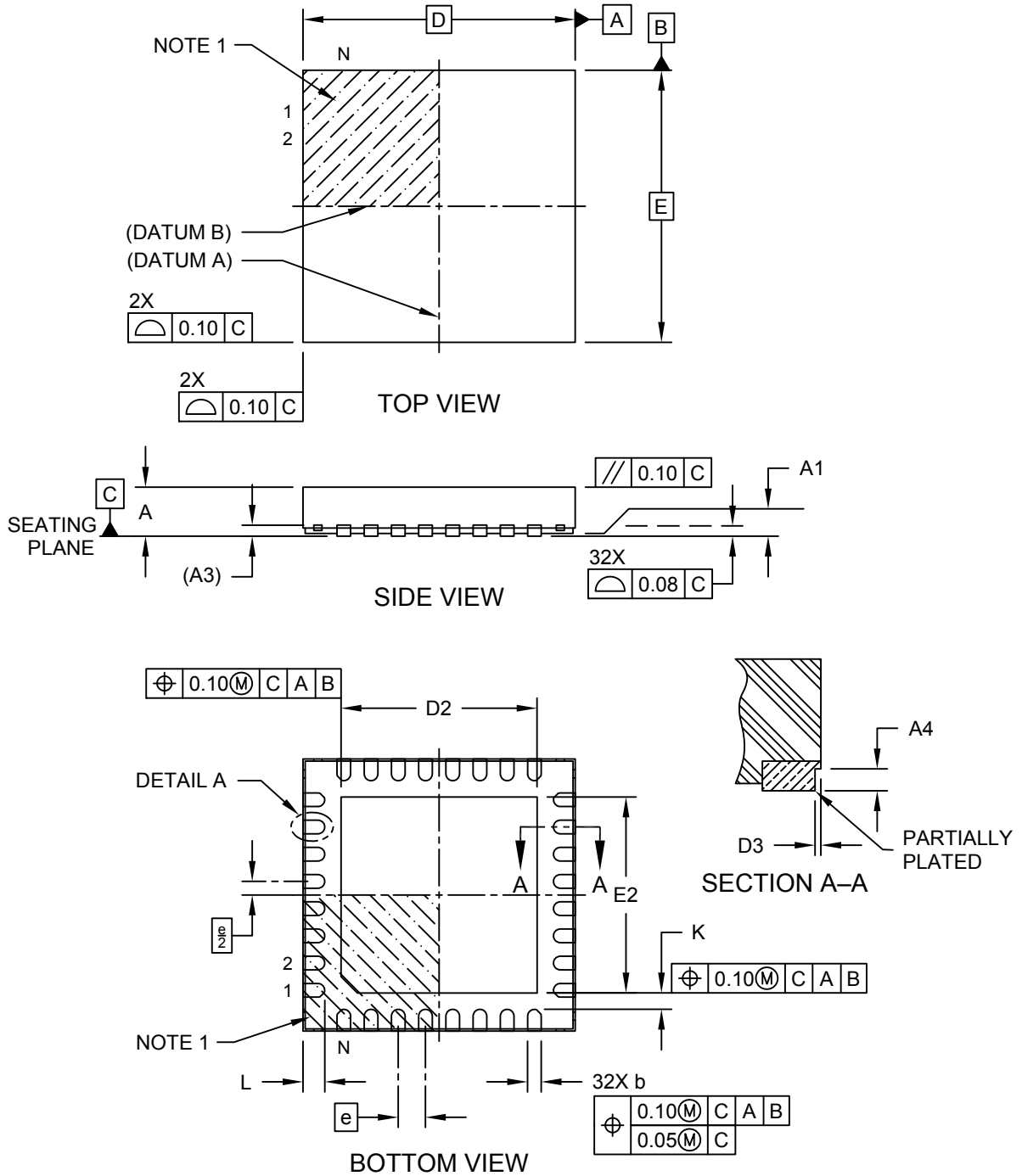
Microchip Technology Drawing C04-21391 Rev E Sheet 1 of 2
