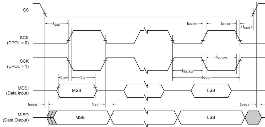
Figure 34-8. SPI Timing Requirements in Client Mode
