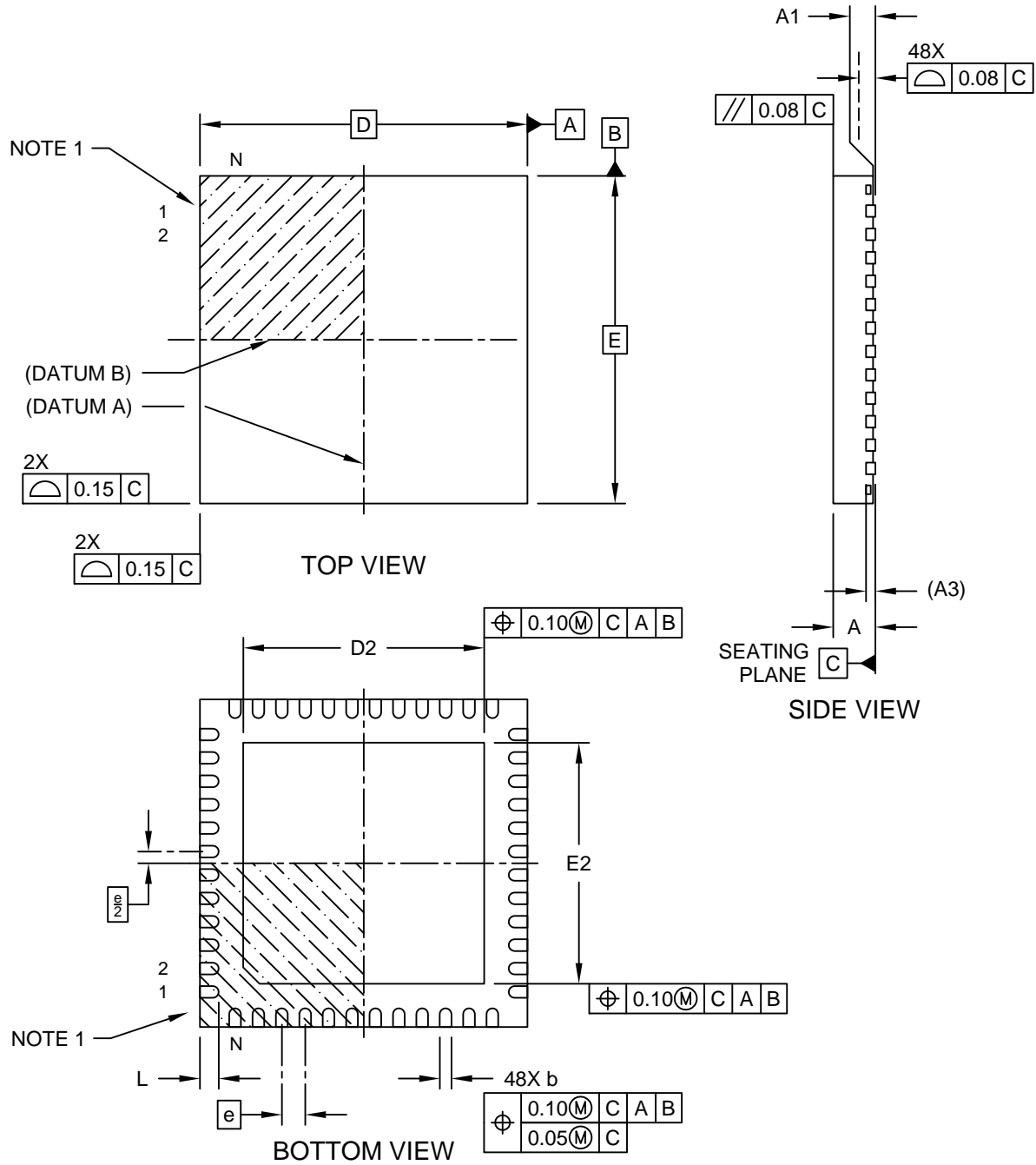
Microchip Technology Drawing C04-21425 Rev A Sheet 1 of 2
