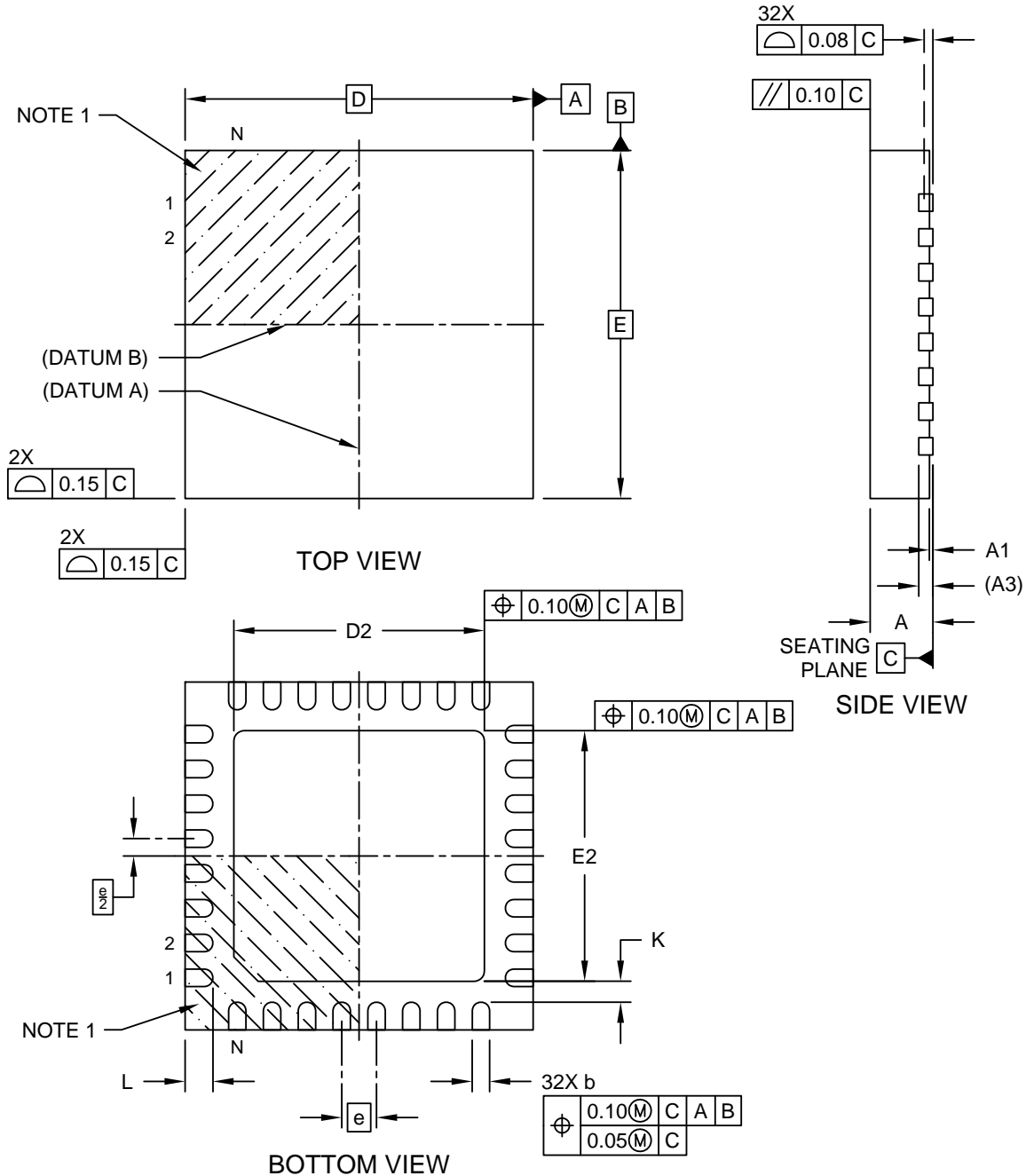
Microchip Technology Drawing C04-21402 Rev A Sheet 1 of 2
