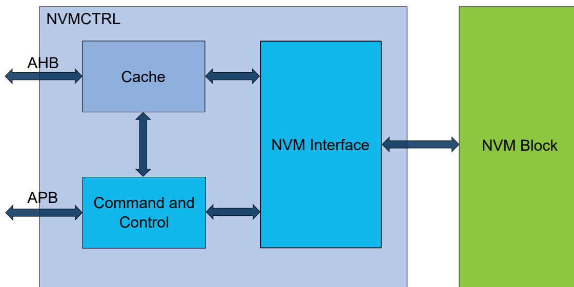
Figure 20-1. Block Diagram
