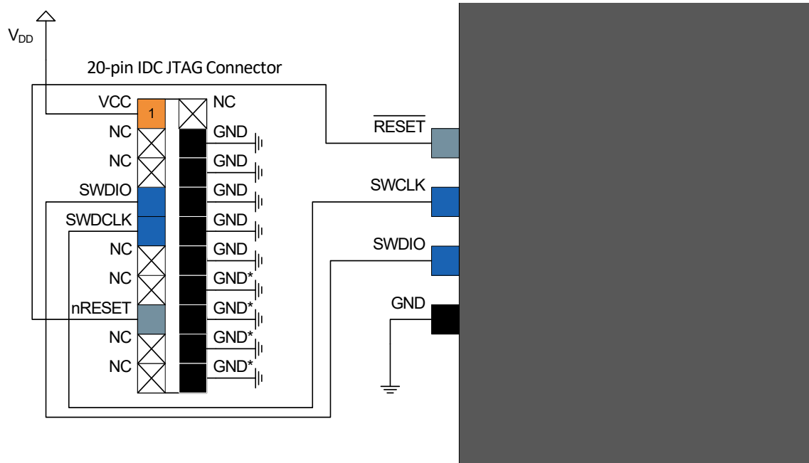
Figure 36-12. 20-pin IDC JTAG Connector
