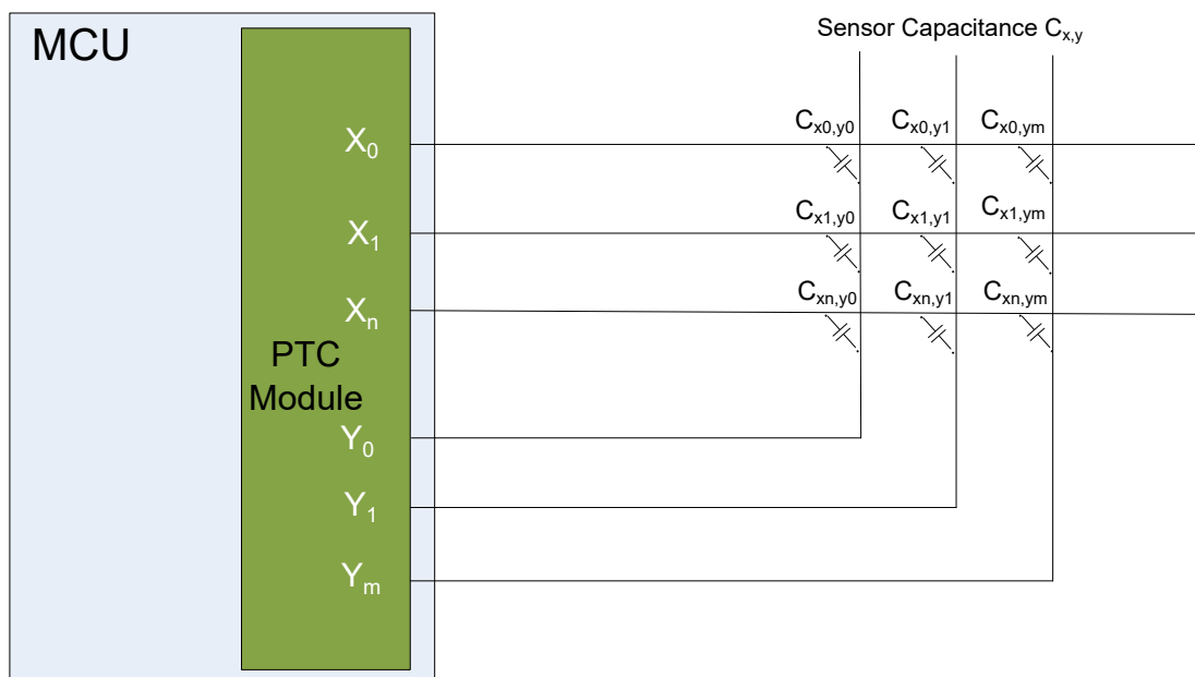
Figure 31-3. Mutual Capacitance Sensor Arrangement
