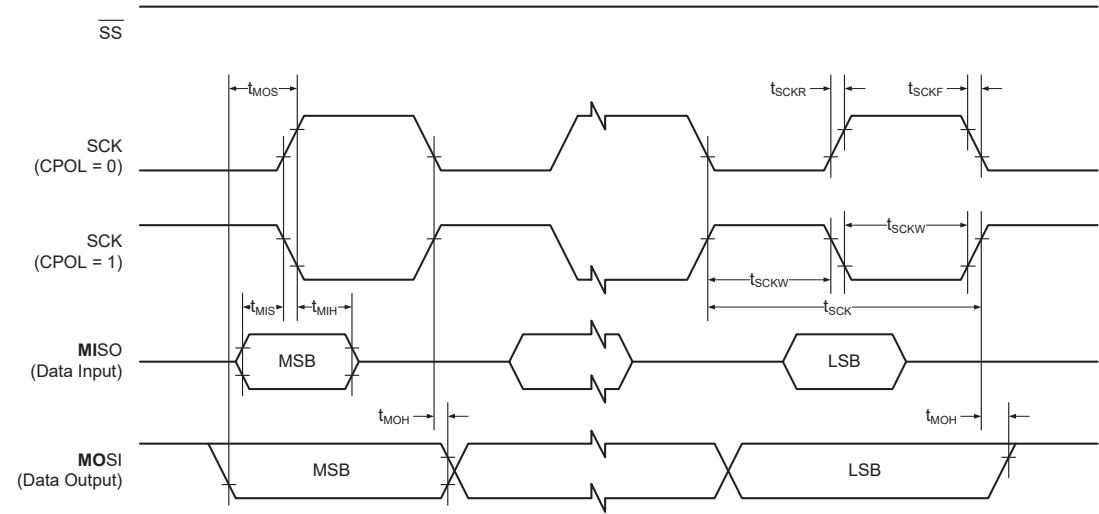
Figure 32-14. SPI timing requirements in Host mode
