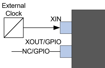
Figure 36-5. External Clock Source Example Schematic
