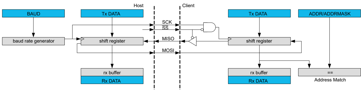
Figure 25-1. Full-Duplex SPI Host Client Interconnection
