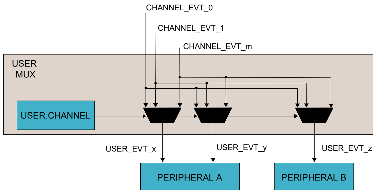
Figure 22-2. User MUX
