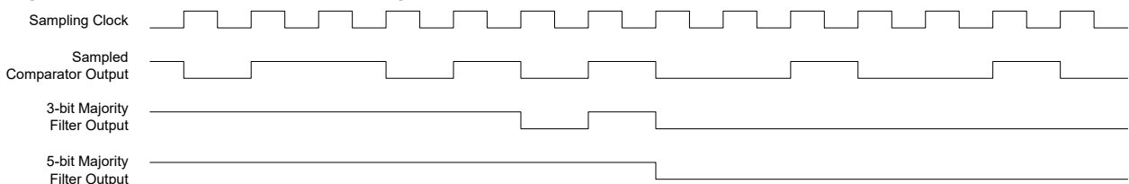
Figure 34-7. Continuous Mode Filtering
