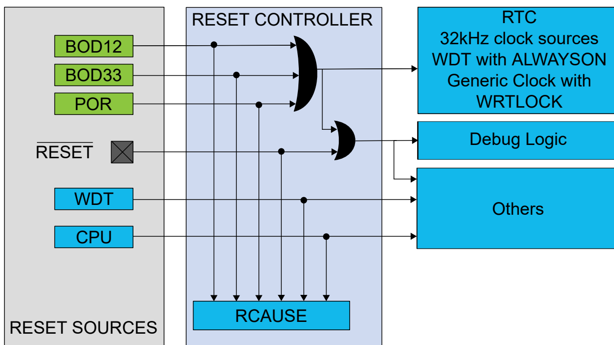
Figure 16-3. Reset Controller
