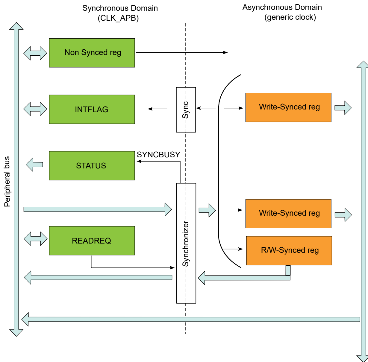
Figure 14-3. Synchronization
