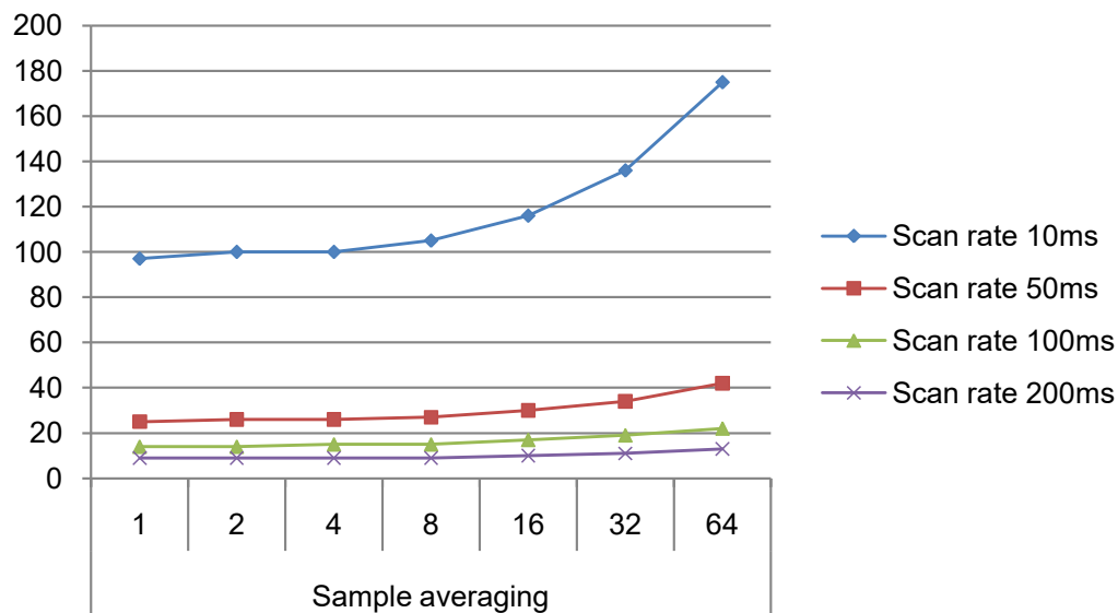
Figure 37-9. Power Consumption [ \mu A]
