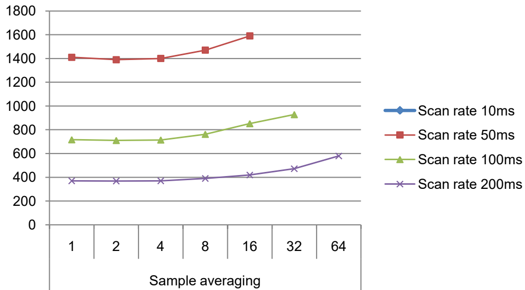
Figure 41-12. Power Consumption [ \mu A]
