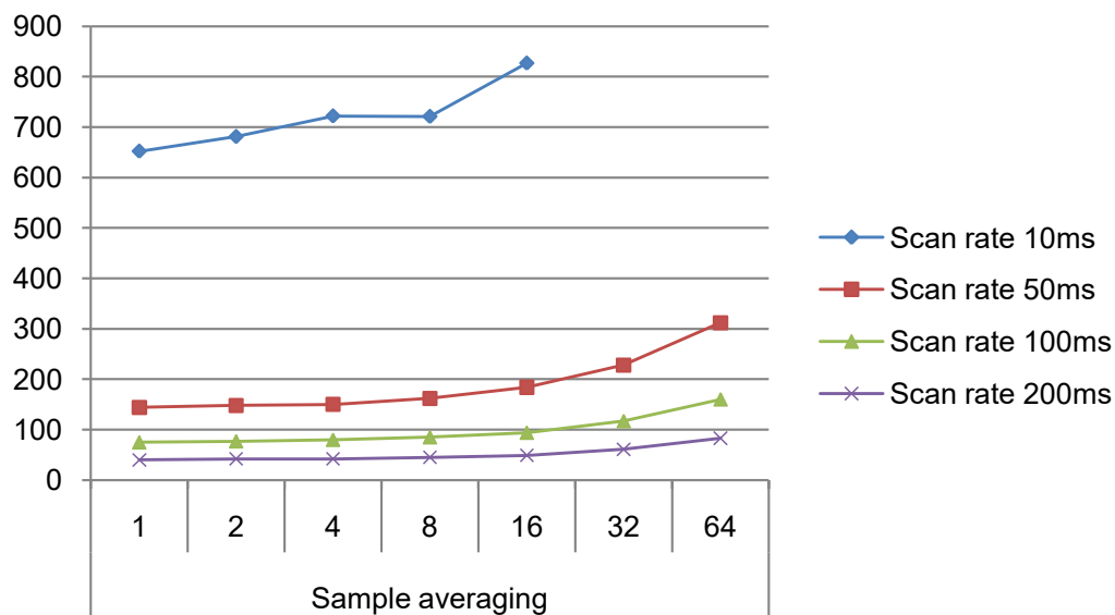
Figure 37-11. Power Consumption [ \mu A]
