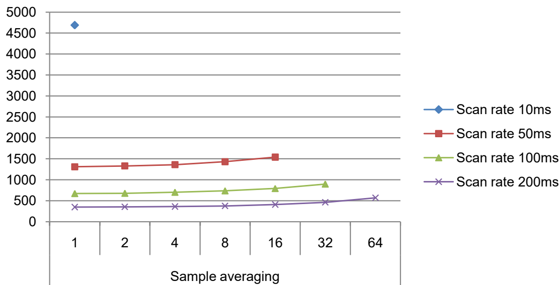
Figure 41-12. Power Consumption [ \mu\text{A} ]
