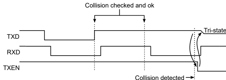
Figure 26-13. Collision Detected
