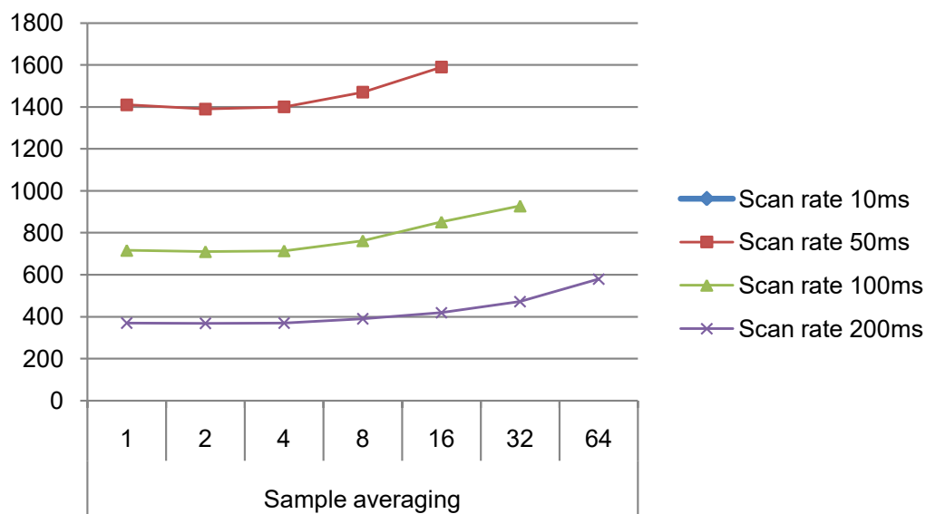
Figure 41-12. Power Consumption [ \mu\text{A} ]
