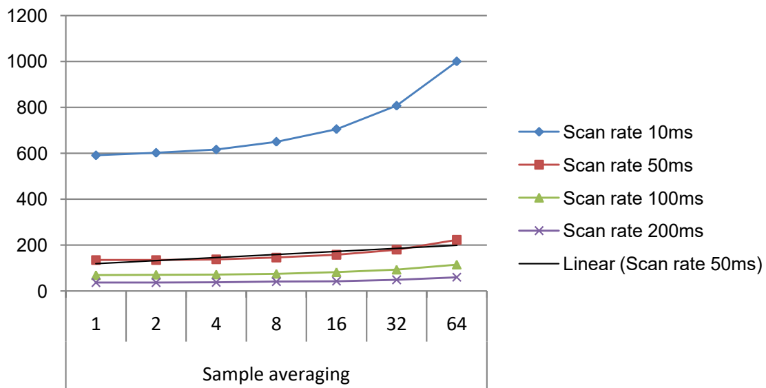
Figure 37-9. Power Consumption [ \mu A]
