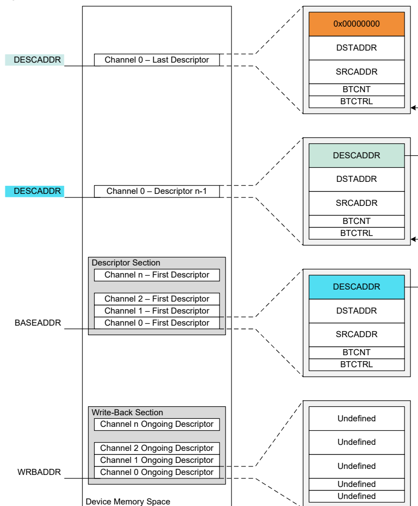
Figure 20-3. Memory Sections
