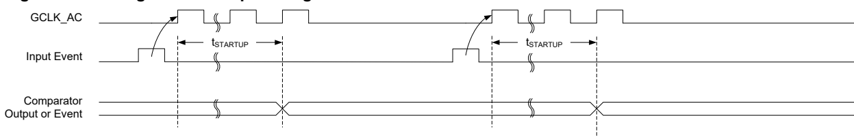
Figure 34-11. Single-Shot SleepWalking
