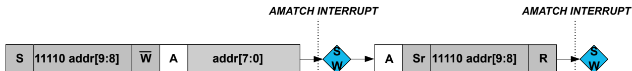
Figure 28-12. 10-bit Addressing
