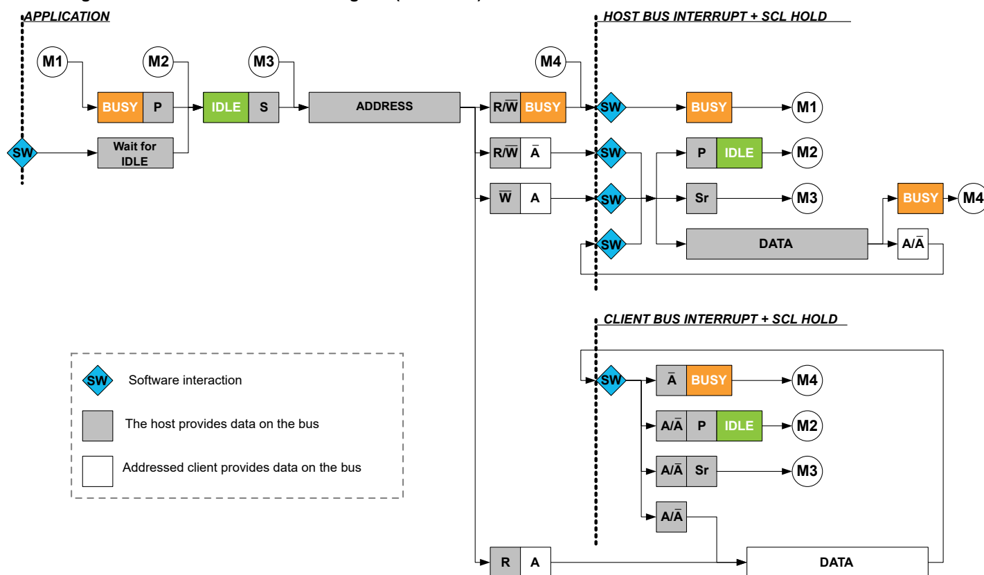
Figure 28-5. I 2 C Host Behavioral Diagram (SCLSM=0)
