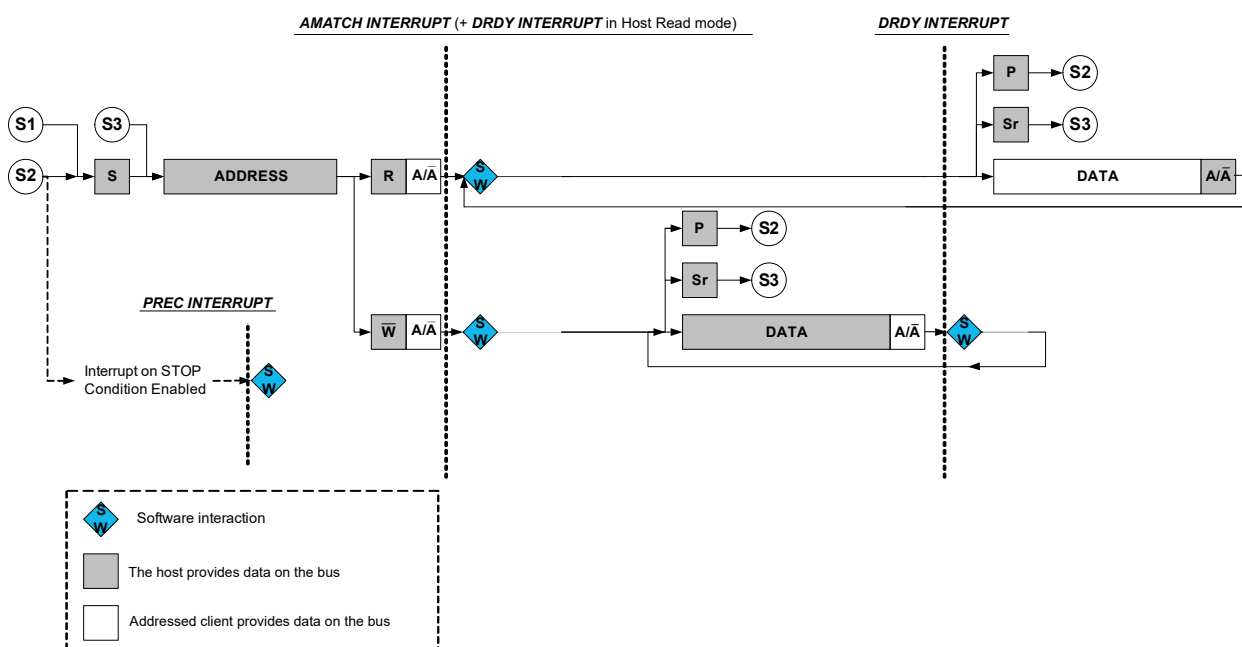
Figure 28-11. I 2 C Client Behavioral Diagram (SCLSM=1)
