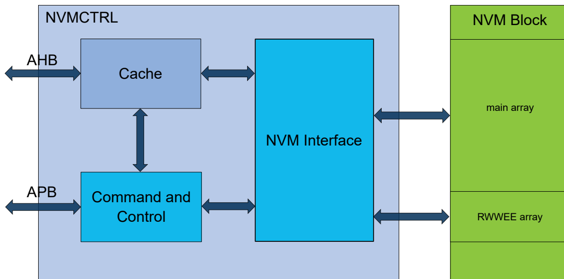
Figure 22-1. Block Diagram
