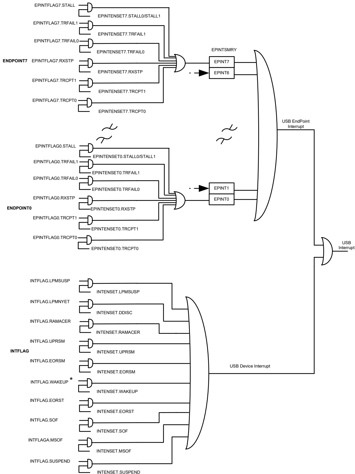
Figure 32-9. Device Interrupt
