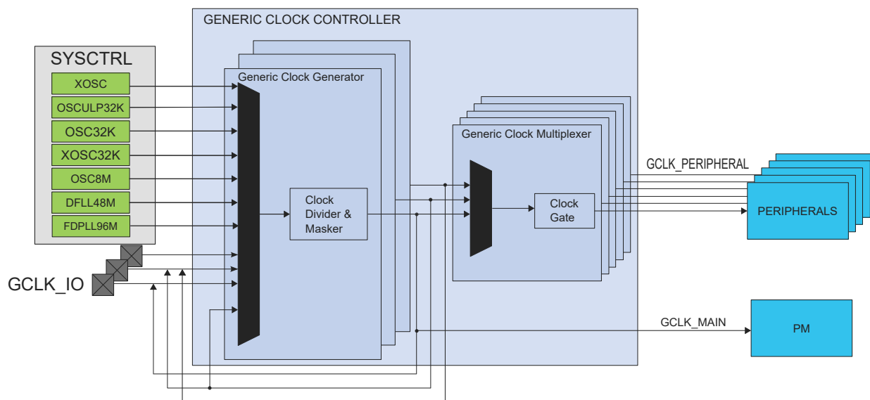
Figure 15-1. Device Clocking Diagram
