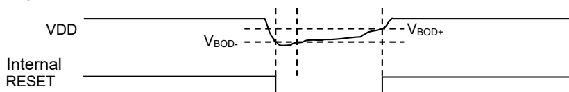
Figure 41-4. BOD33 Hysteresis ON
