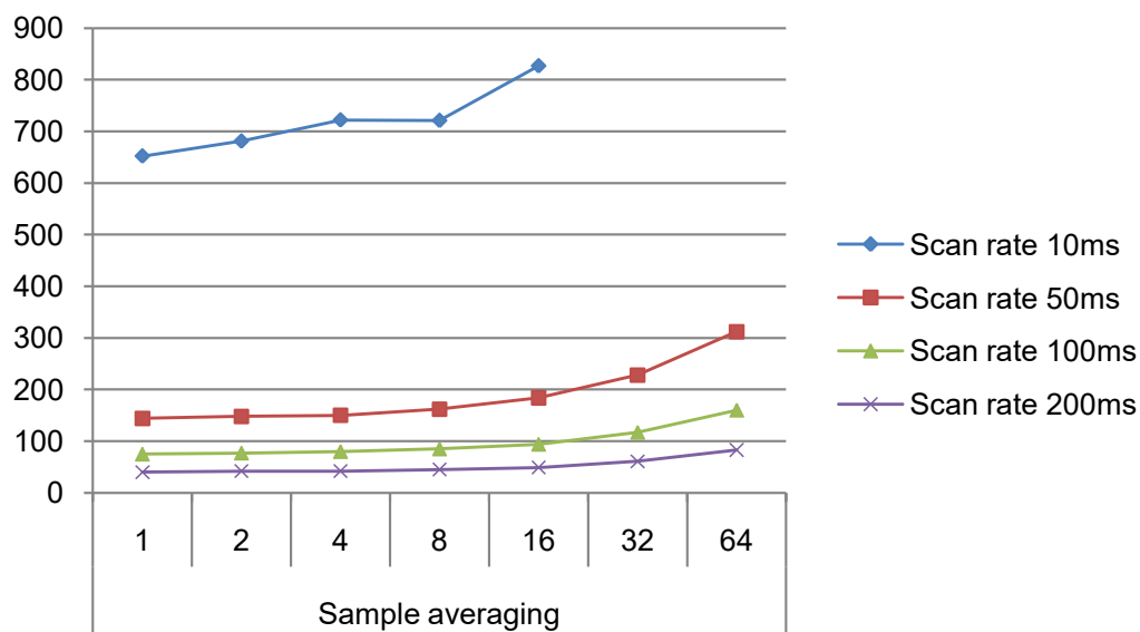
Figure 41-10. Power Consumption [ \mu A]
