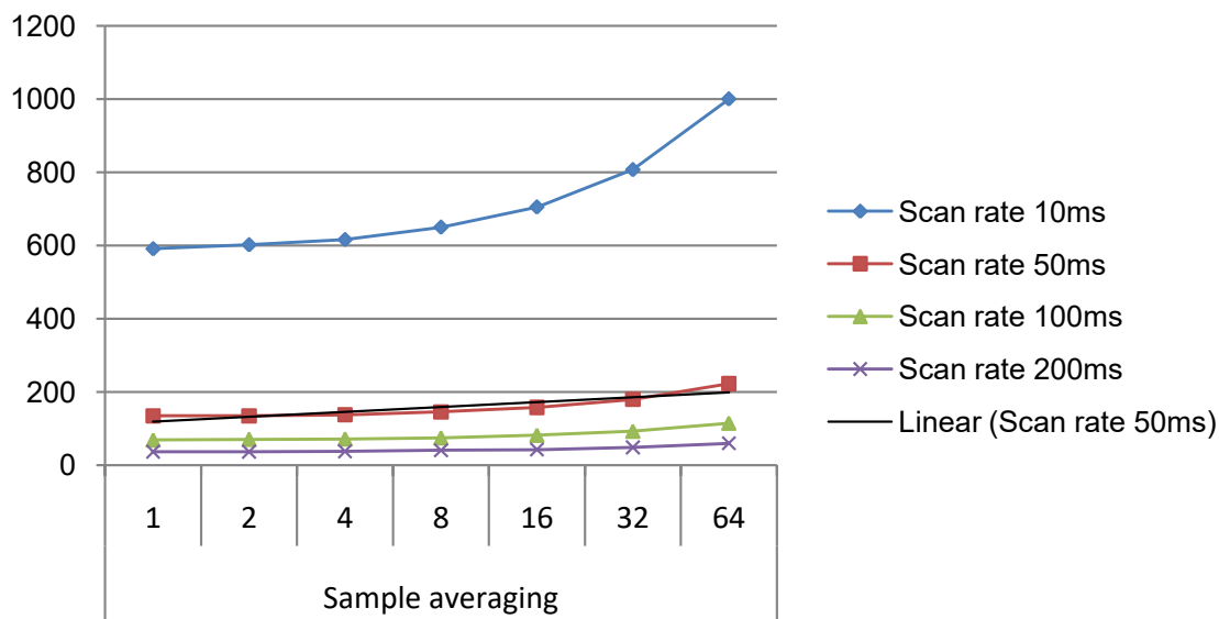
Figure 41-10. Power Consumption [ \mu\text{A} ]
