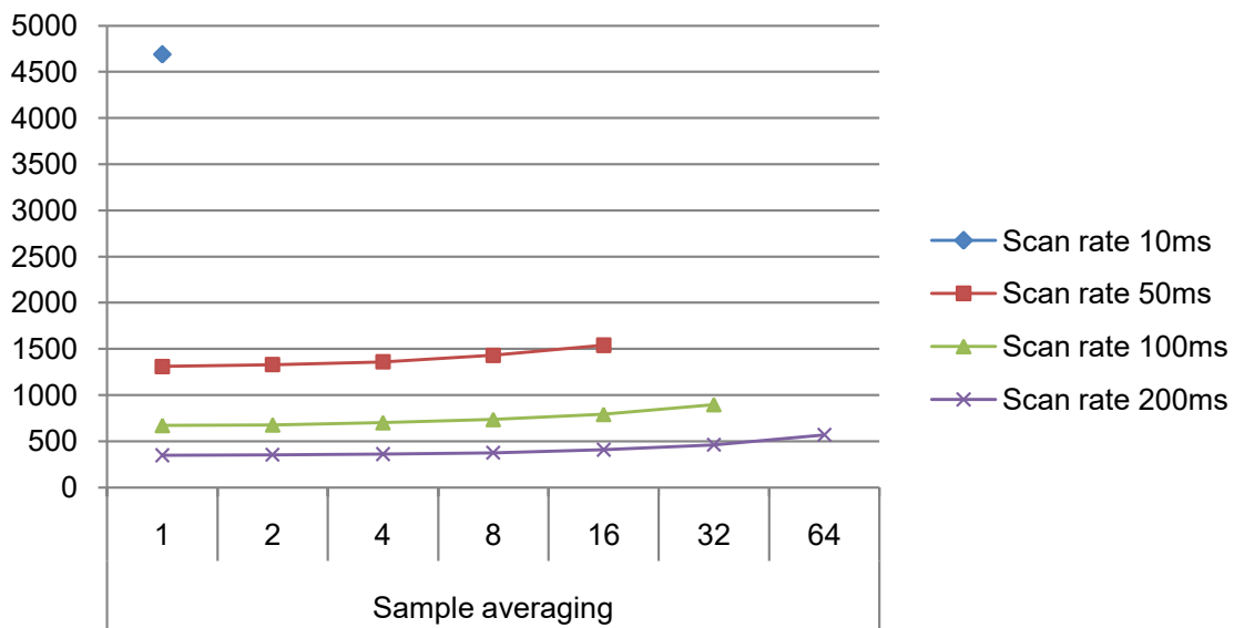
Figure 37-11. Power Consumption [ \mu A]
