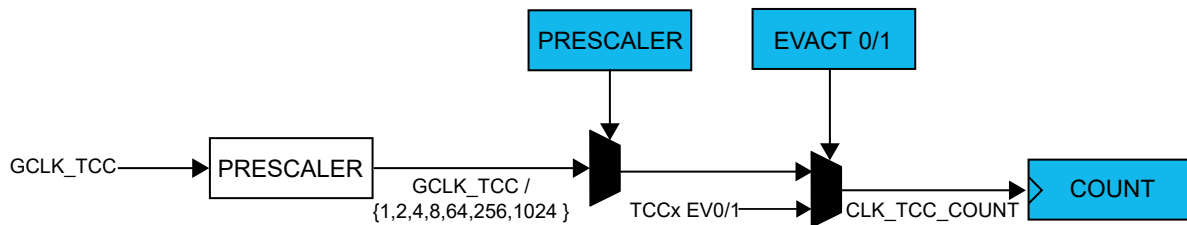
Figure 31-2. Prescaler
