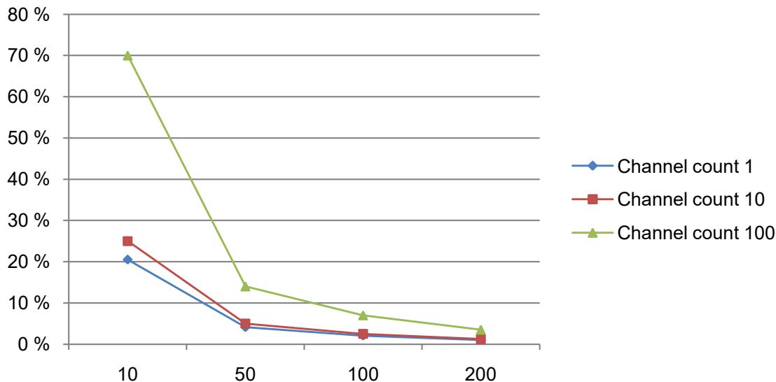
Figure 41-13. CPU Utilization
