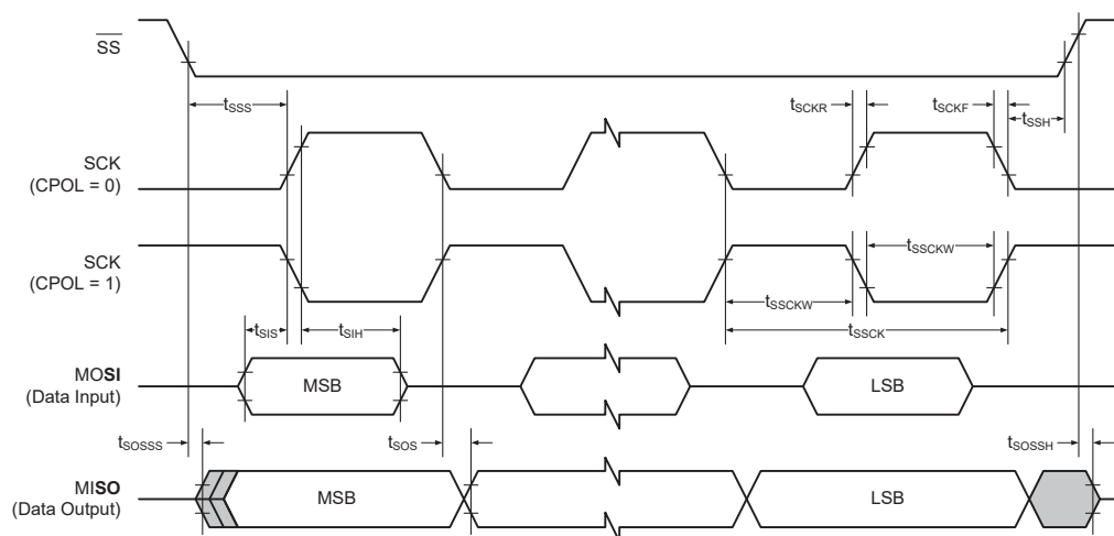
Figure 37-21. SPI Timing Requirements in Client Mode
