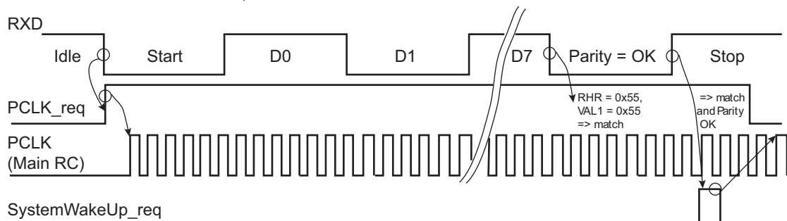
Figure 30-27. Asynchronous Wakeup Use Case Examples
