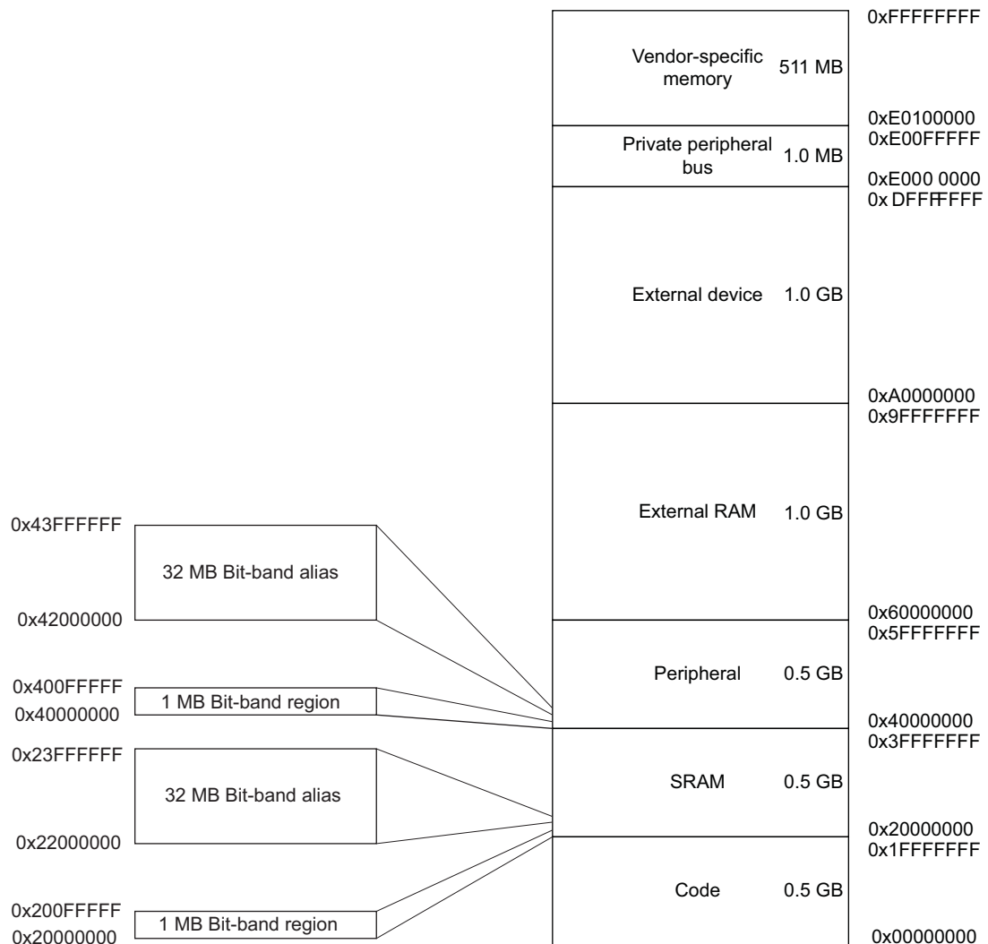
Figure 13-3. Memory Map
