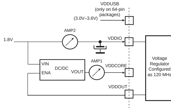
Figure 39-6. Wait Mode Measurement Setup (Dual Supply)
