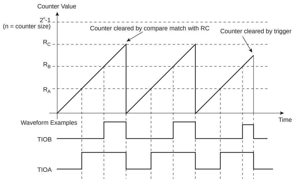
Figure 24-11. WAVSEL = 10 with Trigger
