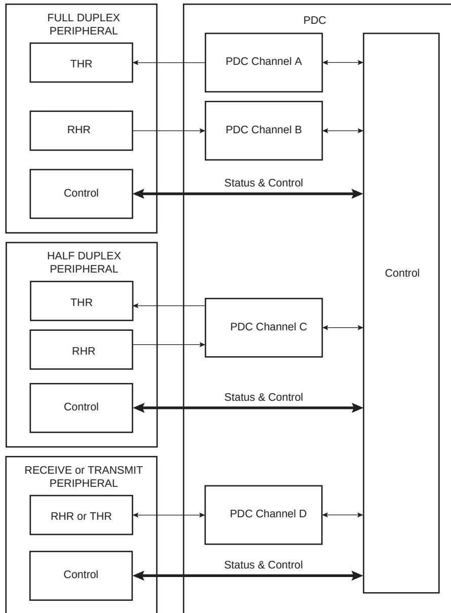
Figure 21-1. Block Diagram
