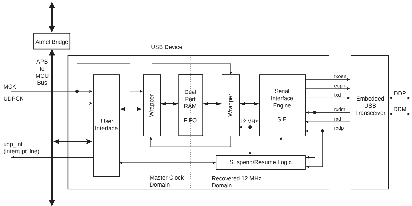
Figure 37-1. Block Diagram
