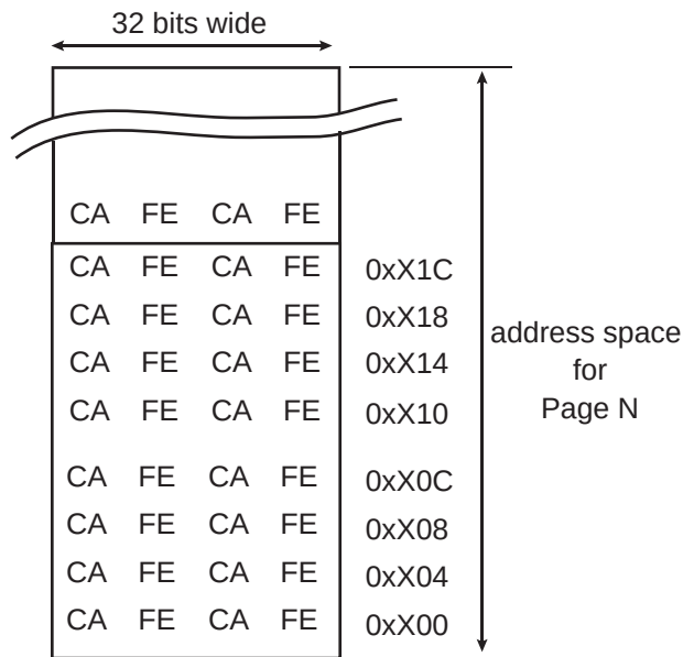
Figure 23-8. Full Page Programming
