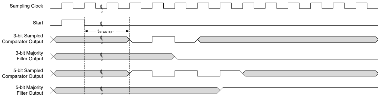
Figure 42-7. Single-Shot Filtering
