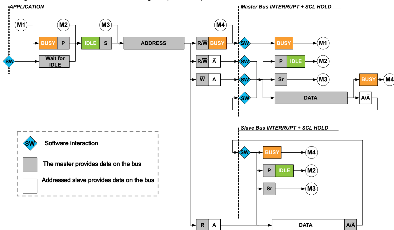
Figure 37-6. I 2 C Master Behavioral Diagram (SCLSM=1)
