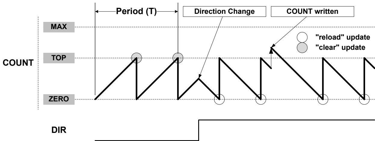
Figure 38-3. Counter Operation
