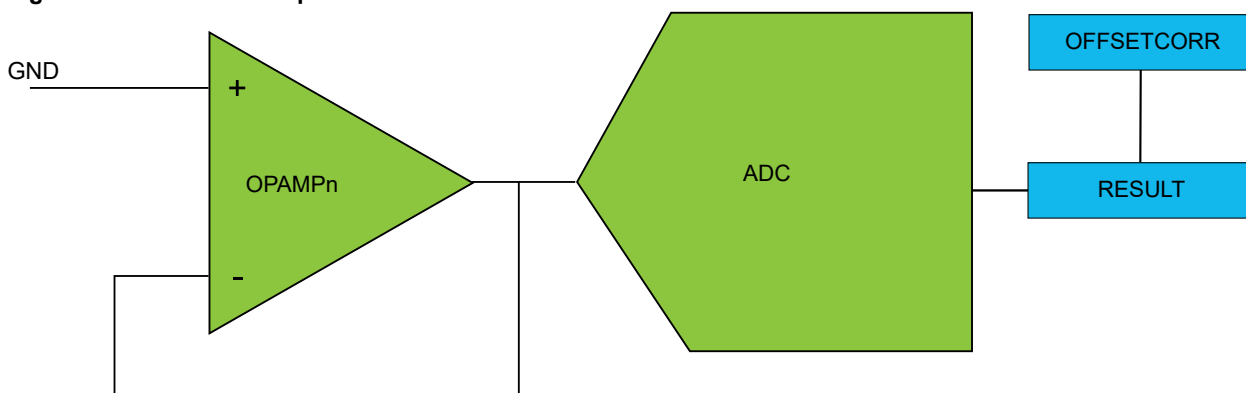
Figure 44-13. Offset Compensation
