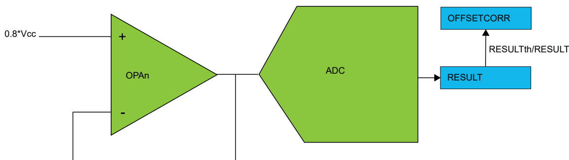
Figure 44-14. Gain Compensation
