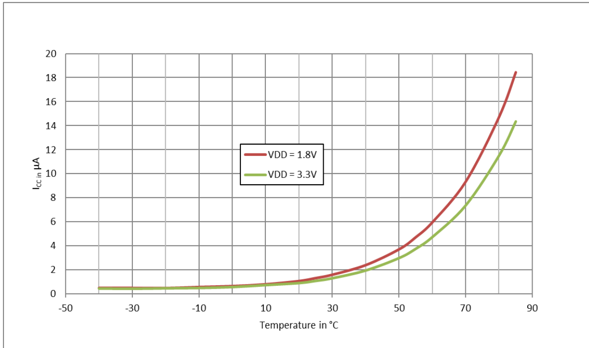
Figure 49-1. Power Consumption over Temperature in Standby Sleep Mode with PDSW in Active state
