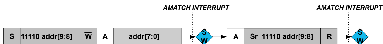
Figure 37-12. 10-bit Addressing
