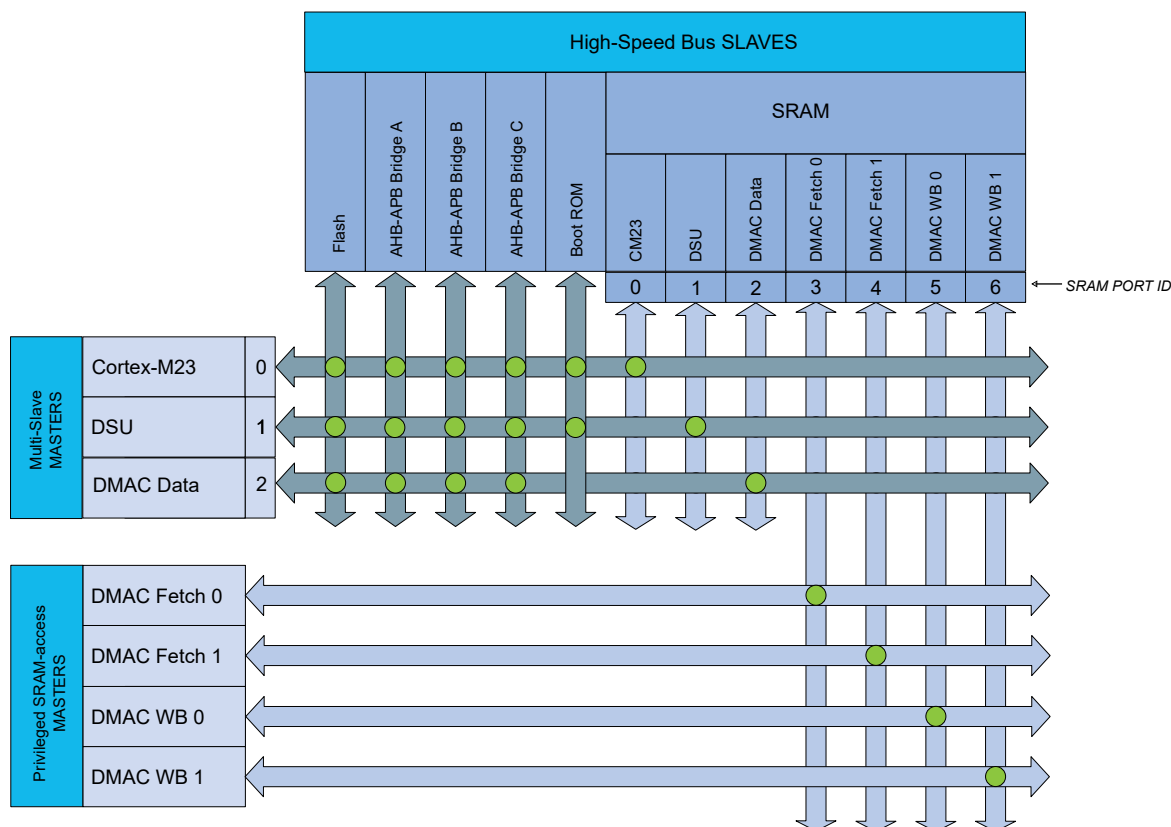
Figure 11-1. Master-to-Slave Access
