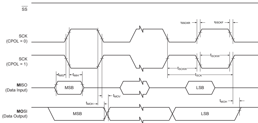
Figure 47-2. SPI Timing Requirements in Master Mode
