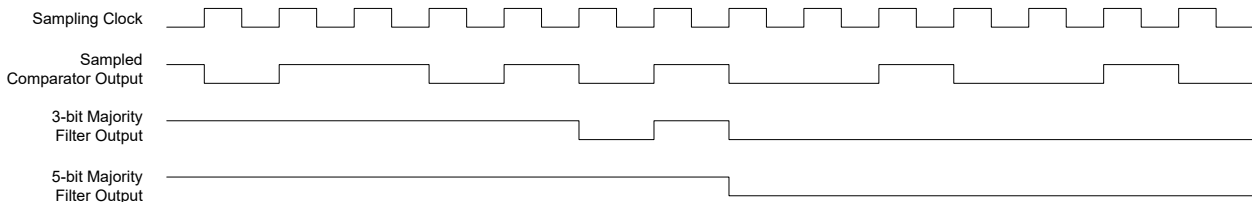
Figure 42-7. Single-Shot Filtering
