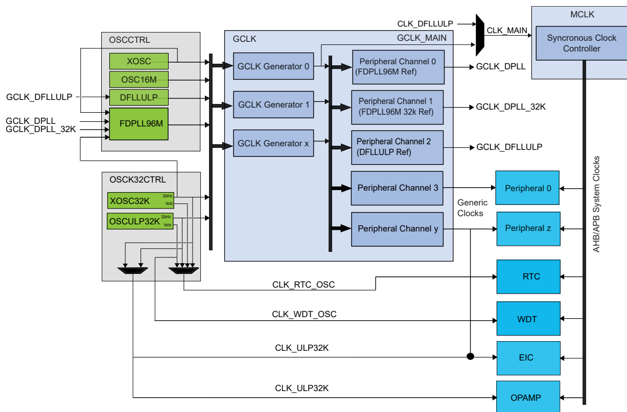
Figure 17-1. Clock Distribution
