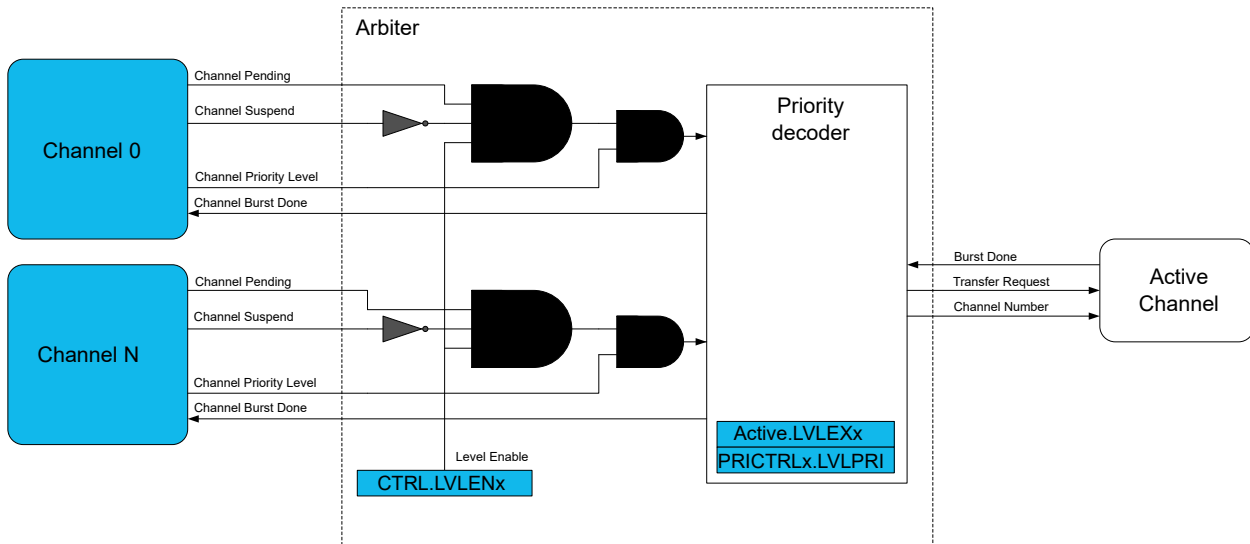
Figure 26-4. Arbiter Overview
