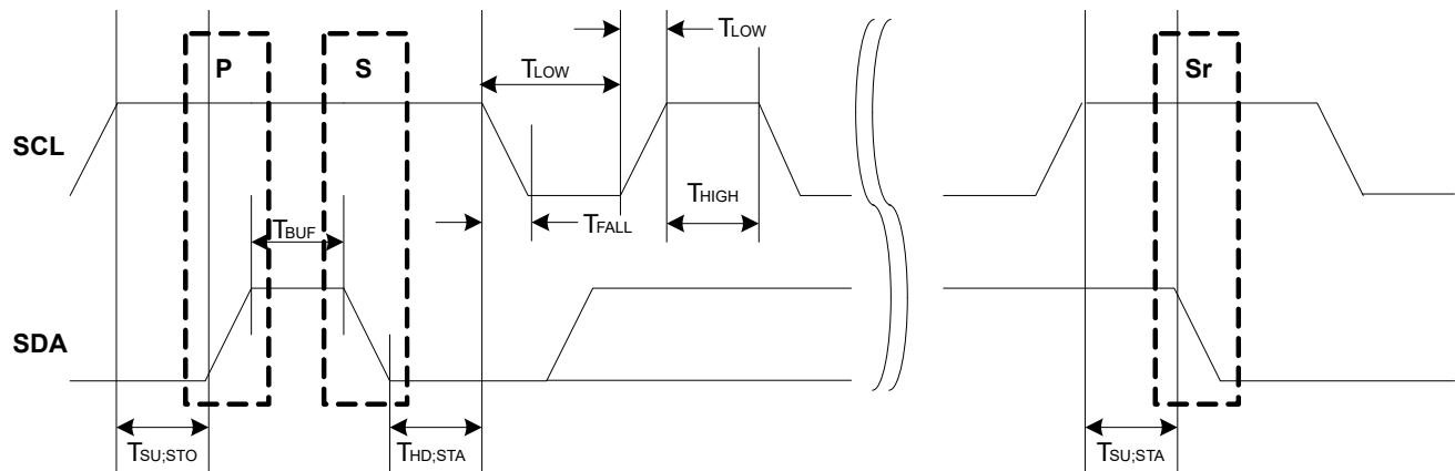
Figure 34-6. SCL Timing
