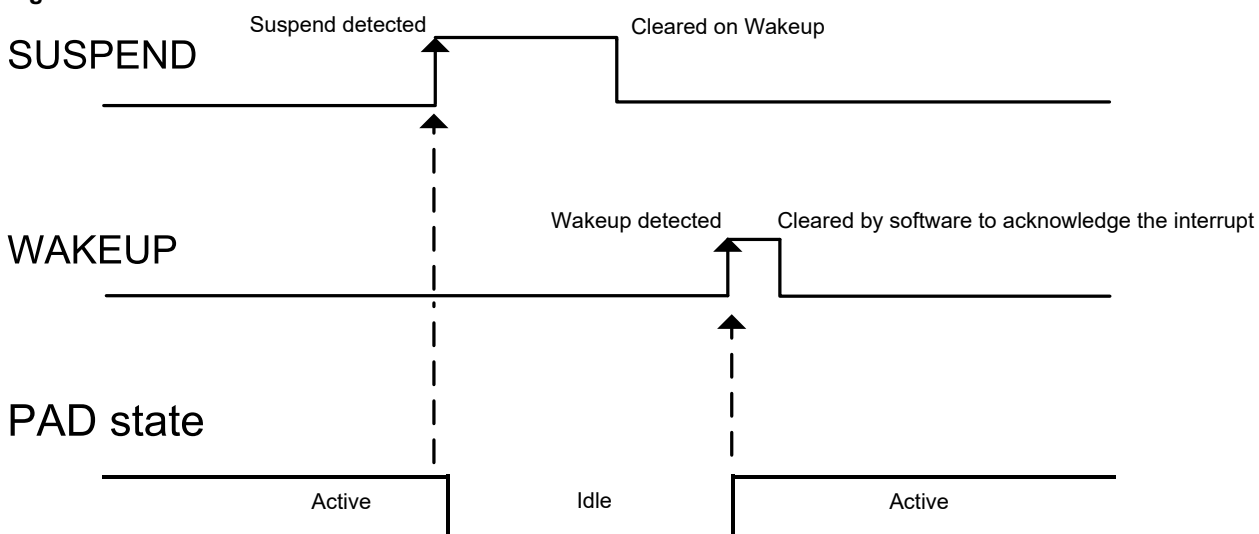
Figure 39-8. Pad Events
