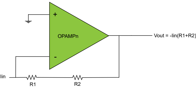
Figure 41-9. Transimpedance Amplifier
