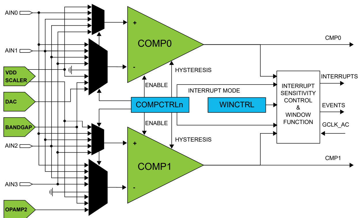
Figure 43-1. Analog Comparator Block Diagram
