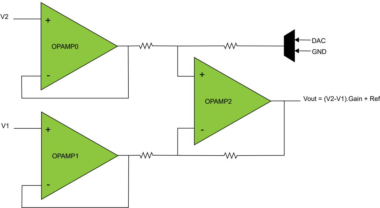
Figure 41-8. Instrumentation amplifier
