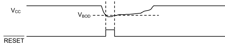
Figure 23-2. BOD Hysteresis Principle
