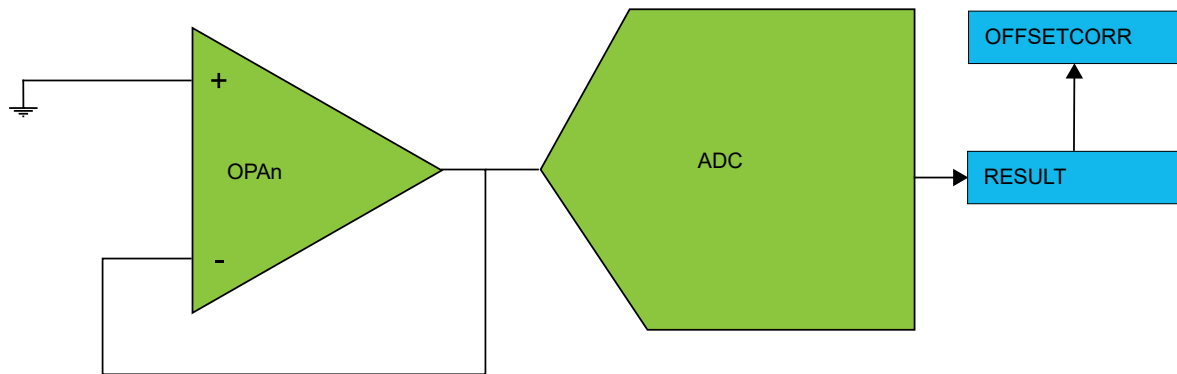
Figure 41-12. Offset Compensation
