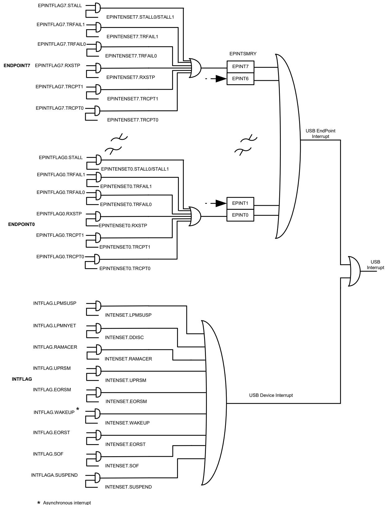
Figure 39-9. Device Interrupt
