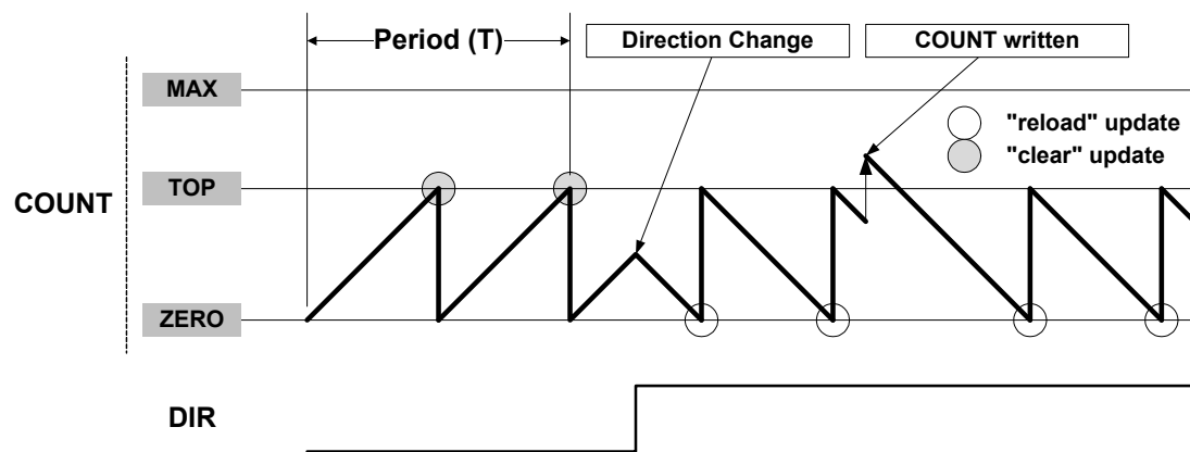
Figure 28-5. Counter Operation
