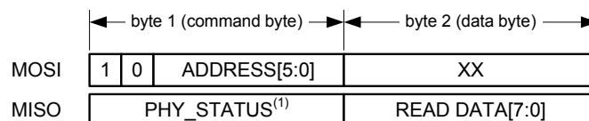
Figure 35-4. Packet Structure - Register Read Access
