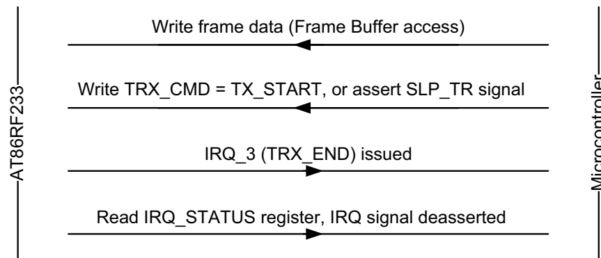
Figure 39-2. Transaction between AT86RF233 and Microcontroller during Transmit
