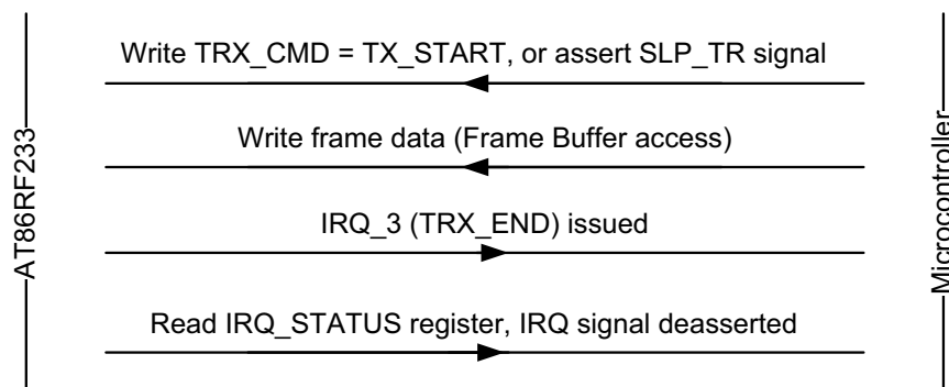
Figure 39-3. Time Optimized Frame Transmit Procedure.
