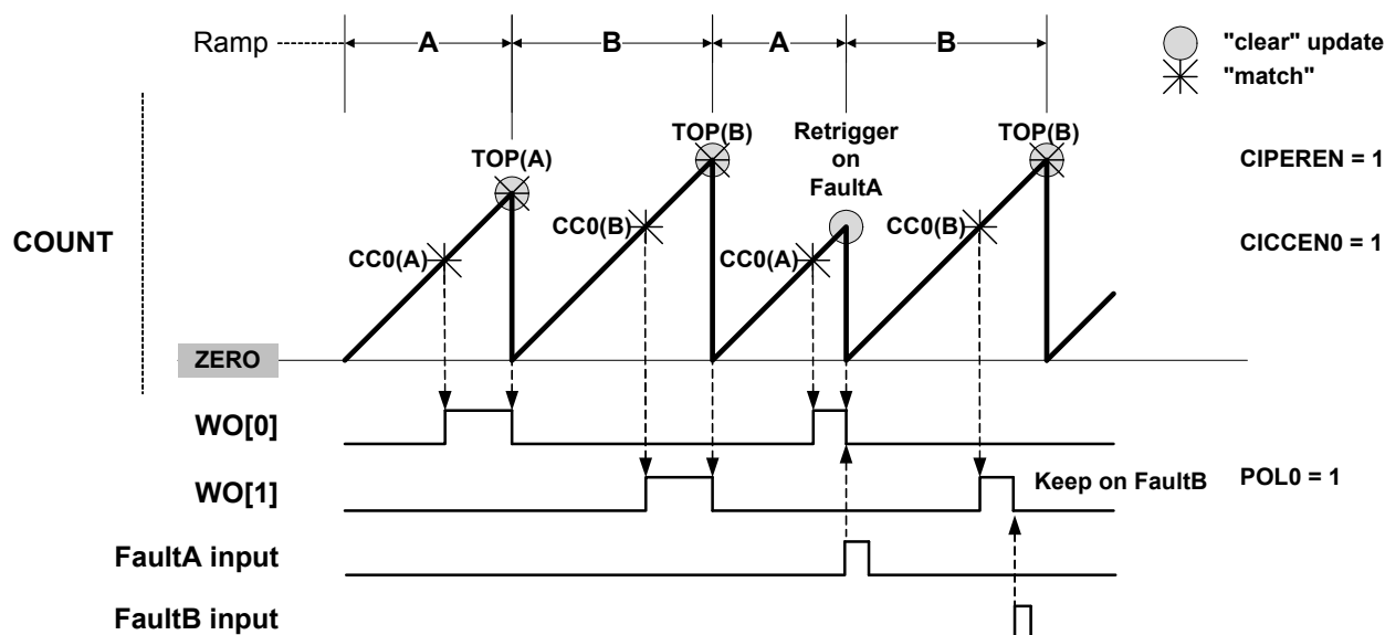
Figure 28-21.RAMP2 Alternate Operation
