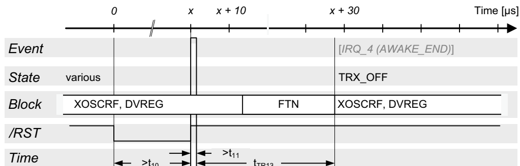
Figure 36-8. Reset Procedure
