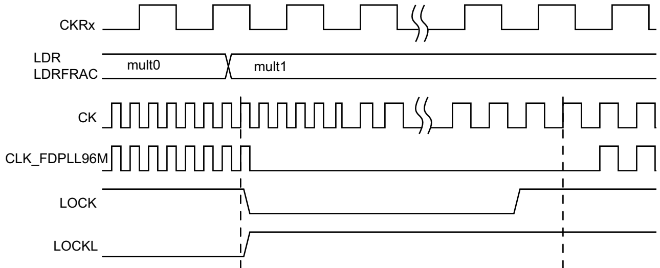
Figure 15-6. RATIOCTRL Register Update Operation
