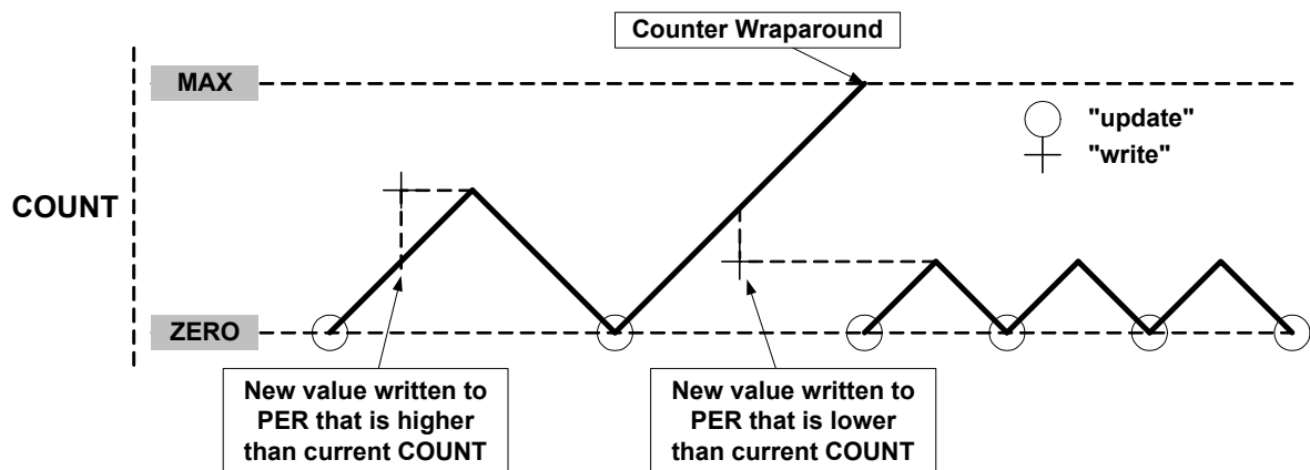
Figure 28-14.Unbuffered Dual-Slope Operation
