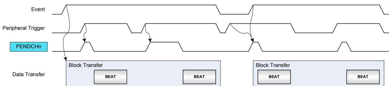
Figure 18-14. Conditional Block Transfer with Beat Peripheral Triggers
