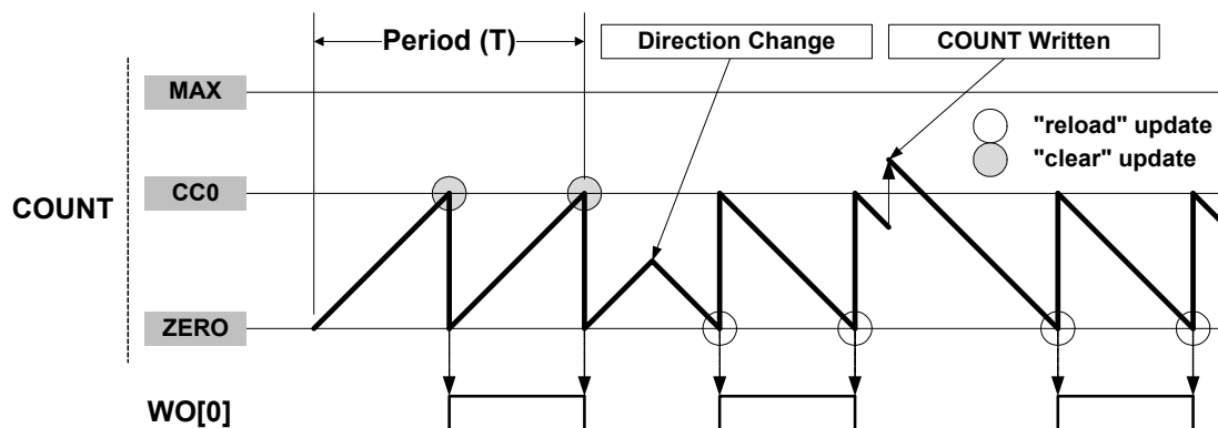
Figure 28-7. Match Frequency Operation
