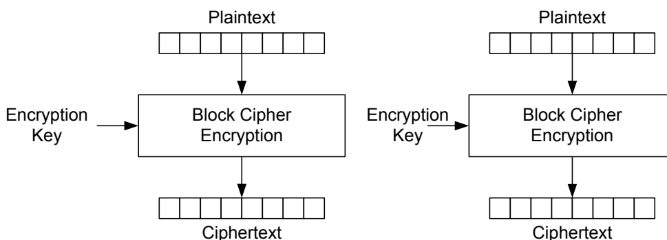
Figure 40-2. ECB Mode – Encryption
