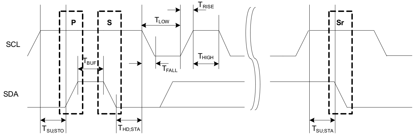
Figure 26-5. SCL Timing
