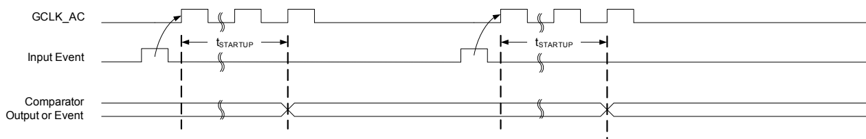
Figure 31-10. Single-Shot SleepWalking
