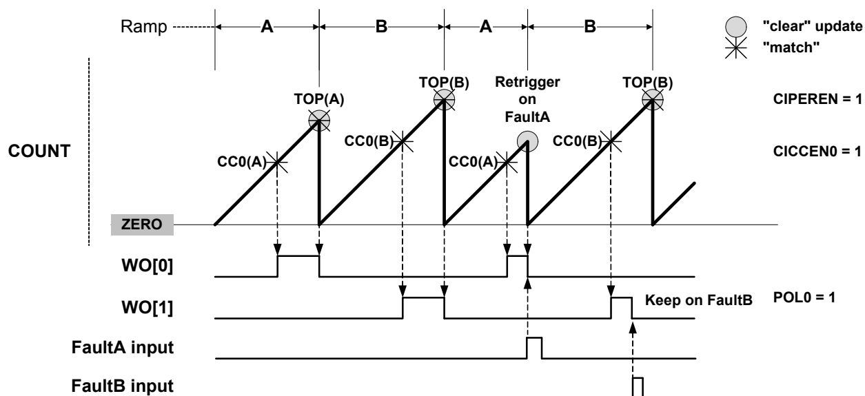
Figure 28-21.RAMP2 Alternate Operation
