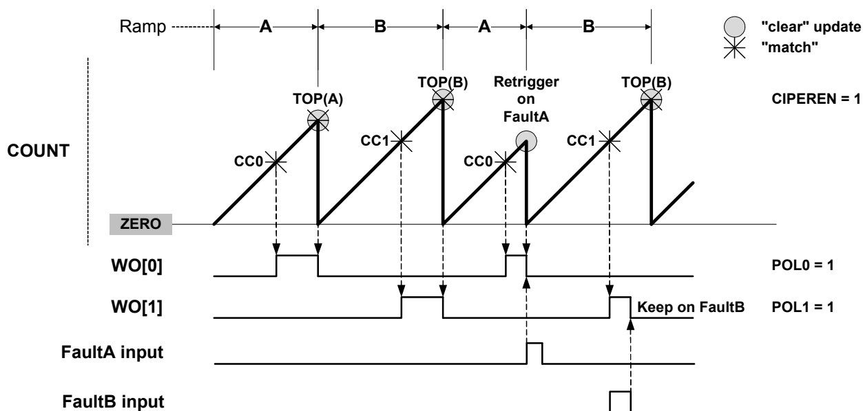
Figure 28-20.RAMP2 Standard Operation
