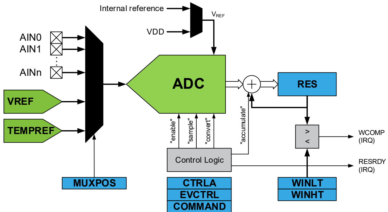
Figure 29-1. Block Diagram
