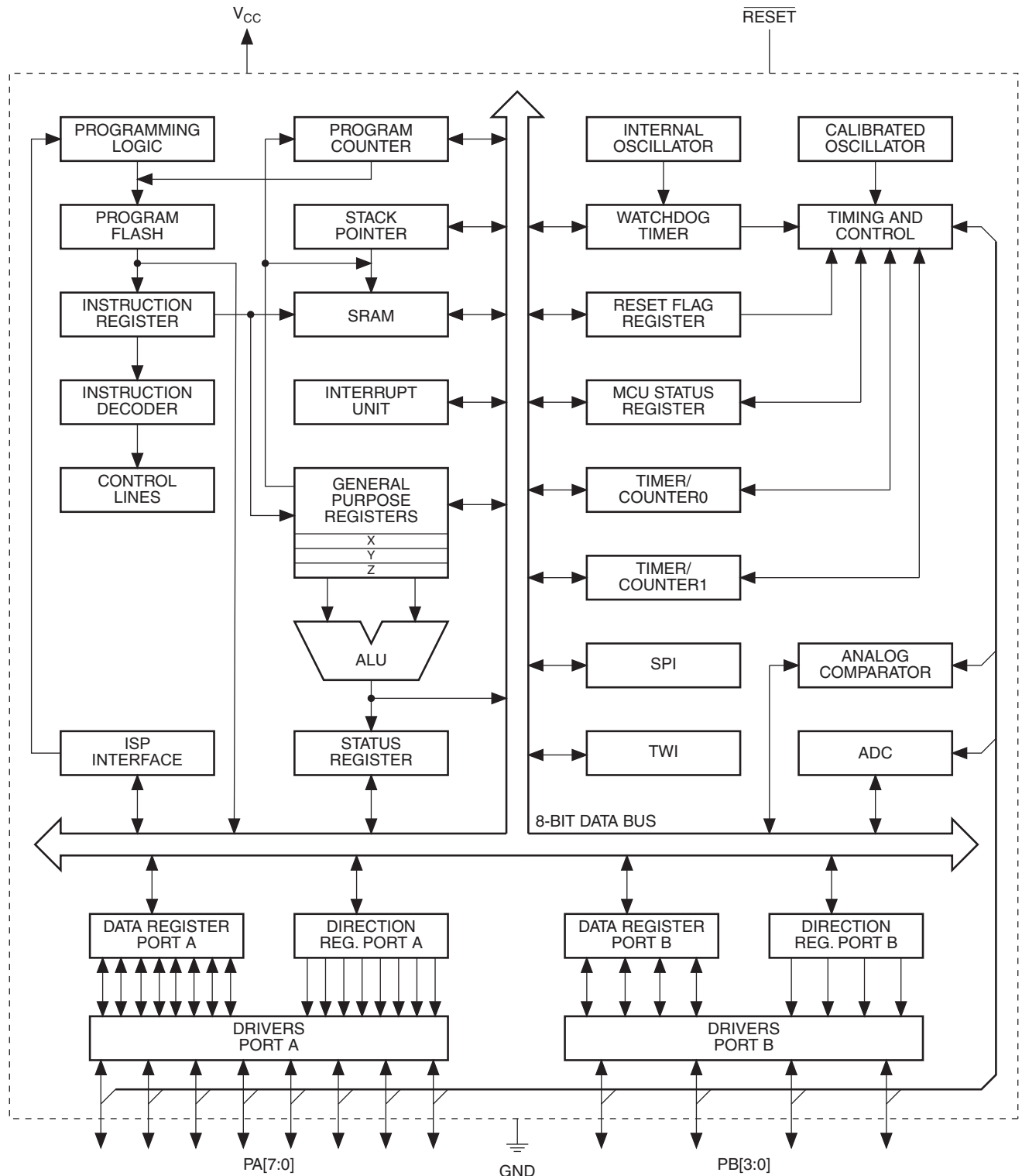
Figure 2-1. Block Diagram
