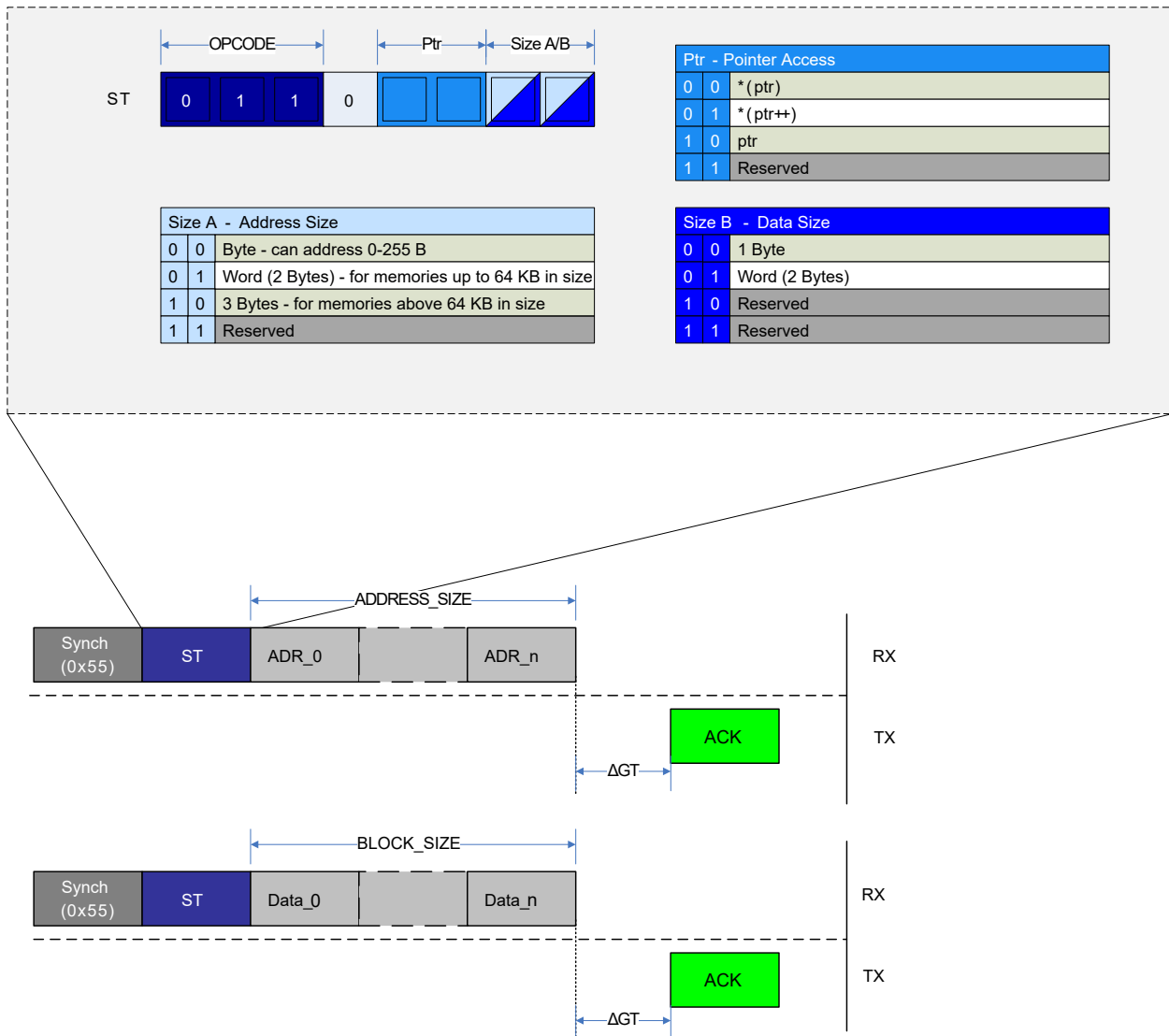
Figure 32-11. ST Instruction Operation
