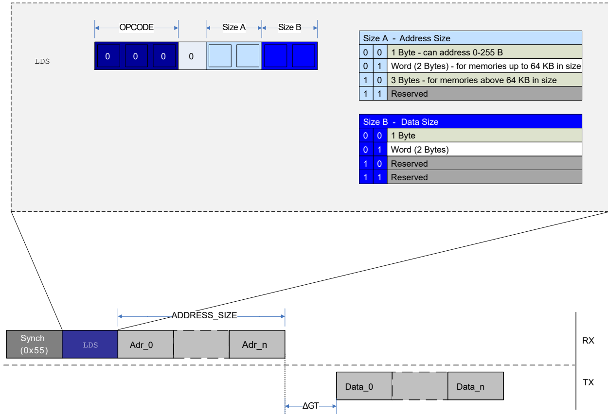
Figure 32-8. LDS Instruction Operation
