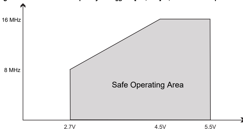
Figure 35-2. Maximum Frequency vs. V_{DD} for [-40, 125]^{\circ}\text{C} , Extended Temperature Range
