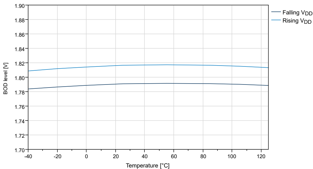
Figure 36-38. BOD Threshold vs. Temperature (Level 1.8V)
