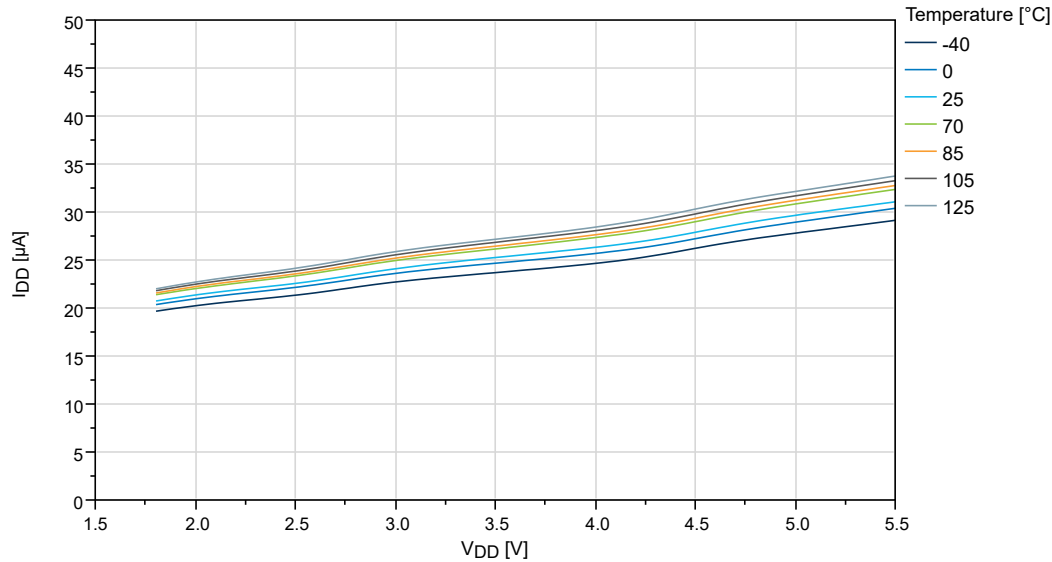
Figure 36-36. BOD Current vs. V_{DD} (Sampled BOD at 125 Hz)
