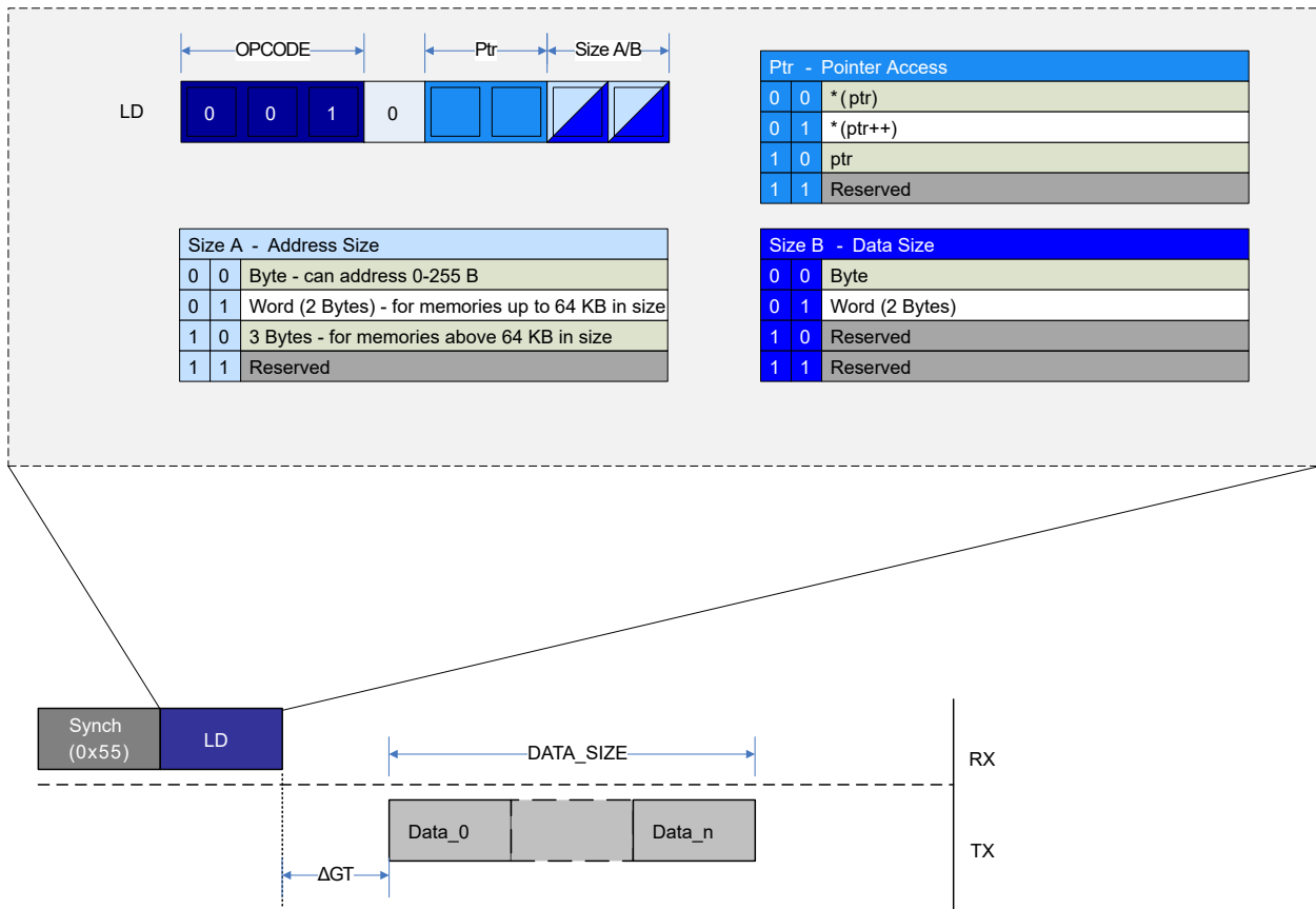
Figure 32-10. LD Instruction Operation
