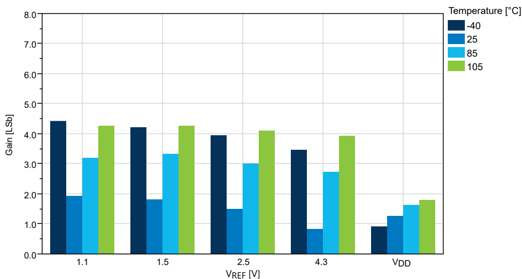
Figure 36-46. Gain Error vs. V_{REF} ( V_{DD} = 5.0\text{V} , f_{ADC} = 115 kps), REFSEL = Internal Reference
