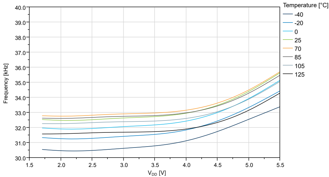
Figure 36-65. OSCULP32K Internal Oscillator Frequency vs. V_{DD}
