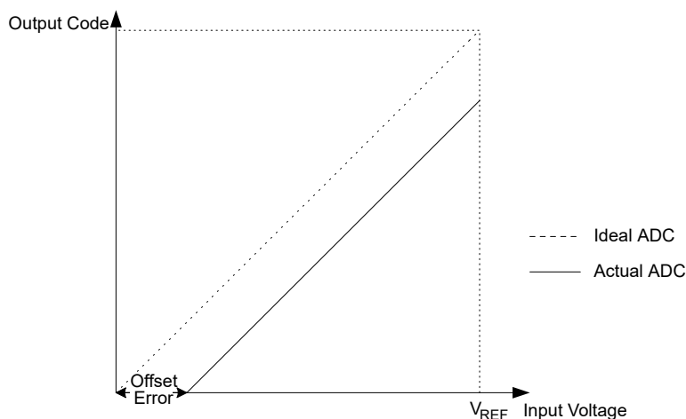
Figure 34-1. Offset Error
