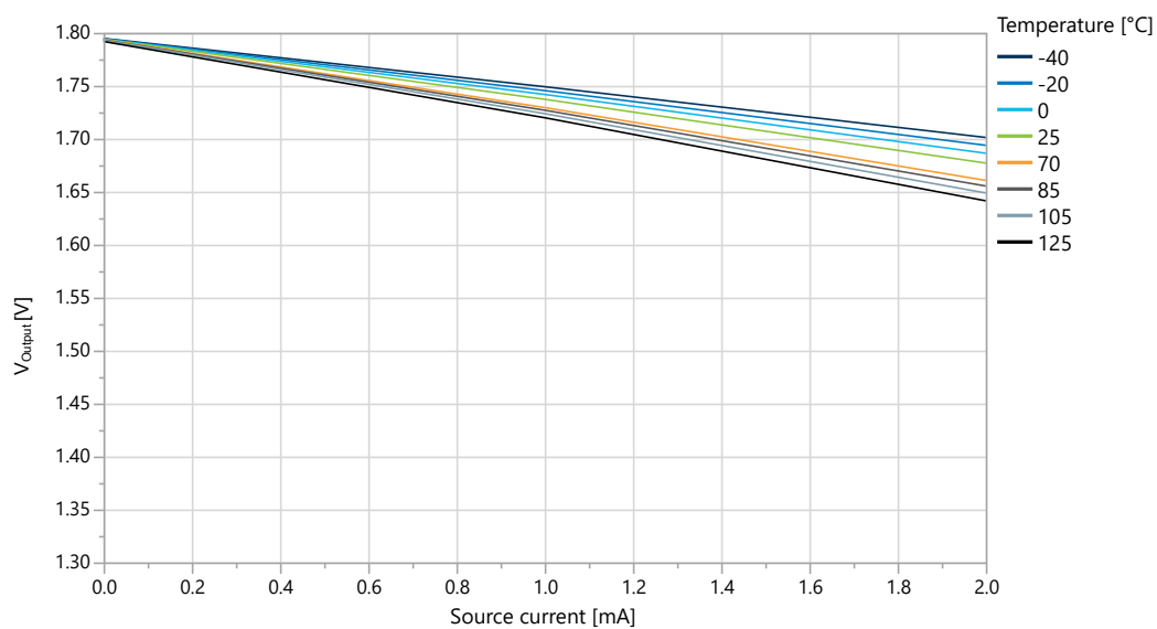
Figure 36-24. I/O Pin Output Voltage vs. Source Current ( V_{\text{DD}} = 1.8\text{V} )
