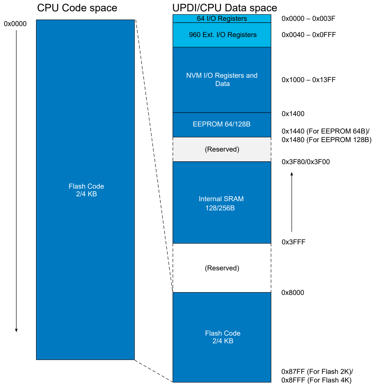
Figure 6-1. Memory Map
