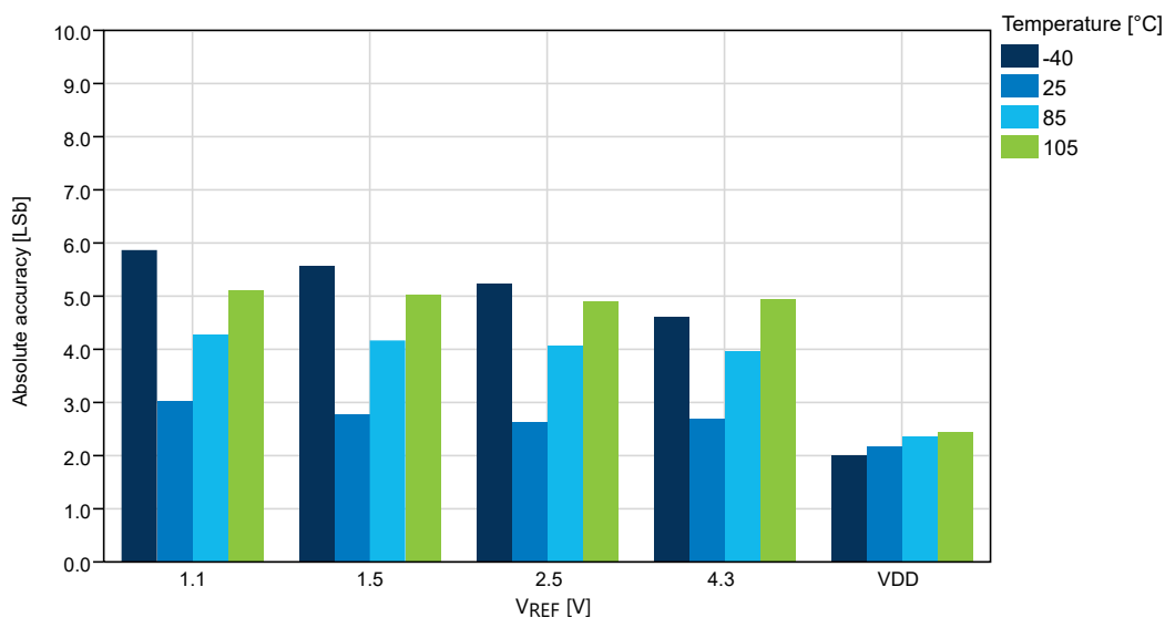
Figure 36-42. Absolute Accuracy vs. V_{REF} ( V_{DD} = 5.0\text{V} , f_{ADC} = 115 kps), REFSEL = Internal Reference
