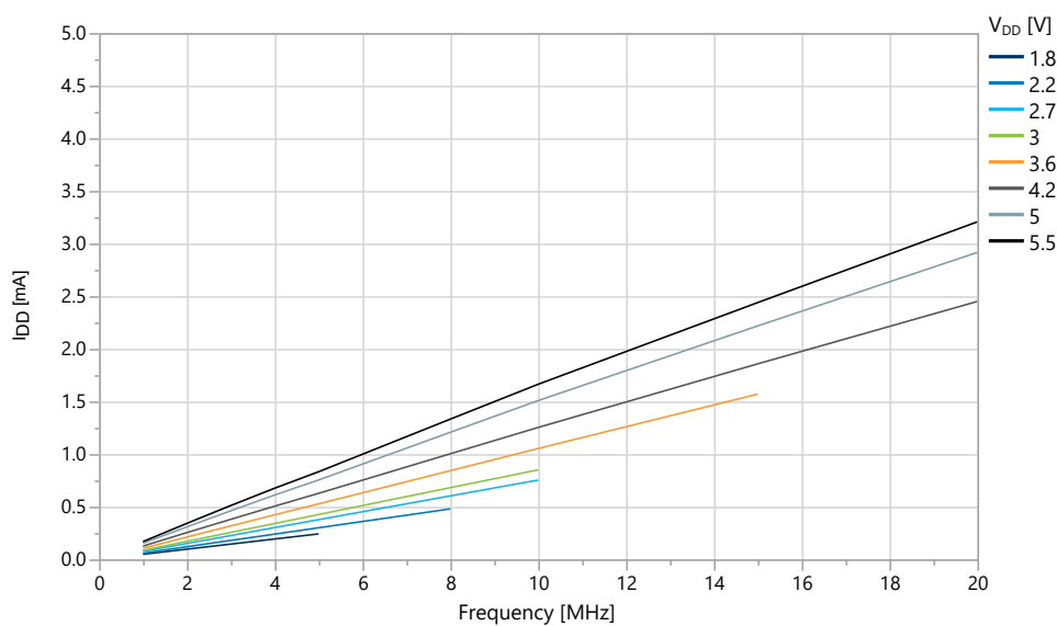
Figure 37-6. Idle Supply Current vs. Frequency (1-20 MHz) at T = 25^{\circ}C
