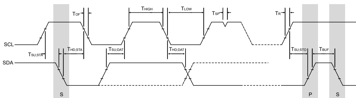
Figure 26-3. SCL Timing
