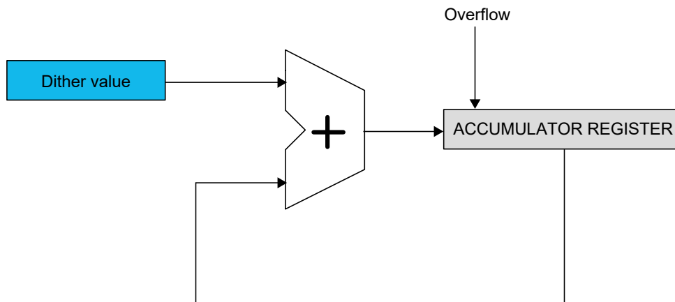
Figure 22-27. Dither Logic
