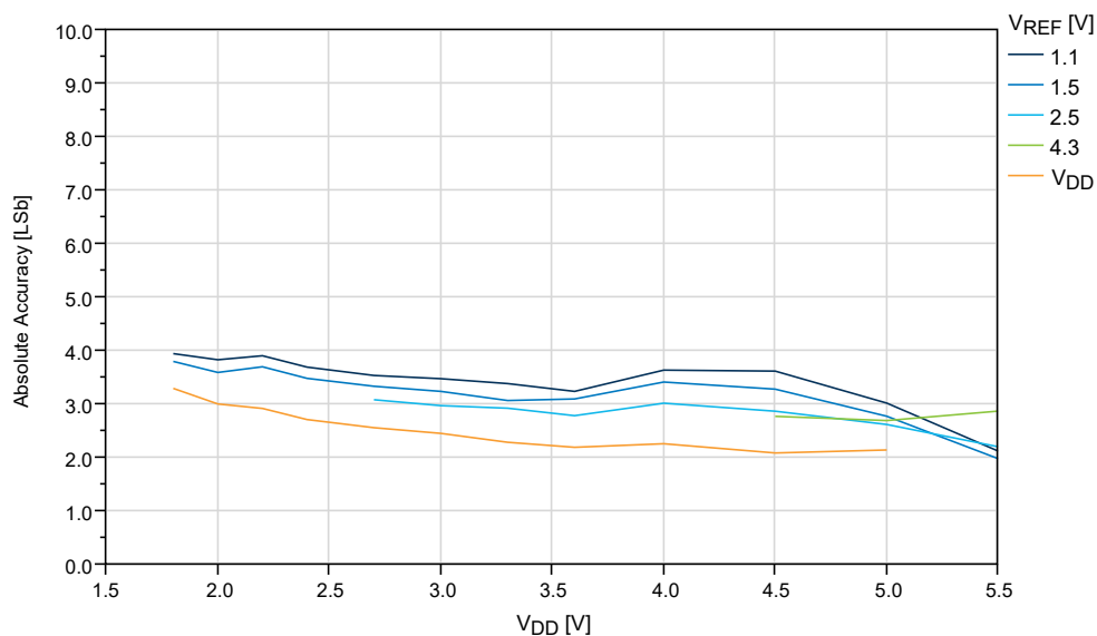
Figure 37-40. Absolute Accuracy vs. V_{DD} ( f_{ADC} = 115 kps) at T = 25^{\circ}\text{C} , REFSEL = Internal Reference
