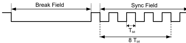
Figure 24-9. Auto-Baud Timing
