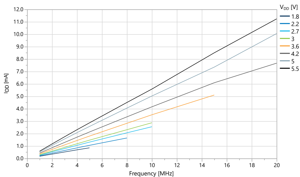
Figure 37-1. Active Supply Current vs. Frequency (1-20 MHz) at T = 25°C
