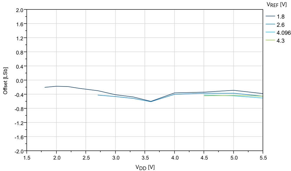
Figure 37-58. Offset vs. V_{DD} ( f_{ADC} = 115 ksp/s, T = 25^{\circ}C , REFSEL = External Reference)
