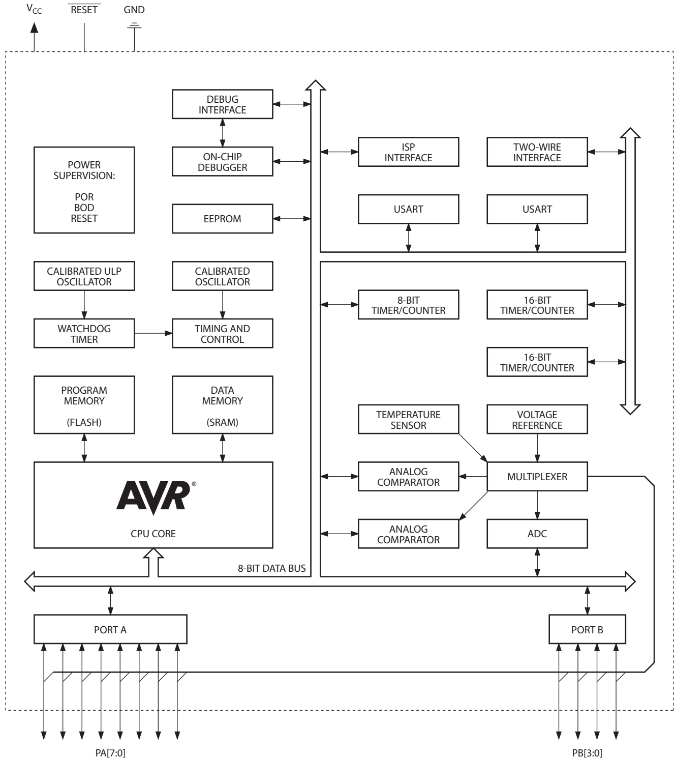
Figure 2-1. Block Diagram
