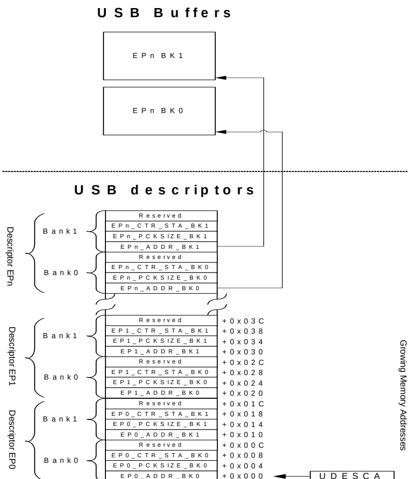
Figure 8-5. Memory organization
