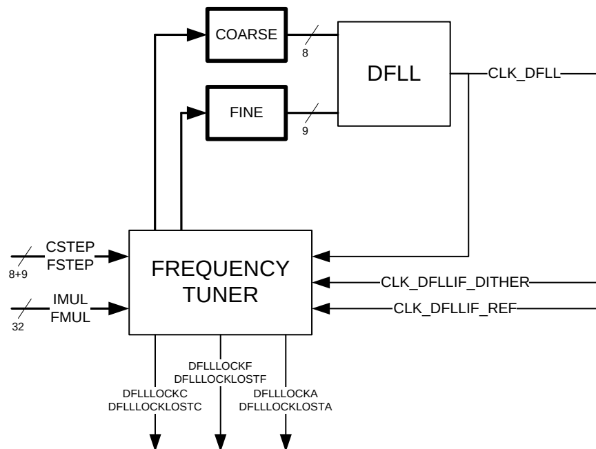
Figure 14-2. DFLLIF Block Diagram
