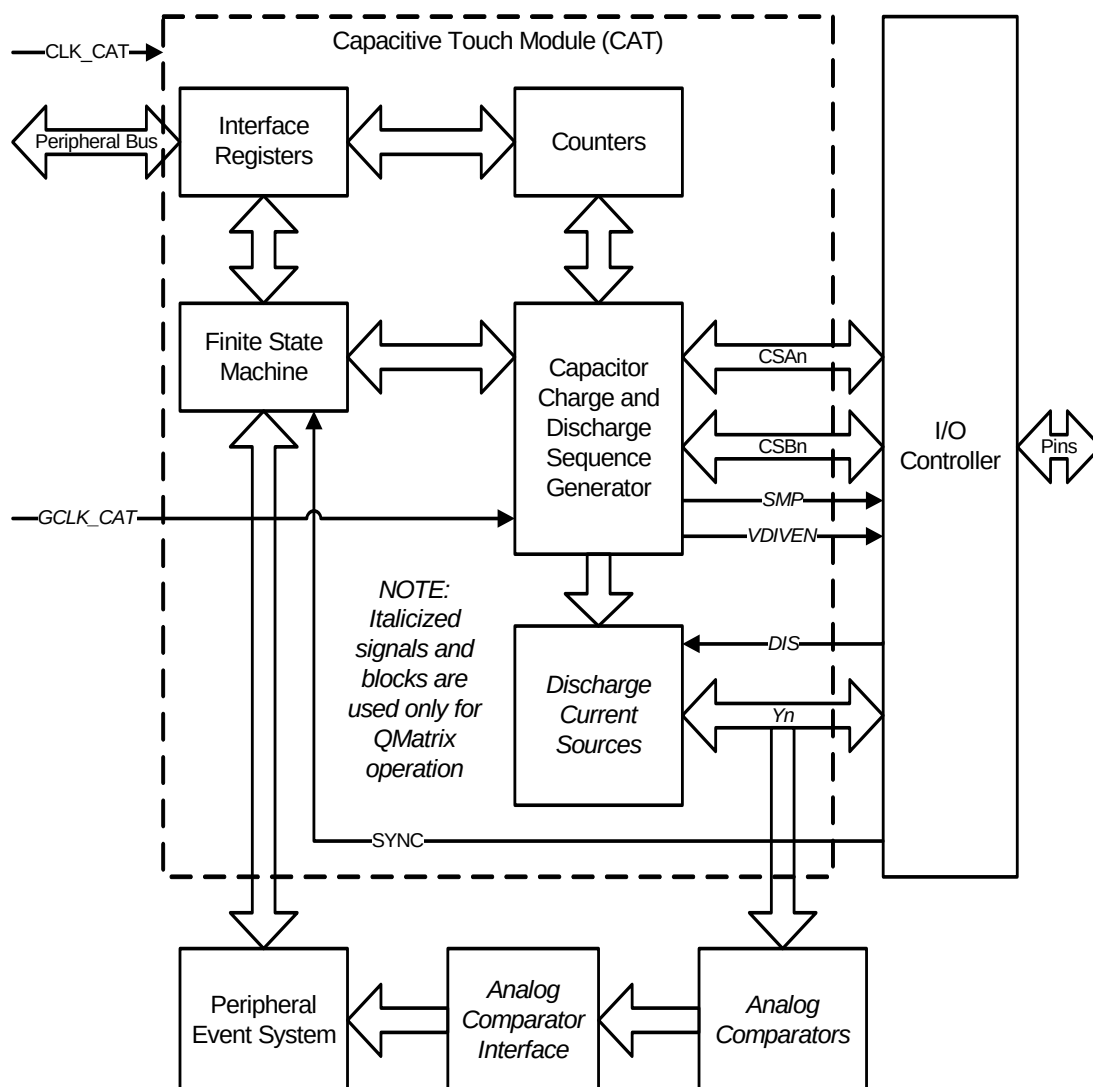
Figure 31-1. CAT Block Diagram
