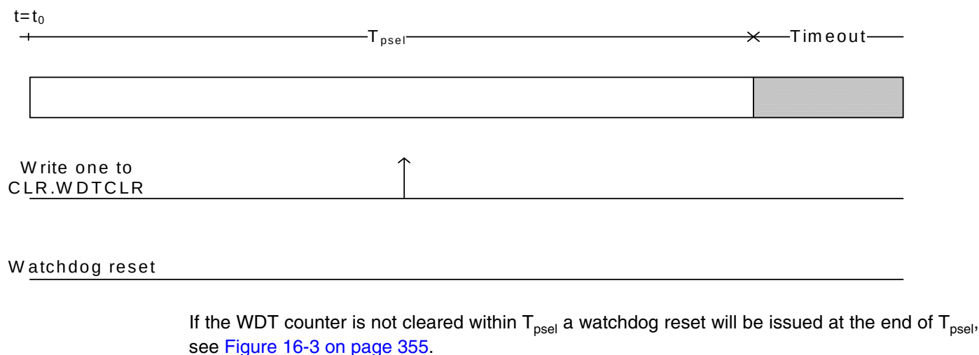
Figure 16-3. Basic Mode WDT Timing Diagram, no clear within T_{psel} .
