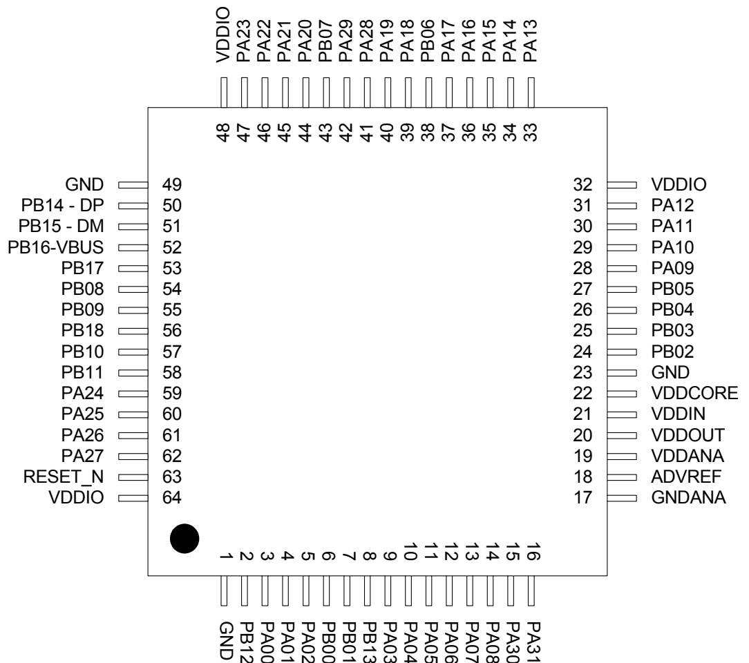
Figure 3-2. TQFP64/QFN64 Pinout
