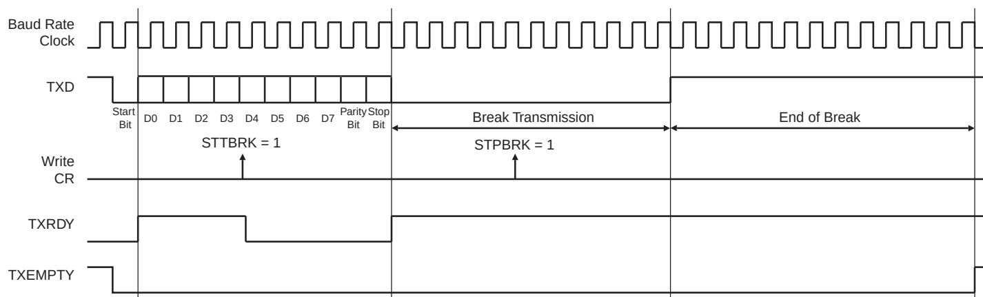
Figure 20-13. Break Transmission
