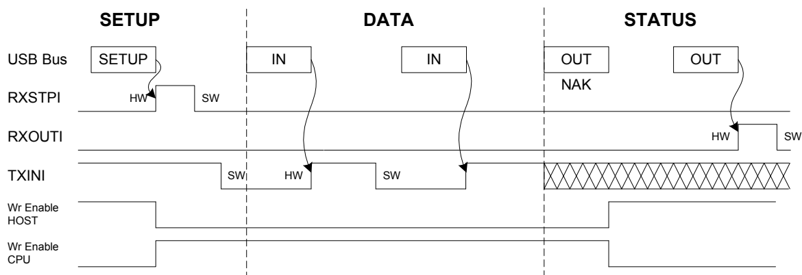
Figure 19-7. Control Read
