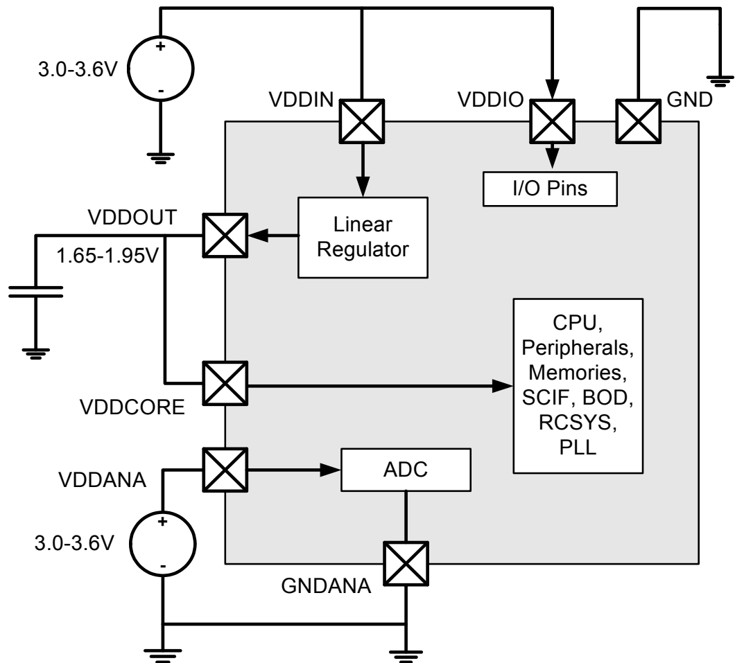
Figure 4-2. 3.3V Single Power Supply mode
