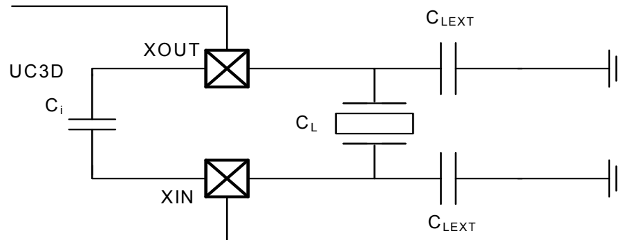
Figure 32-2. Oscillator Connection
