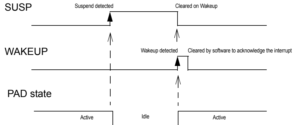
Figure 19-4. Pad events
