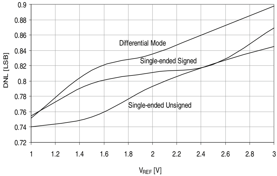
Figure 37-123. DNL error vs. external V_{REF}
