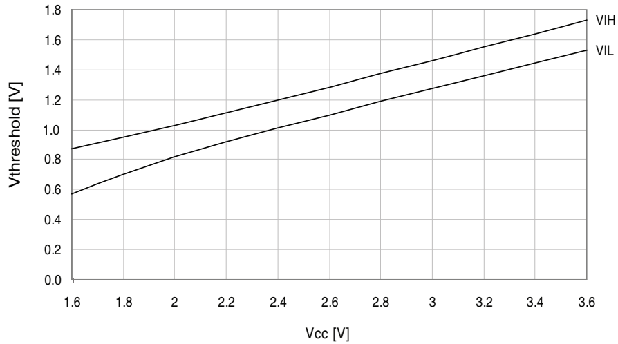
Figure 37-200. I/O pin input threshold voltage vs. V_{CC} . T = 25^{\circ}C .
