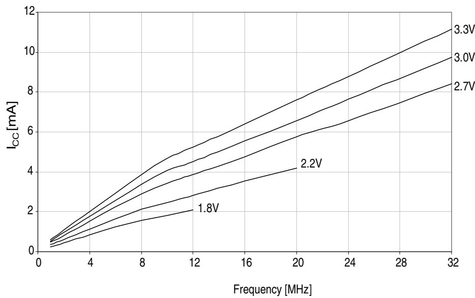
Figure 37-86. Active supply current vs. frequency.
