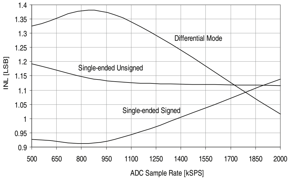
Figure 37-37. INL error vs. sample rate. T = 25°C, V_{CC} = 3.6V , V_{REF} = 3.0V external.
