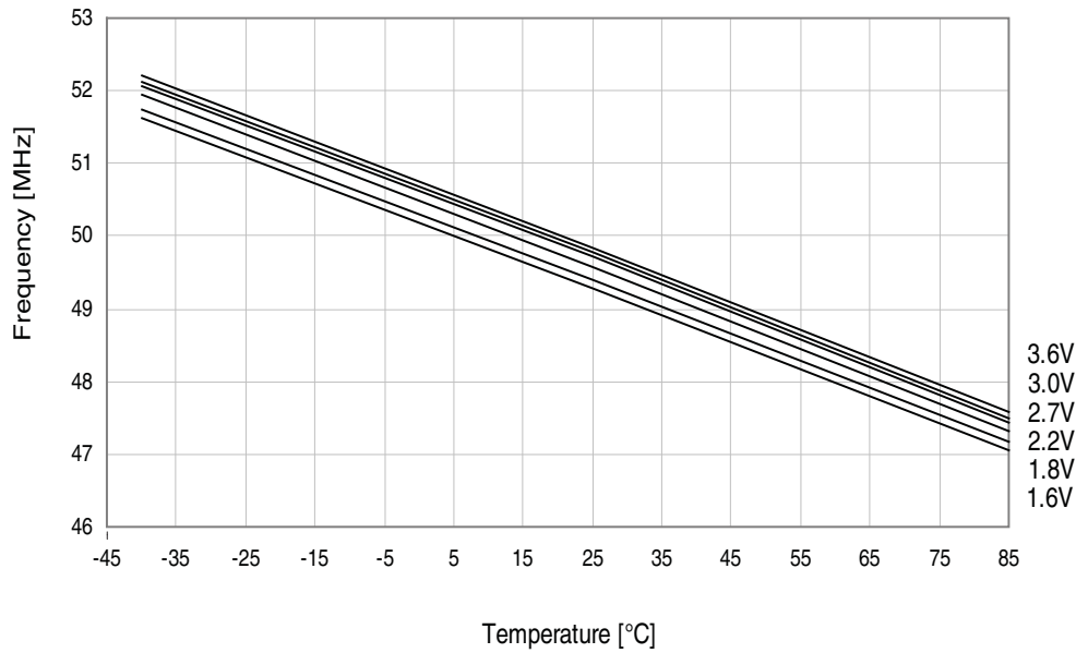
Figure 37-72. 48MHz internal oscillator frequency vs. temperature.
