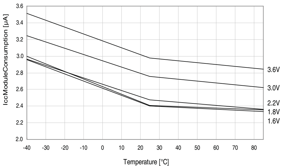
Figure 37-82. Psave LCD LP 32Hz vs. Temperature RTC, WDT, BOD sampled
