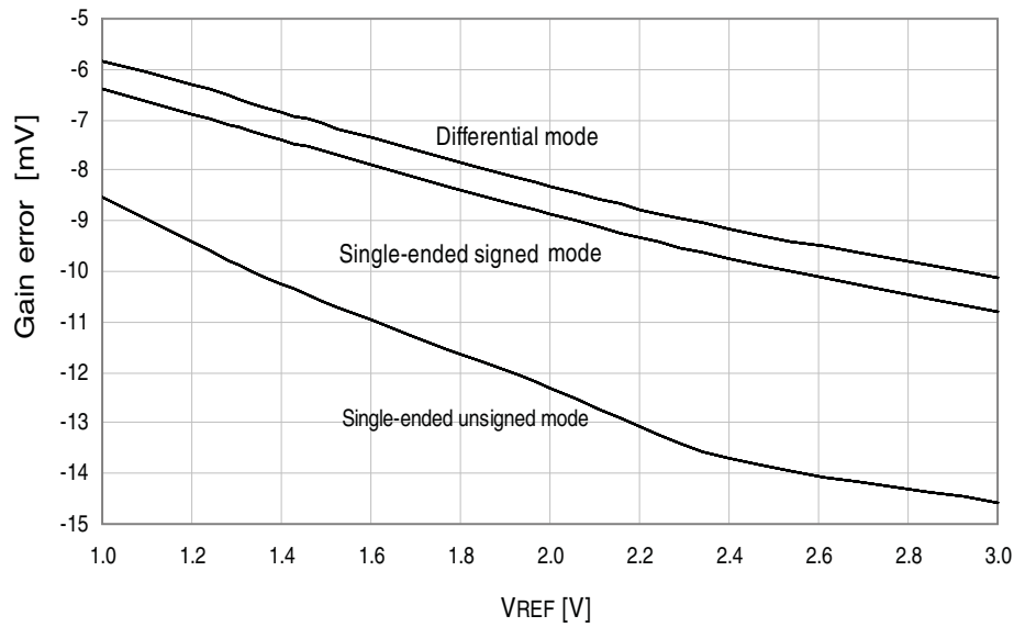
Figure 34-318. Gain Error vs. V_{REF} T = 25°C, V_{CC} = 3.6V , ADC sample rate = 300ksps
