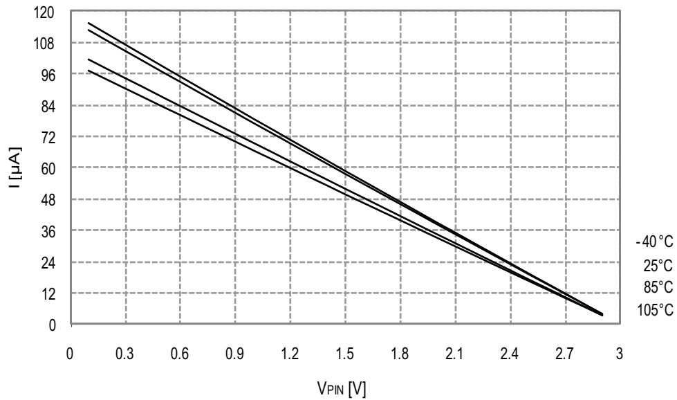
Figure 34-20. I/O Pin Pull-up Resistor Current vs. Input Voltage
