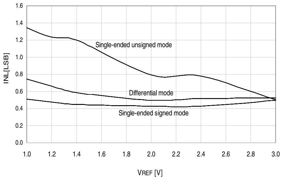
Figure 34-312. INL Error vs. External V_{REF} T = 25\text{ °C} , V_{CC} = 3.6\text{V} , external reference
