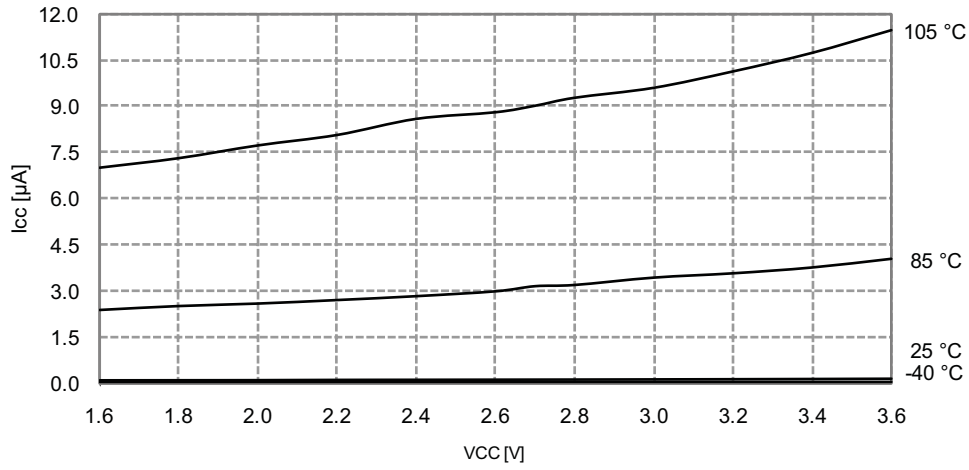
Figure 34-297. Power-down Mode Supply Current vs. V_{CC} All functions disabled
