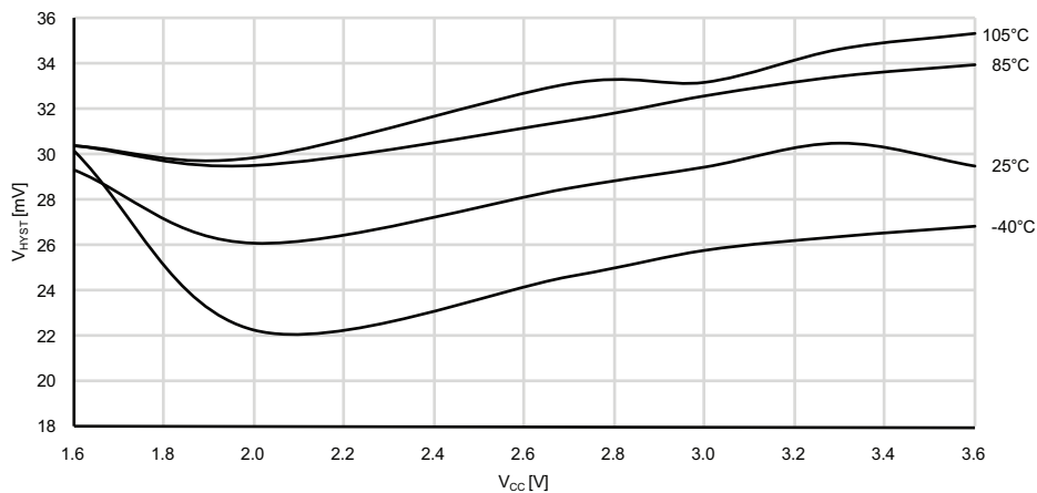
Figure 33-254. Analog Comparator Hysteresis vs. V_{CC}
