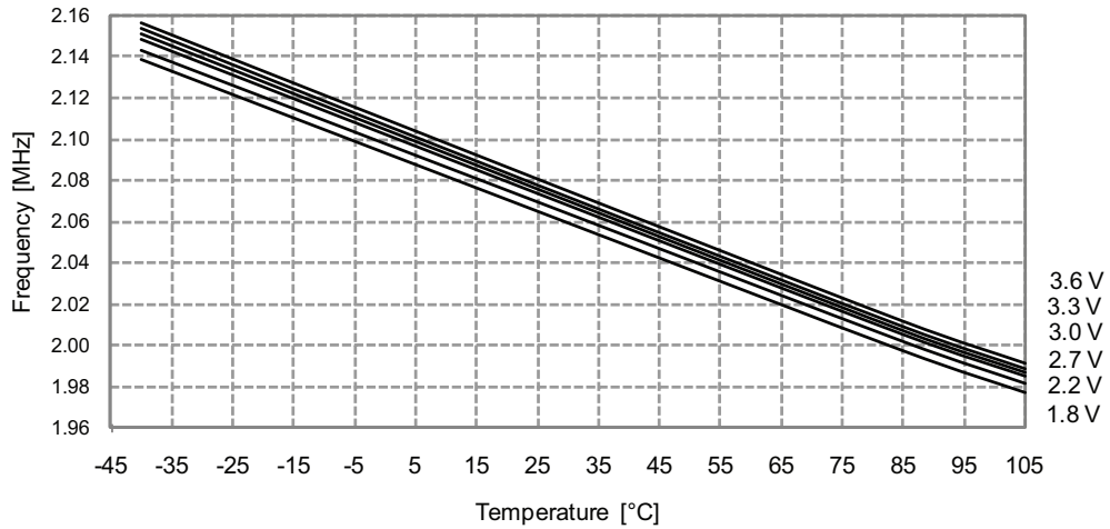
Figure 33-268. 2MHz Internal Oscillator Frequency vs. Temperature
