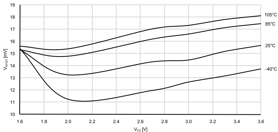
Figure 33-253. Analog Comparator Hysteresis vs. V_{CC}
