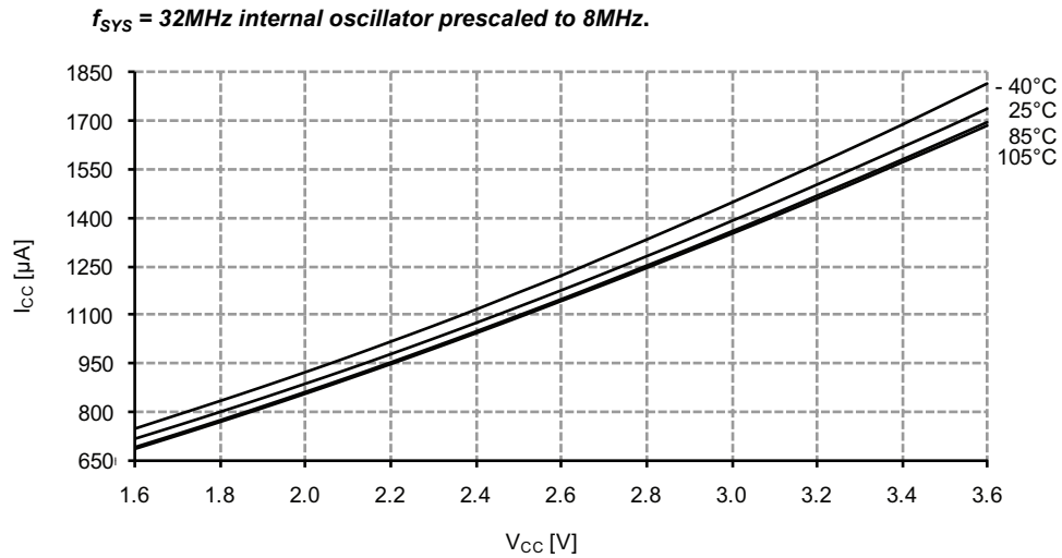
Figure 37-181. Idle mode supply current vs. V_{CC} .
