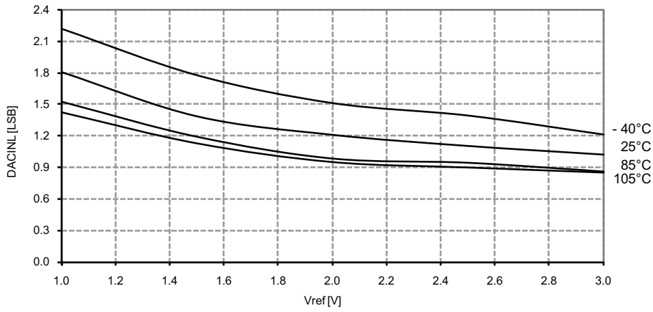
Figure 37-217. DAC INL error vs. V_{REF} . V_{CC} = 3.6V.
