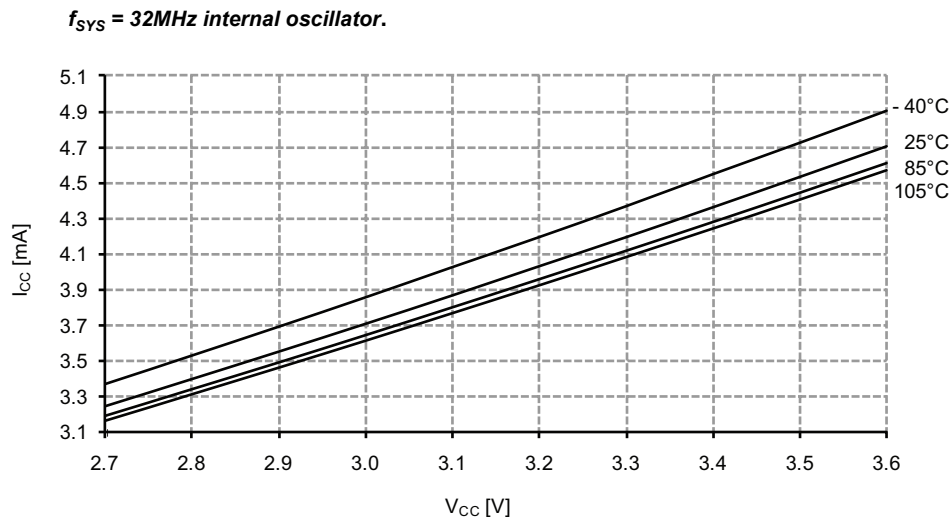
Figure 37-182. Idle mode current vs. V_{CC} .
