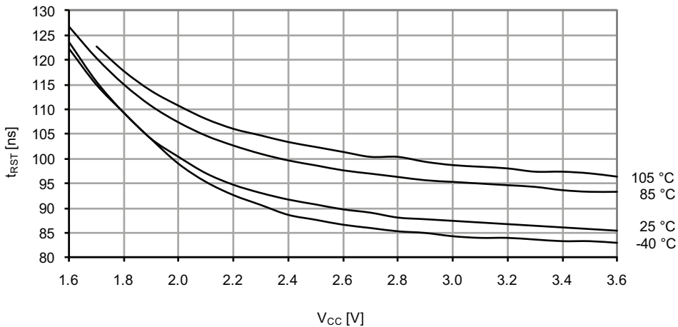
Figure 37-62. Minimum Reset pin pulse width vs. V CC .
