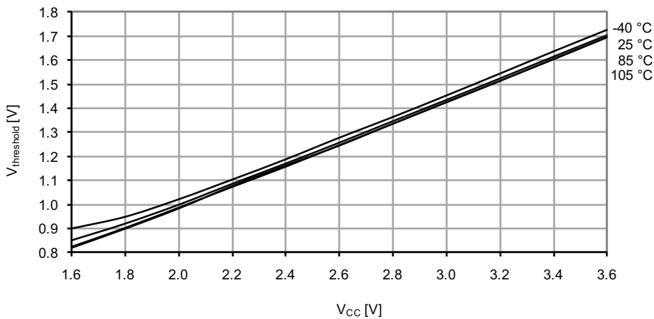
Figure 37-117. I/O pin input threshold voltage vs. V_{CC} . V_{\text{IH}} I/O pin read as "1".
