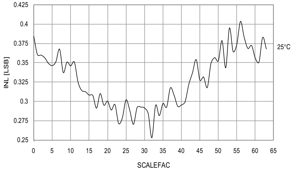
Figure 34-45. Voltage Scaler INL vs. SCALEFAC
