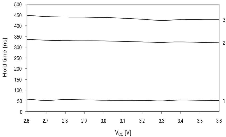
Figure 34-70. SDA Hold Time vs. Supply Voltage
