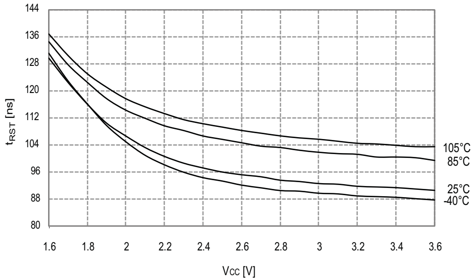
Figure 34-120. Minimum Reset Pin Pulse Width vs. V_{CC}
