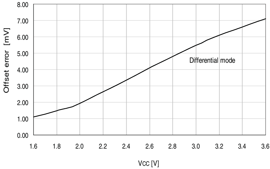
Figure 34-112. Offset Error vs. V_{CC} T = 25°C, V_{REF} = external 1.0V, ADC sample rate = 300ksps
