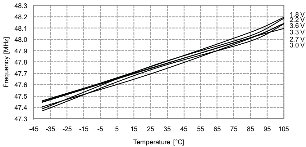
Figure 34-349. 48MHz Internal Oscillator Frequency vs. Temperature DPLL enabled, from the 32.768kHz internal oscillator
