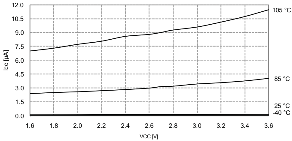
Figure 34-227. Power-down Mode Supply Current vs. V CC All functions disabled
