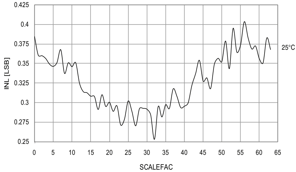
Figure 33-45. Voltage Scaler INL vs. SCALEFAC
