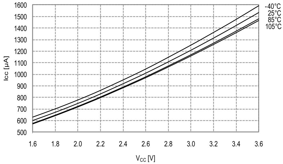
Figure 33-84. Idle Mode Supply Current vs. V_{CC}
