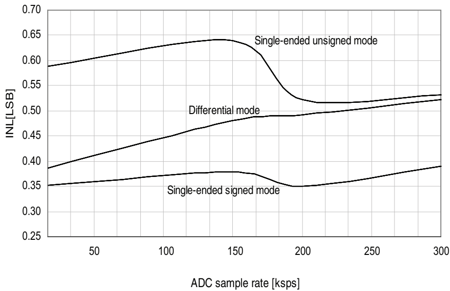
Figure 33-32. INL Error vs. Sample Rate T = 25°C, V_{CC} = 3.6V , V_{REF} = 3.0V external
