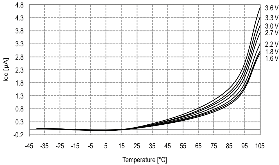
Figure 33-88. Power-down Mode Supply Current vs. Temperature All functions disabled
