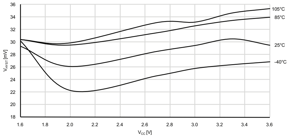
Figure 33-254. Analog Comparator Hysteresis vs. V_{CC} Large hysteresis
