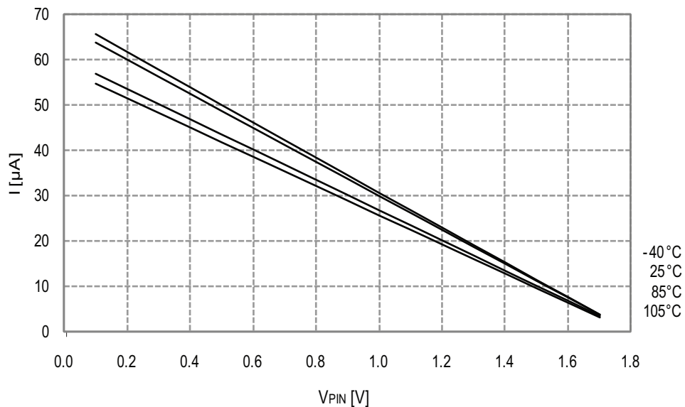
Figure 33-90. I/O Pin Pull-up Resistor Current vs. Input Voltage
