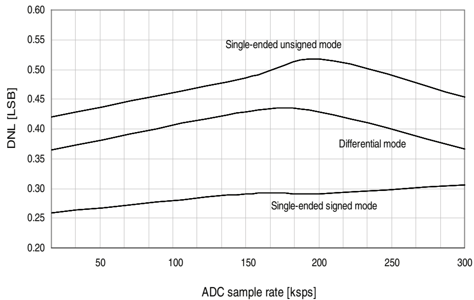
Figure 33-386. DNL Error vs. Sample Rate
