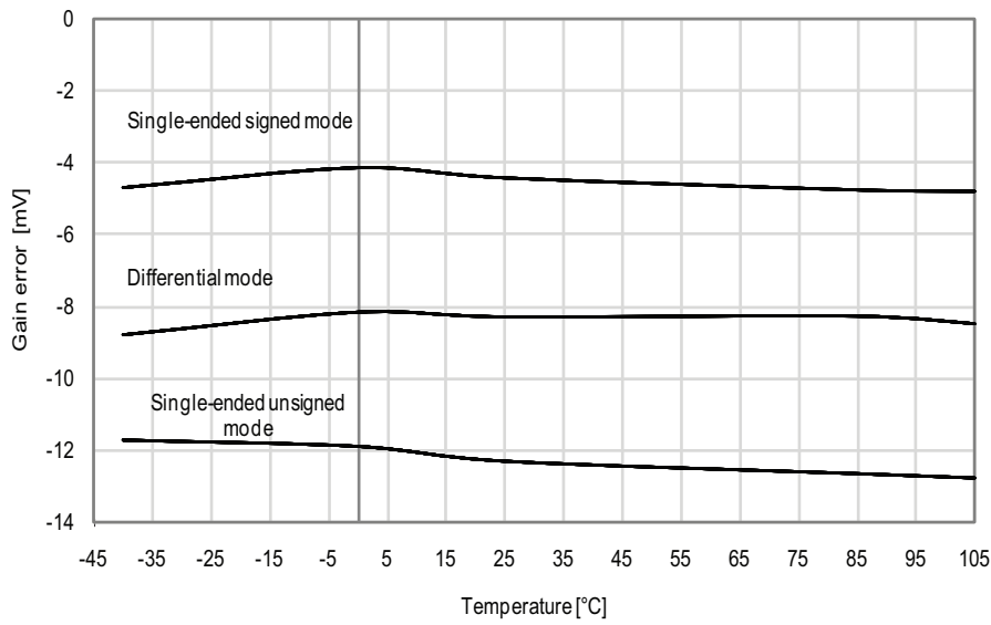
Figure 33-321. Gain Error vs. Temperature
