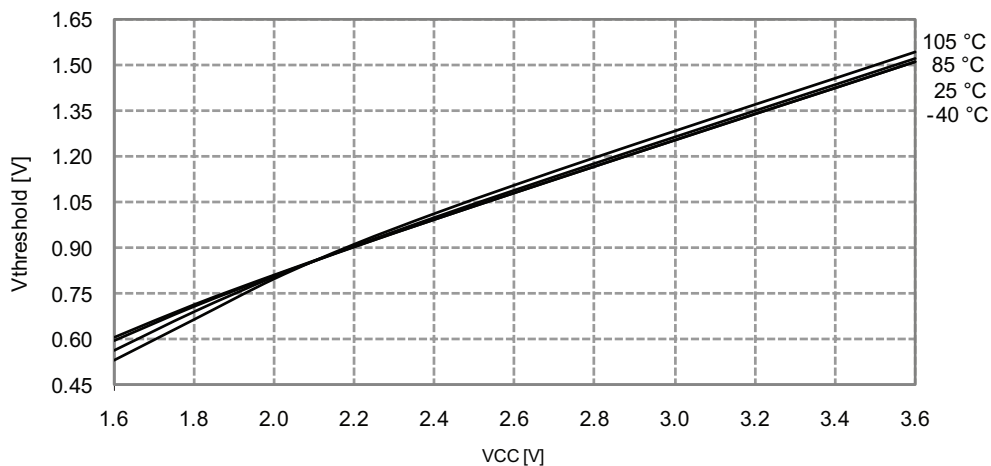
Figure 33-240.I/O Pin Input Threshold Voltage vs. V_{CC}
