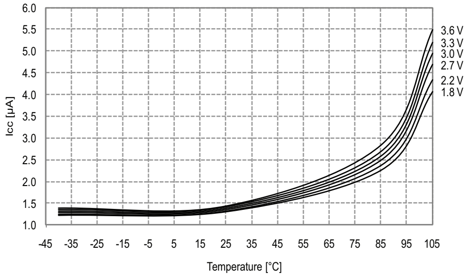
Figure 33-89. Power-down Mode Supply Current vs. Temperature Watchdog and sampled BOD enabled and running from internal ULP oscillator
