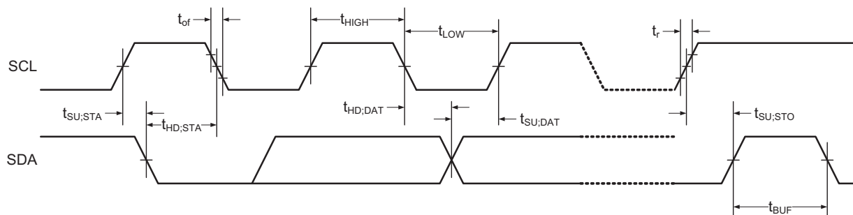
Figure 32-7. Two-wire Interface Bus Timing
