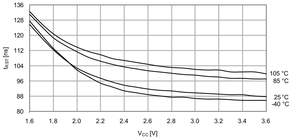
Figure 33-260. Minimum Reset Pin Pulse Width vs. V CC
