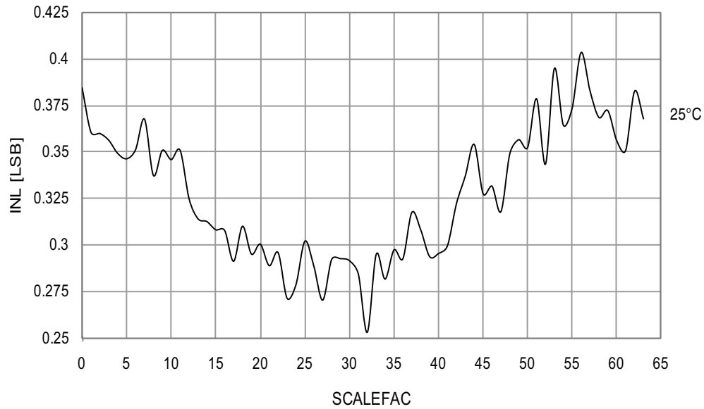
Figure 34-116. Voltage Scaler INL vs. SCALEFAC
