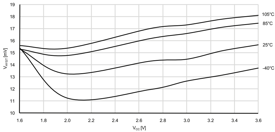
Figure 33-393. Analog Comparator Hysteresis vs. V_{CC} Small hysteresis
