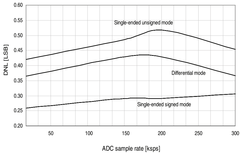
Figure 33-176. DNL Error vs. Sample Rate T = 25°C, V_{CC} = 3.6V , V_{REF} = 3.0V external
