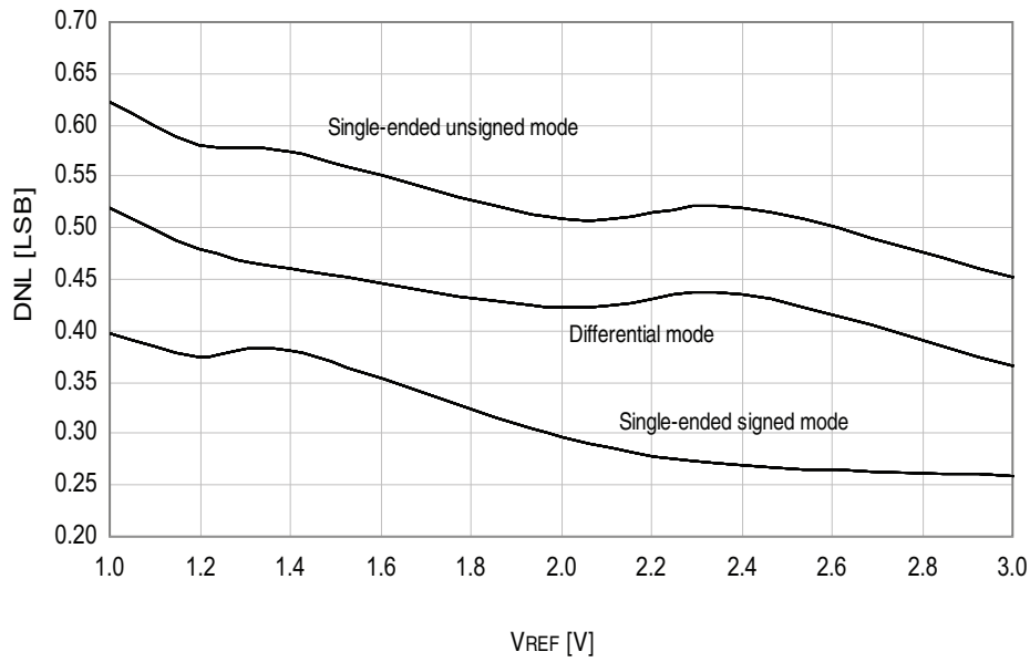
Figure 33-175. DNL Error vs. External V_{REF} T = 25°C, V_{CC} = 3.6V , external reference
