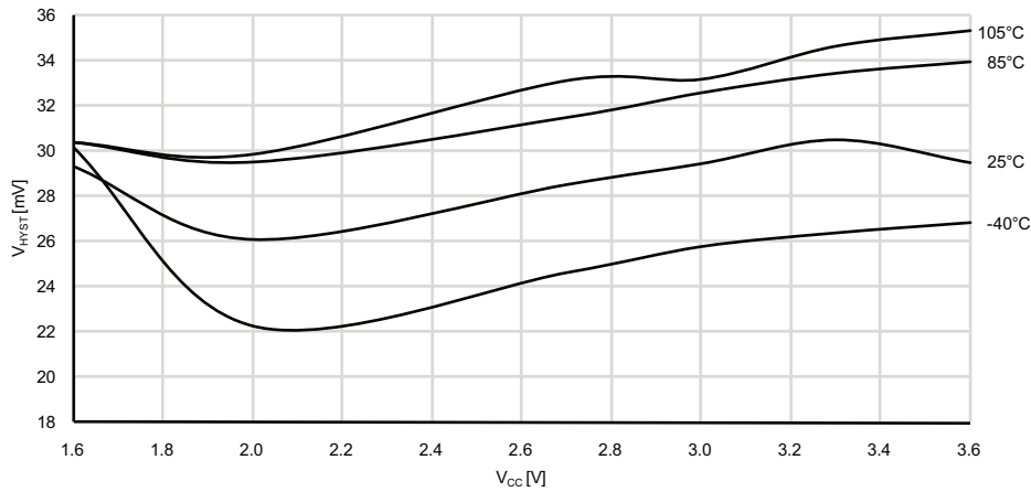
Figure 33-394. Analog Comparator Hysteresis vs. V_{CC} Large hysteresis
