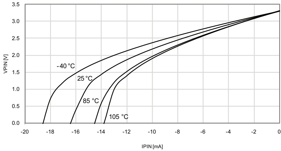
Figure 33-165. I/O Pin Output Voltage vs. Source Current
