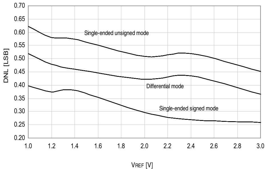
Figure 33-34. DNL Error vs. External V_{REF}
