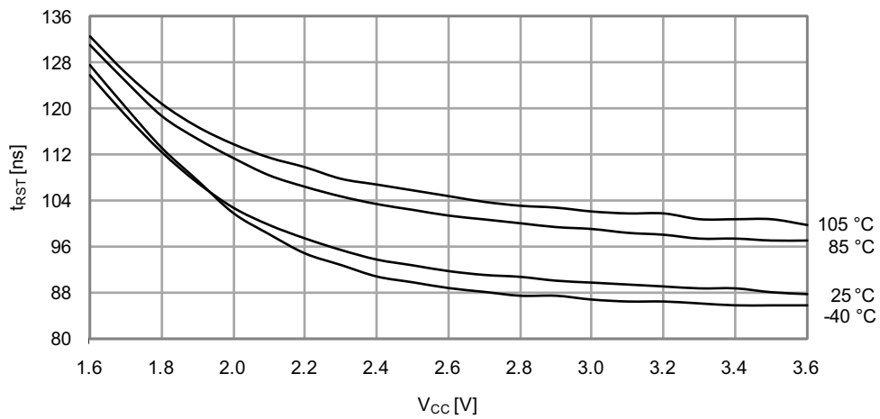
Figure 36-48. Minimum Reset Pin Pulse Width vs. V CC
