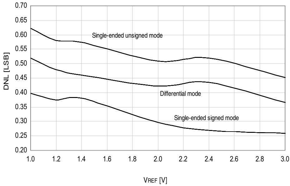
Figure 36-33.DNL Error vs. External V_{REF} T = 25^{\circ}\text{C} , V_{CC} = 3.6\text{V} , external reference
