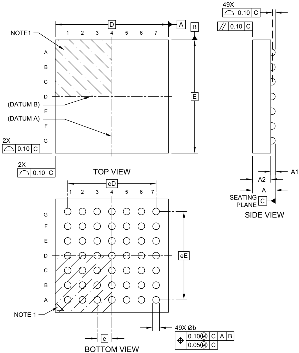
Microchip Technology Drawing C04-21168-C7B Rev A Sheet 1 of 2
