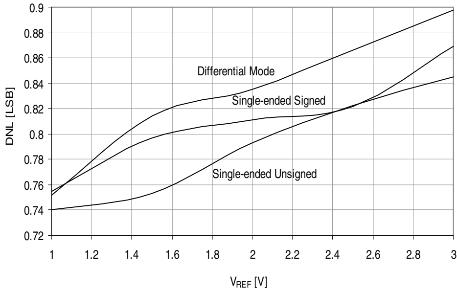
Figure 37-123. DNL error vs. external V_{REF}
