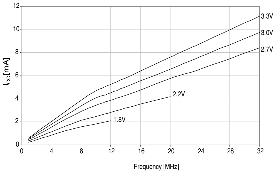
Figure 37-2. Active supply current vs. frequency.
