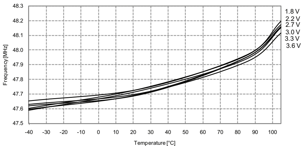
Figure 37-332. 48MHz internal oscillator frequency vs. temperature DPLL enabled, from the 32.768kHz internal oscillator
