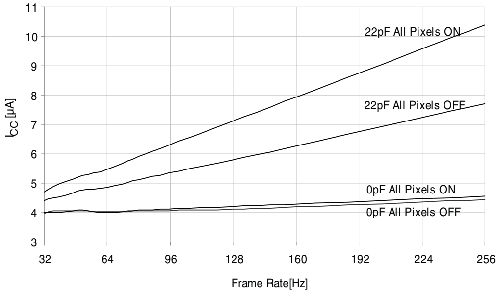
Figure 37-77. I_{CC} vs. Frame Rate
