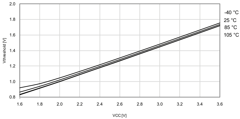
Figure 33-169. I/O Pin Input Threshold Voltage vs. V_{CC}
