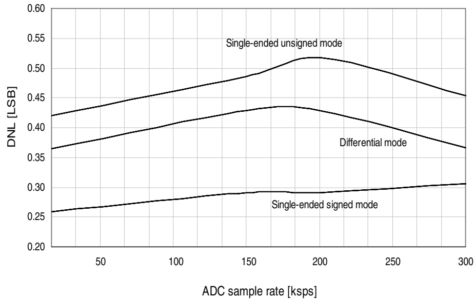
Figure 33-386. DNL Error vs. Sample Rate T = 25°C, V_{CC} = 3.6V , V_{REF} = 3.0V external
