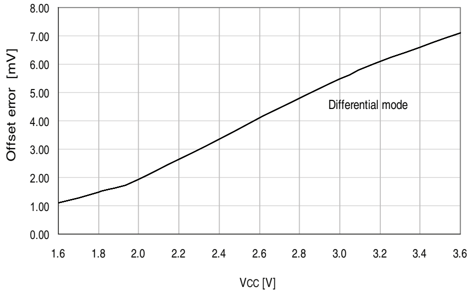
Figure 33-112. Offset Error vs. V_{CC}
