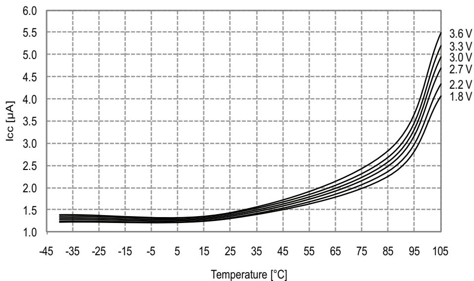
Figure 33-89. Power-down Mode Supply Current vs. Temperature Watchdog and sampled BOD enabled and running from internal ULP oscillator
