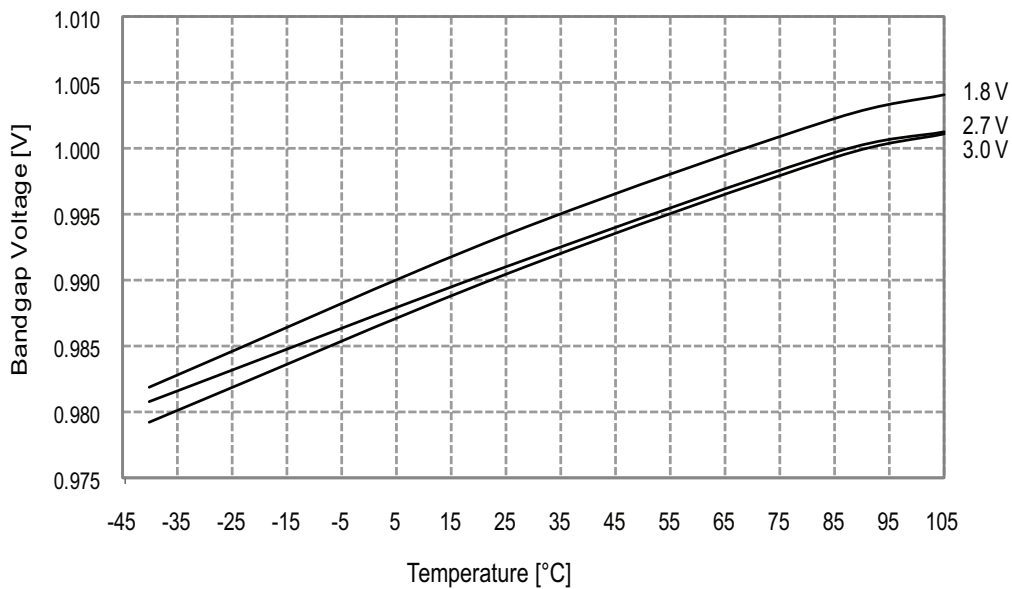
Figure 33-117. ADC Internal 1.0V Reference vs. Temperature
