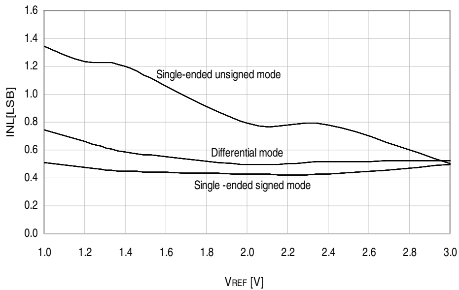
Figure 33-382. INL Error vs. External V_{REF} T = 25^\circ\text{C} , V_{CC} = 3.6\text{V} , external reference
